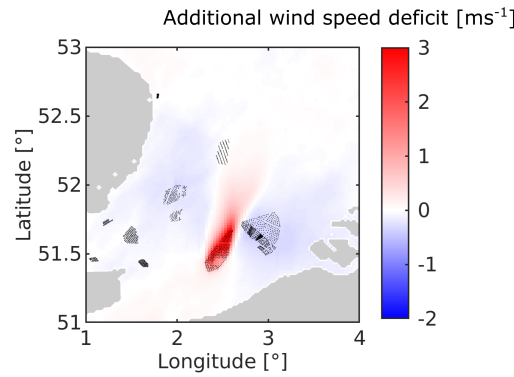
Figure 8. This map shows the additional wind speed deficit, for wind directions between 180^\circ and 210^\circ after the construction of the PE wind farm for timesteps with negative external wake energy losses over the farm.
