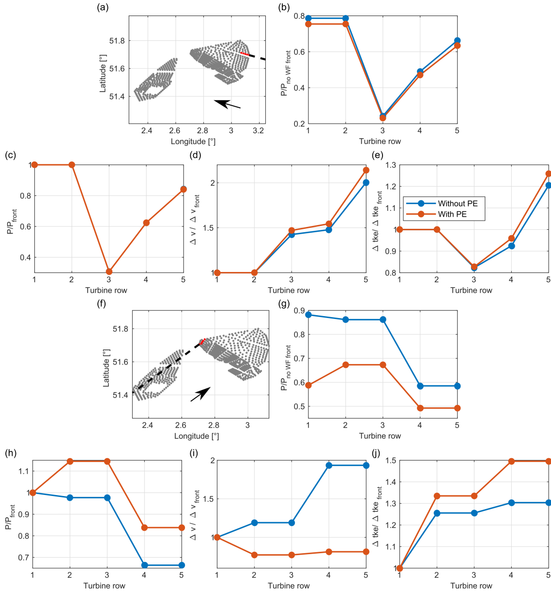
Figure 12. (a,f) Wind turbine locations considered for two representative wind directions (black arrows): (a) 105°, corresponding to a case where the BE–NL wind farm cluster is not influenced by wakes from the PE wind farm cluster, and (f) 234°, corresponding to a case where the BE–NL cluster is waked by the PE wind farm cluster. The red dots indicate the turbine used for the analysis. Panels (b–e) and (g–j) show turbine quantities as a function of turbine row number, illustrating how wake interactions evolve through the wind farm under unwaked and waked conditions (blue and orange, respectively). Specifically, (b,g) show turbine power normalized by the no WF front-row turbine power, (c,h) show turbine power normalized by the front-row turbine power, (d,i) show wind speed deficits relative to the no WF simulation and normalized by the front row, and (e,j) show added TKE relative to the no WF simulation and normalized by the front row.
