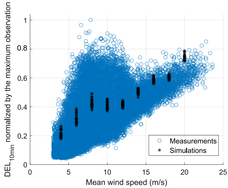
Figure A2. The cluster of 10-minute DEL data in the freestream versus the DEL estimations from simulations in each mean wind speed
