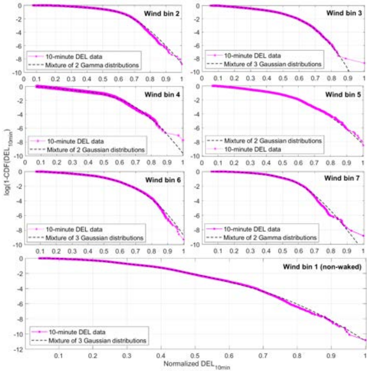
Figure A5. Logarithm of the probability of exceedance of the normalized DEL_{10min} in different wind direction bins in the location of the wind turbine (purple dotted line) and the best distribution fits (black dashed-line)
