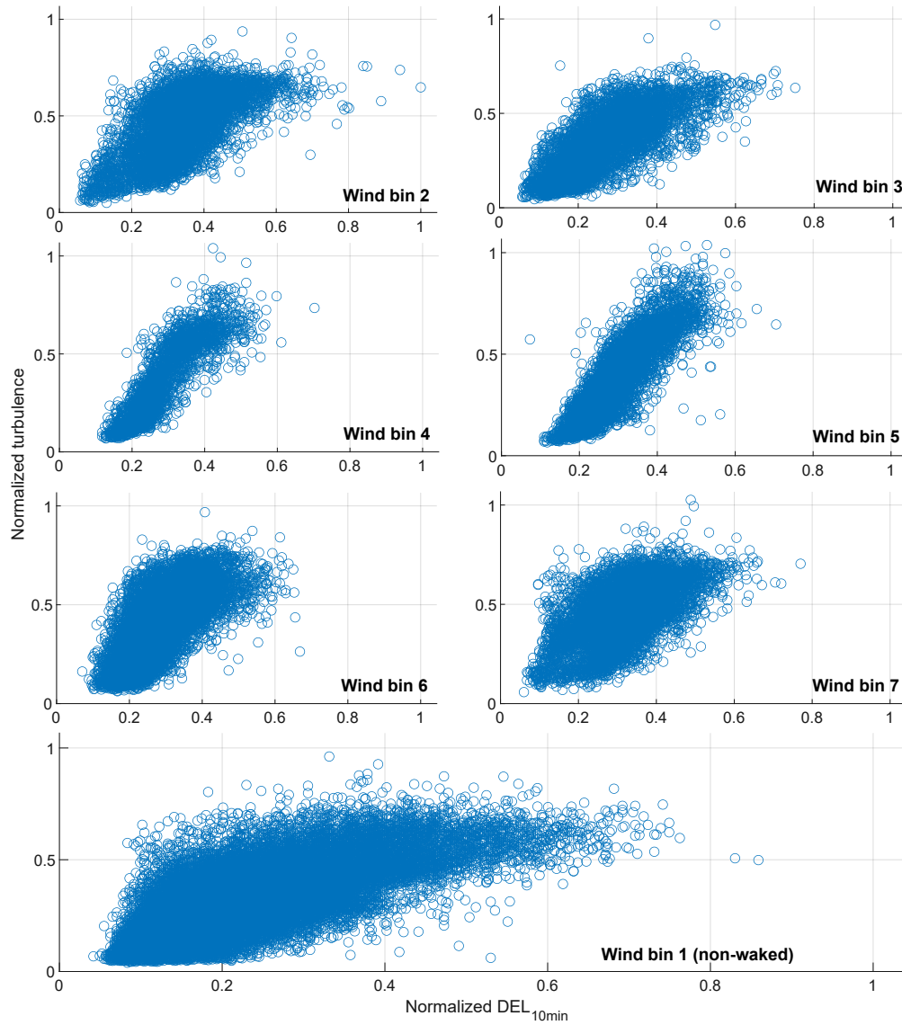
Figure A4. Scatter plot of turbulence data normalized by the highest observations versus corresponding 10-minute DEL observations at the same time in different wind direction bins before filtration
