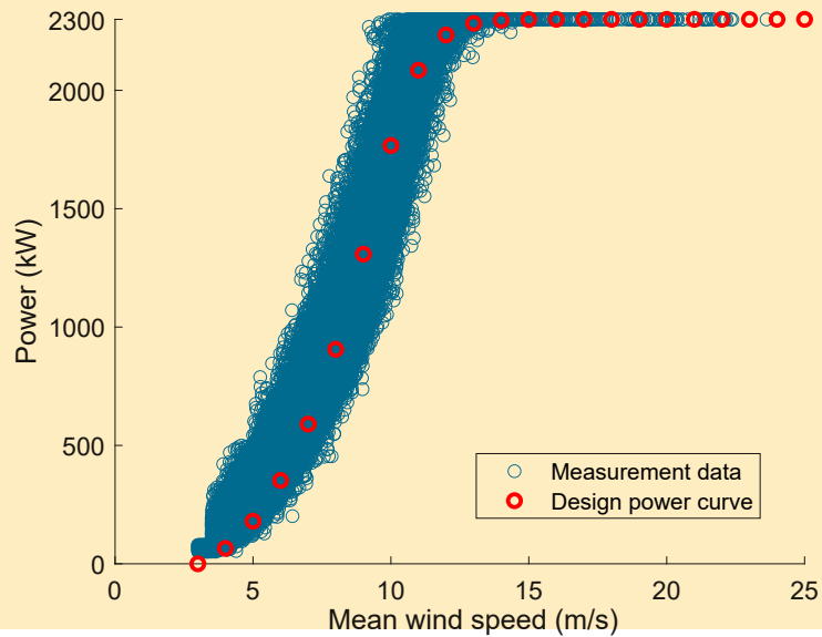
Figure A3. The filtered power production data versus mean wind speed, measured by met-mast mounted anemometer, (blue) compared with the nominal power curve (red)
