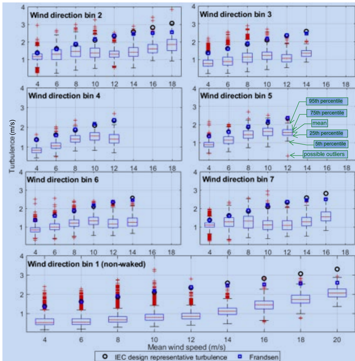
Figure 3. The enhanced turbulence (m/s) based on Frandsen estimation (blue squares) compared with IEC design representative turbulence (black circles) and the site turbulence measurements (box plots)
