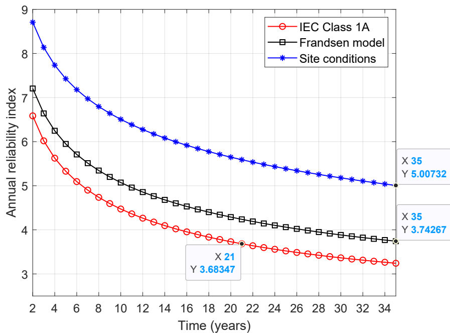
Figure 7. Annual reliability of the case study wind turbine in two scenarios of using Frandsen model (black square) and site load measurements with (blue) versus the IEC design class (red circle)
