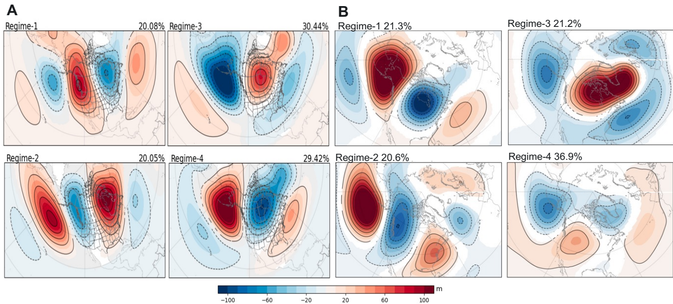
Figure R1 Weather Regime (500 mb geopotential height anomaly) based in Liu et al., 2023. (A) results using 4-node SOM and (B) results using the two-stage (SOM+K-means) method. The percentage numbers indicate the occurrence of each weather regime.
