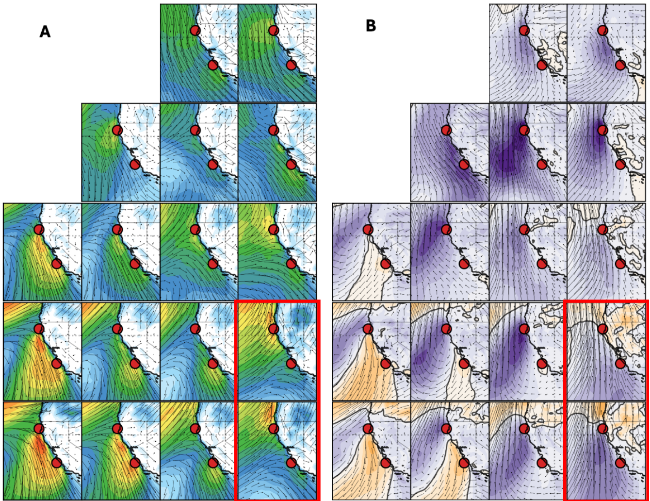
120 Figure R4 Wind speed and direction of SOMs associated with post-ridge LSMP. (A) Mean wind speed and direction and (B) anomalous wind speed and direction. The red boxes outline the two SOMs with strong winds.
