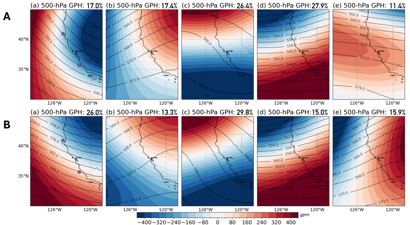
70 Figure R3 Comparison of the LSMPs identified using (A) two-step SOM/K-means approach and (B) SOM clustering.
