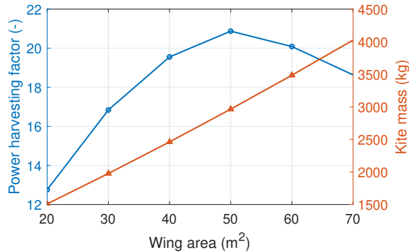
Figure 31. Effect of wing area on the performance of a system with fixed tether diameter of 2.7 cm at a wind speed of 12 ms -1 .
