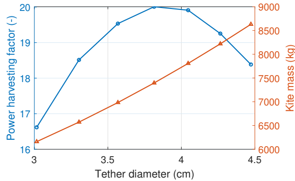
Figure 30. Effect of tether diameter on the performance of an AWE system with a fixed kite wing area of 100 m 2 at a constant wind speed of 12 ms -1 .
