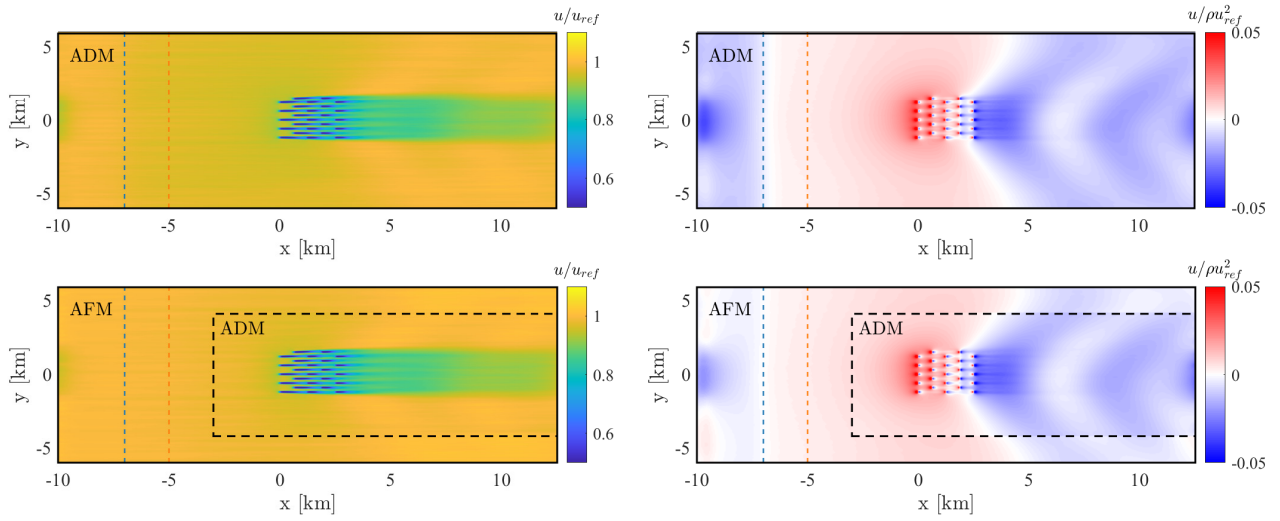
Figure 21. Time-averaged hub height velocity (left) and pressure perturbation (right), calculated as p_p(x, y, z) = p(x, y, z) - p(x_\infty, y, z) , where x_\infty = -7 km and p(x, y, z) is the time-averaged pressure. Top and bottom panels correspond to the ADM and AFM cases, respectively. In the latter, the horizontal inner domain size is identified by the black dashed line. The end of the fringe and advection damping regions are identified by the dashed blue and orange lines, respectively.
