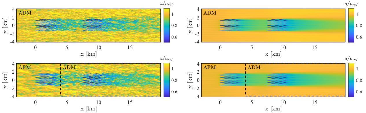
Figure 15. Instantaneous (left) and time-averaged (right) hub height wind speed obtained from cases 1 (top) and 3 (bottom) of Table 3. The dashed black line shows the horizontal size of the inner domain in the AFM simulation.
