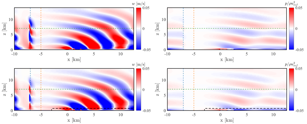
Figure 22. Time-averaged vertical velocity (left) and pressure perturbation (right) at y = 0 . Top and bottom panels correspond to the ADM and AFM cases, respectively. In the latter, the horizontal inner domain size is identified by the black dashed line. The end of the fringe and advection damping regions are identified by the dashed blue and orange lines, respectively, while the start of the Rayleigh damping region corresponds to the green dashed line.
