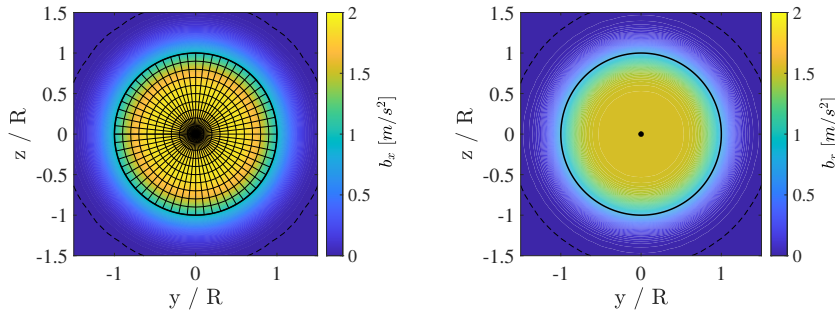
Figure 1. Comparison of two sections located at x = 0 of the body force projection function for the ADM (left) and AFM (right). In the ADM, the force associated to each actuator point is equal to the total wind turbine force scaled by the ratio between the actuator element area and the rotor swept area. For the AFM, the force is projected from a single actuator point, located at the rotor center. The black continuous circle indicates the radial coordinate corresponding to the wind turbine radius. The parameter \sigma is set to 20 m for both Eq. 3 and Eq. 10, while r_{1/2} and s are set to 60 m and 6, respectively.
