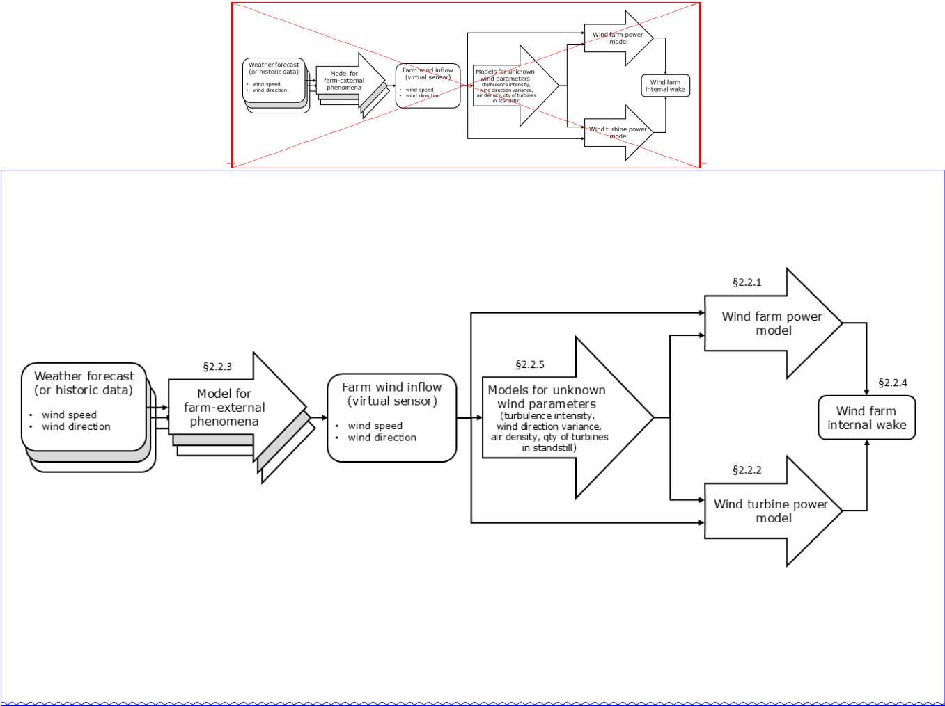
Figure 4. Overview of the modular structure of the multi-component pipeline with multiple ML models
