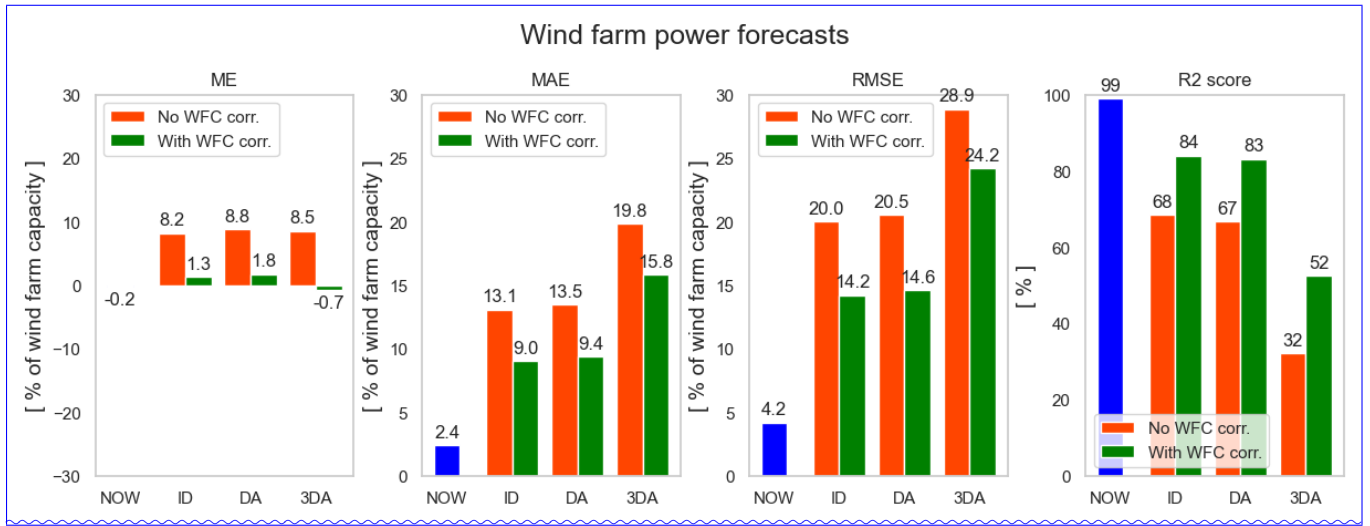
Figure 36. Error metrics for intra-day (ID), day-ahead (DA) and three-days-ahead (3DA) wind farm power forecasts for Wind Farm 1. The orange bars are the metrics for the wind farm power forecasts based directly on the wind speed and direction forecasts of a commercial weather forecast provider. The green bars are the metrics for the wind farm power forecasts based on the corrected wind speed and direction forecasts. The blue bars show the corresponding error metrics for the wind farm model predictions based on actual (NOW) wind inflow measurements.
