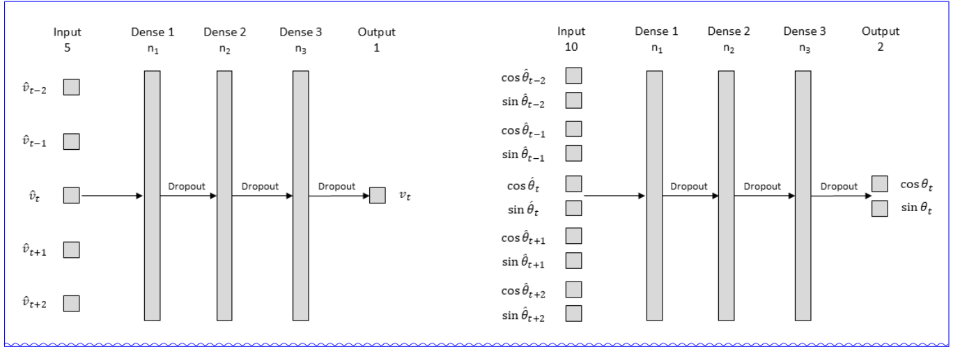
Figure 3. Structure of the deep learning models used to map wind speed forecasts to measured inflow wind speeds (left) and wind direction forecasts to measured inflow wind directions (right).
