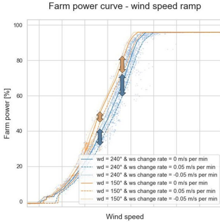
Figure 24. Predicted farm power in function of inflow wind speed ( ws ) with a linearly increasing and decreasing speed with a change rate of 0.05 m/s per minute, for wind directions ( wd ) 240° and 150° (Wind Farm 1).
