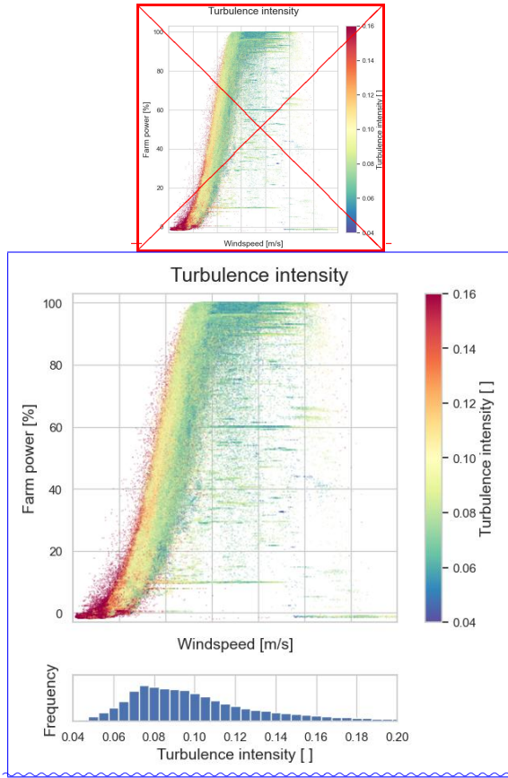
Figure 8. Farm power as a function of inflow wind speed and wind turbulence intensity, and frequency distribution of turbulence intensity (Wind Farm 2)
