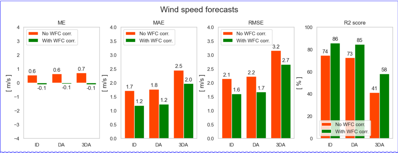
Figure 34. Error metrics for intra-day (ID), day-ahead (DA) and three-days-ahead (3DA) wind speed forecasts for Wind Farm 1. The orange bars are the metrics for the wind speed forecasts of a commercial weather forecast provider. The green bars are the metrics after application of the weather forecast correction (WFC) model.
