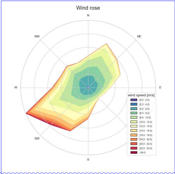
Figure 6. Wind rose for Wind Farm 1
