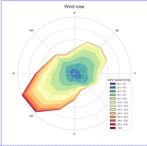
Figure 7. Wind rose for Wind Farm 2
