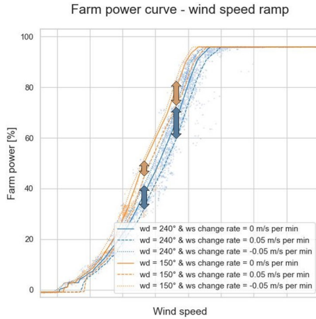
Figure 24. Predicted farm power in function of inflow wind speed (ws) with a linearly increasing and decreasing speed with a change rate of 0.05 m/s per minute, for wind directions (wd) 240^\circ and 150^\circ (Wind Farm 1).
