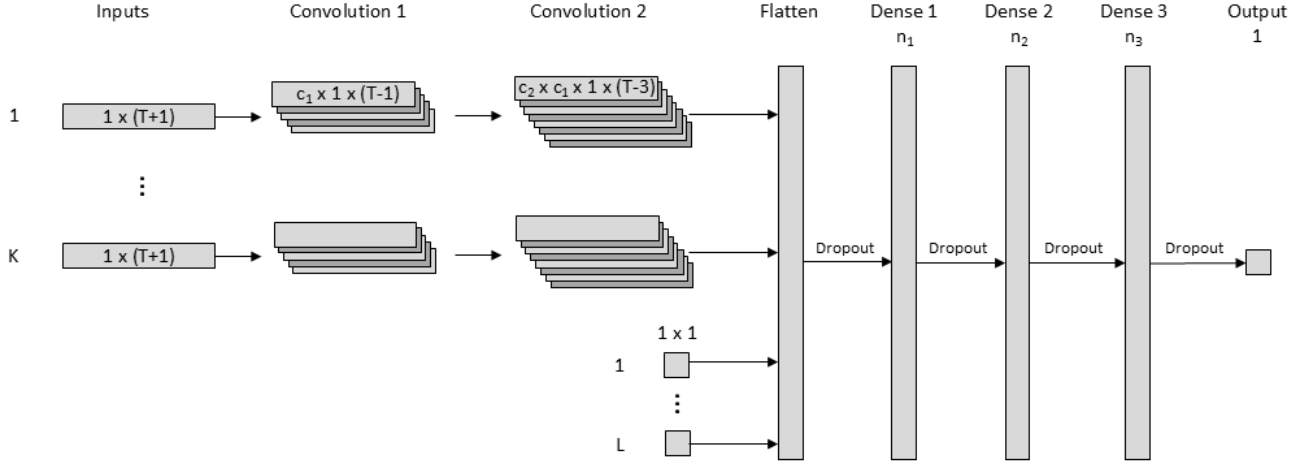
Figure 2. Structure of the proposed deep learning farm power model. K separate convolution branches consist of two 1D convolutional layers. The outputs of these K branches are passed, together with L additional input features, through a flattening and dropout layer, to a three-layer regression model that is composed of three dense layers, each followed by a dropout layer.
