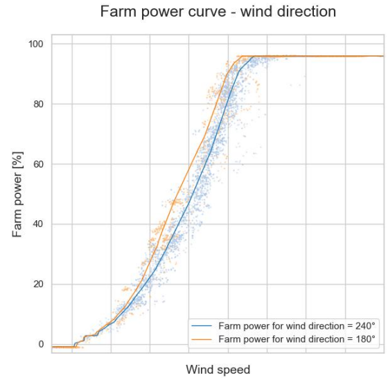
Figure 21. Predicted farm power in function of inflow wind speed and wind direction (Wind Farm 1)
