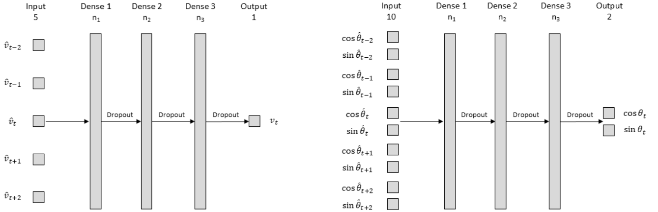
Figure 3. Structure of the deep learning models used to map wind speed forecasts to measured inflow wind speeds (left) and wind direction forecasts to measured inflow wind directions (right).
