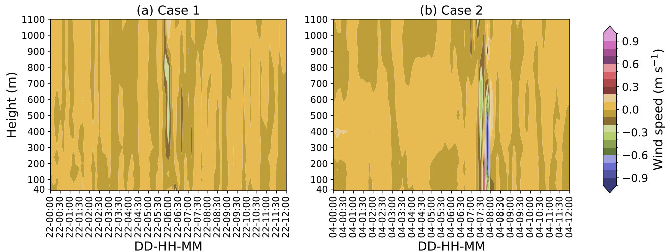
Figure C2. Time-height cross-section of wind speed difference between the CERRA-1d1kmMYFP simulations with 6hr and 12hr spin-up, at the LOT2 location for cases 1 and 2.
