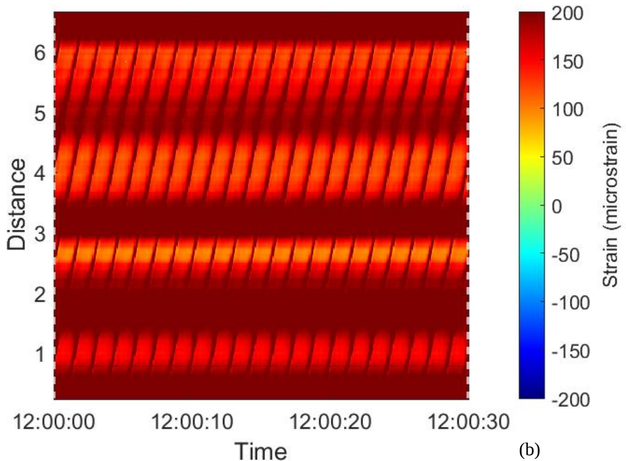
170 Figure 3 Waterfall representation of the strain profile over time for the circumference of the ring rear. The vertical axis denotes 175 distance in meters, while the color gradient indicates strain in micro-strain. (a) Strain profile throughout the entire test period. (b) A magnified view of the strain profile corresponding to the region outlined by the white dashed square in the left panel.
