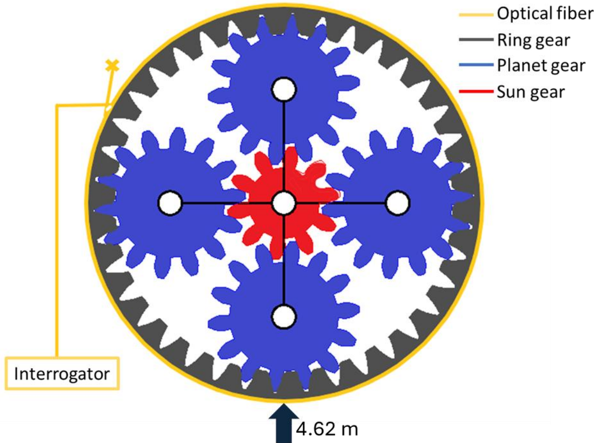
100 Figure 1 The planetary gear stage and the optical fiber attached to the outer surface of the gearbox. The black arrow indicates the location at the bottom of the gearbox used for strain profile demonstration. The point at 4.62 m refers to the distance from the starting point of the optical fiber attachment on the gearbox.
