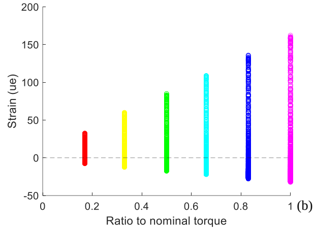
Figure 7 (a) The strain profile in polar axis when different loads are applied to the gearbox and (b) the scatter plot show the clusters of all the collected strain at one location on the ring gears during the load test with different load input.
