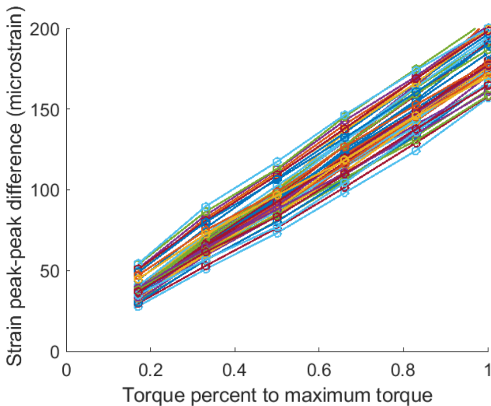
Figure 8 (a) An example of collected strain at 5 locations with time and (b) the peak-peak strain at 49 locations on the ring gear for 6 torque load inputs.
