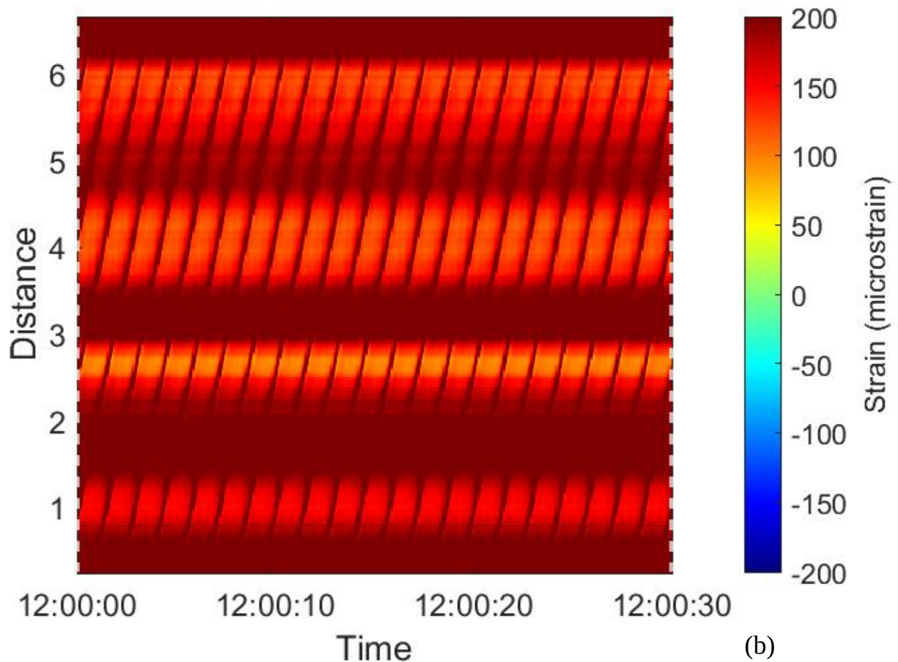
Figure 3 Waterfall representation of the strain profile over time for the circumference of the ring rear. The vertical axis denotes distance in meters, while the color gradient indicates strain in micro-strain. (a) Strain profile throughout the entire test period. (b) A magnified view of the strain profile corresponding to the region outlined by the white dashed square in the left panel.
