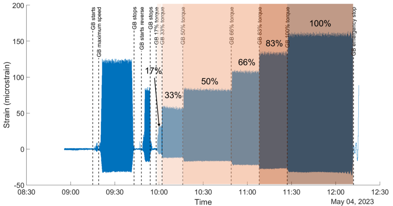
205 Figure 6 The strain response after 0.01 Hz high pass at location 4.62m (one tooth's strain response). The dash line shows the timing of each loading event listed in table 2. The color background shows the percentage of the rated torque input from 17% to 100%, GB represents gearbox.
