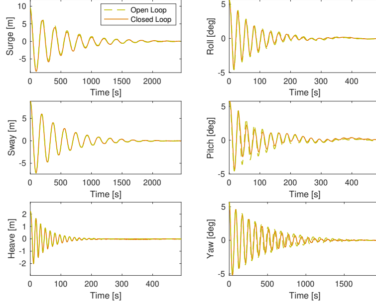
Figure 6. Time histories of floater DOFs for decay tests with the HIL setup in Open-Loop and Closed-Loop configuration. The results are upscaled.
