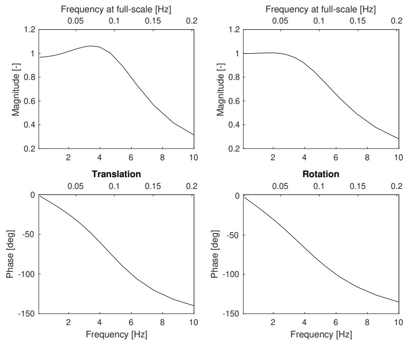
Figure A2. Bode diagram of motion tracking.
