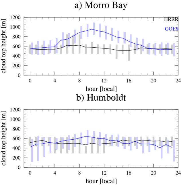
240 Figure 2 Warm season (May-Sept) diurnal cycle of cloud top height as reported by HRRR (gray) and GOES (blue) at (a) Morro Bay and (b) Humboldt Bay. Bounding boxes represent 25 th and 75 th percentile, while the lines represent the mean values.
