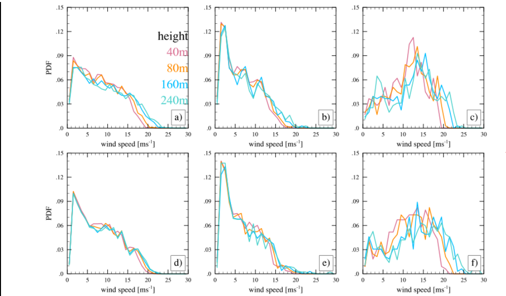
Figure 3 PDF of rotor layer ( \leq 240\text{m} ) wind speed at Morro Bay from (top) HRRR, (bottom) lidar buoy during (left) all conditions, (middle column) cloudy conditions, and (right column) clear sky conditions.
