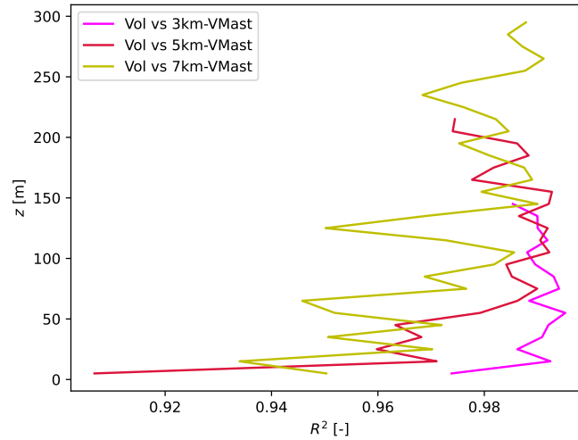
Figure C3. Pearson correlation coefficient between the volumetric and VMast profiles over height.
