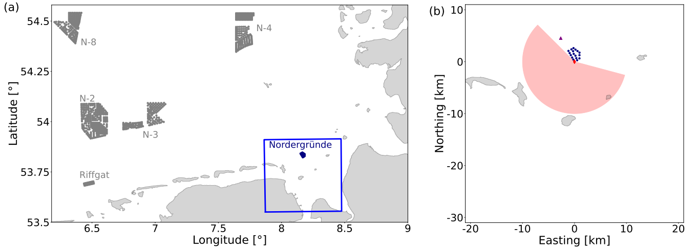
Figure 1. (a) Overview of the German North Sea with operational German offshore wind farms, as of the time of the end of our study (October 2022), depicted in grey. The wind farm Nordergründe where the measurements were conducted, is marked in blue. (b) Layout of NG, also including the nearby coastline (blue square in (a)). The unobstructed lidar scan sector is marked in red. Further, the position of the lighthouse Alte Weser is depicted (purple ▲).
