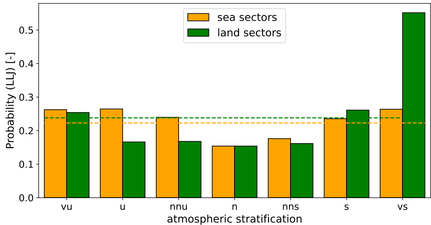
Figure 8. LLJ occurrence frequency across different stability regimes from very unstable towards very stable for land (green) and sea (orange) sectors respectively. The occurrence frequency is computed as a subset of the distribution of stratification events shown in Table 6.
