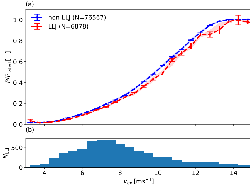
Figure 11. (a) Average apparent power production per binned v_{\text{eq}} (cf. Eq. 11) during non-LLJ situations (blue) and LLJ situations (red). Error bars depict the standard error of the mean of the apparent power within each wind speed bin. Shaded areas depict the corresponding uncertainty intervals obtained by computing power curves with added and subtracted uncertainty estimations respectively (cf. Section 2.4). (b) Number of LLJs per wind speed bin.
