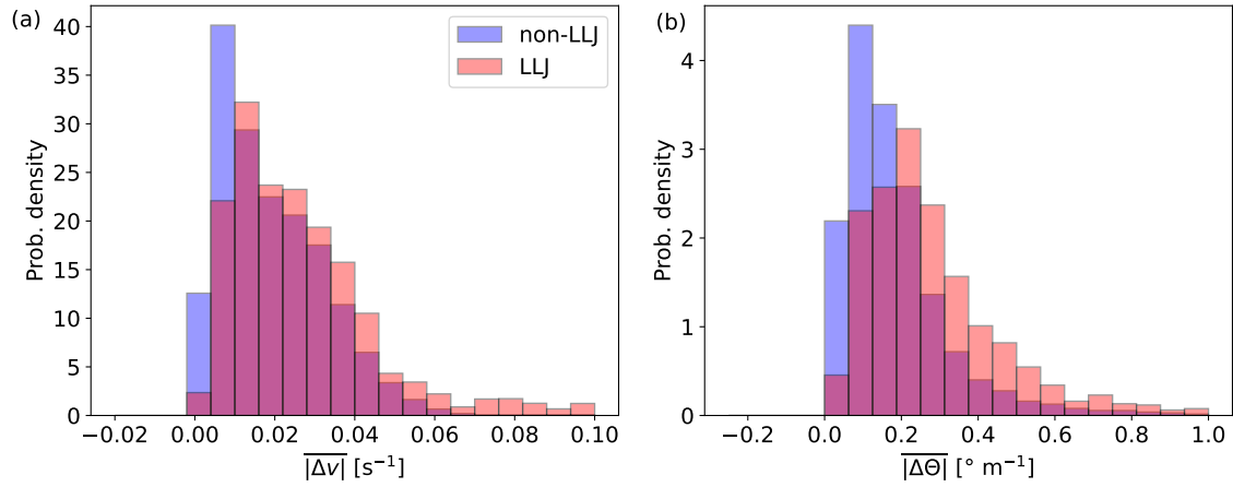
Figure 10. (a) Average wind shear and (b) veer across the rotor swept area for all measured profiles not containing LLJs shaded in blue and those containing LLJs in red.
