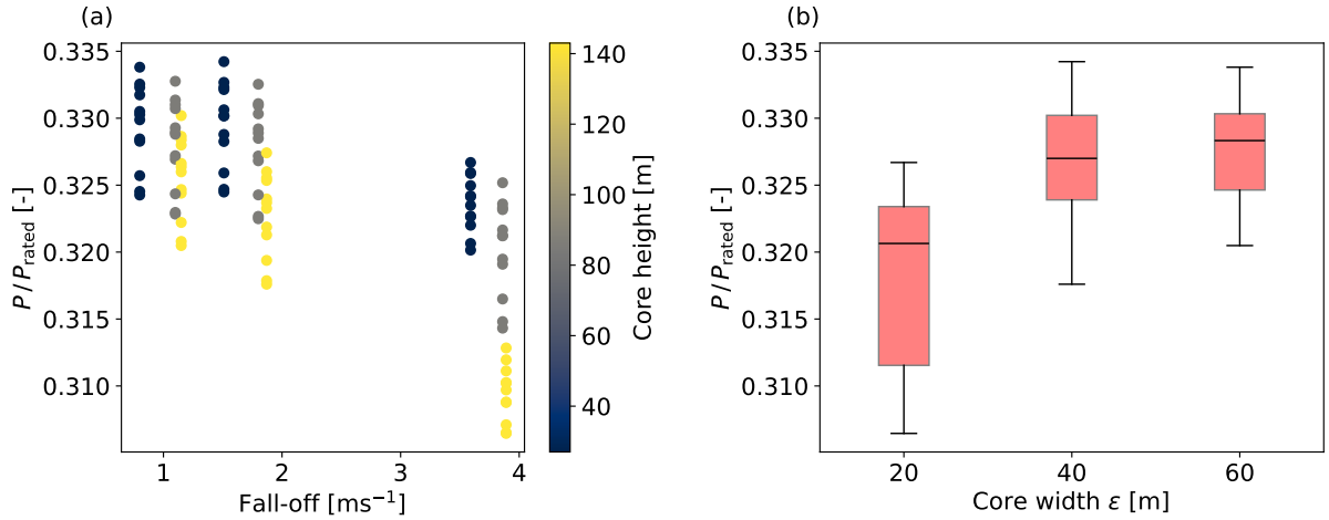
Figure 15. Average power production during simulations with LLJ wind profiles plotted over the fall-off and the core height as colour code (a) and the width of the LLJ core in (b) where the box represents the limits from first and third quartile and the black line the median value.
