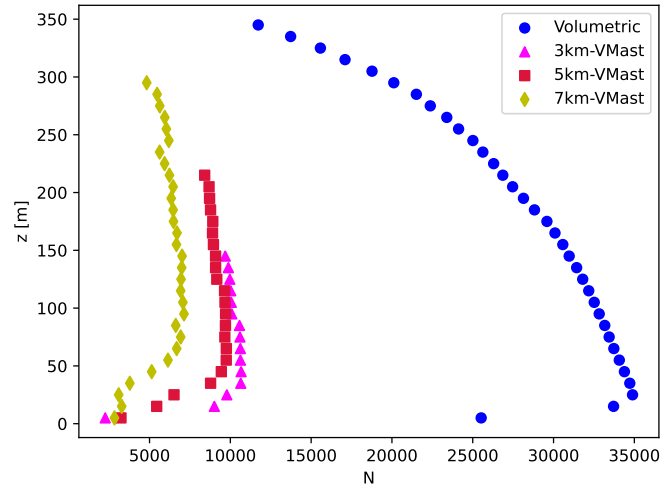
Figure C2. Number of available data points ( N ) throughout the entire measurement campaign at each height for the different profile generation approaches.
