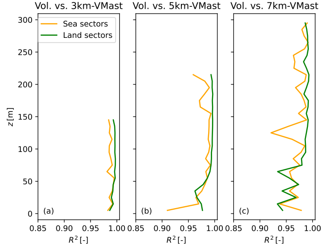
Figure C4. Same as Fig. C3, but separated into land and sea sectors for the VMasts at (a) 3 km, (b) 5 km and (c) 7 km distance to the lidar.
