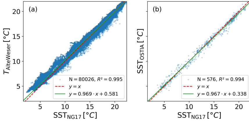
Figure A4. Scatter plots showing the correlation between the SST measurements at NG17 and water temperature measurement at the lighthouse Alte Weser (a) and the OSTIA data set (b), respectively. The y = x curve is depicted as a dashed red line and the regression line in green.
