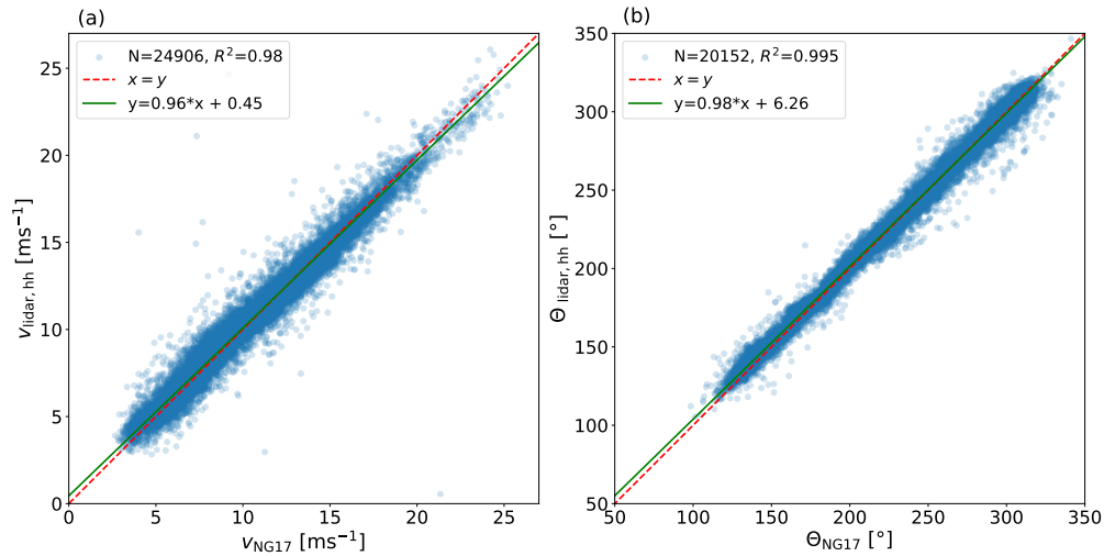
Figure C5. Scatter plot between (a) nacelle wind speed measurements of NG17 lidar derived hub-height wind speed and (b) nacelle measurements of the wind direction and the lidar estimated wind direction at hub height. The dashed red line shows the x = y and the regression line is drawn in green.
