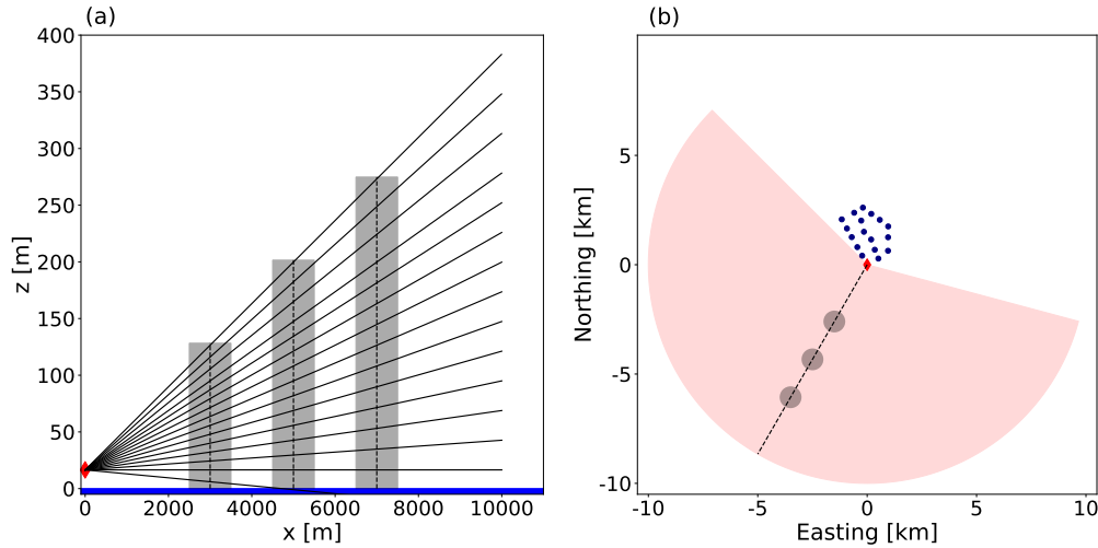
Figure C1. Scanning characteristics of the measurement campaign. (a) Different elevations across the entire range of the scans (black). Relative locations of the VMasts in the scan (dashed lines) and the area of included measurement points for each VMast (grey shaded). The x-axis is oriented along the dashed line in (b). (b) Top view on the measurement sector, with the entire measurement range of the lidar (red) and the sub-areas considered for the VMast approach (grey).
