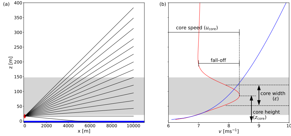
Figure 2. (a) Exemplary scanning pattern for the lidar measurement campaign, with the position of the lidar displayed at the height of the transition piece (red \blacklozenge ), the lidar beams as black lines and the height range of the rotor swept area marked as a gray background. (b) Exemplary LLJ profile in red, with the important terminology defined. For reference, a logarithmic wind profile with the same REWS of 8 \text{ ms}^{-1} is shown in blue.
