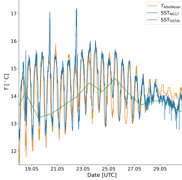
Figure A2. Water temperature at the lighthouse Alte Weser T_{AlteWeser} with a resolution of 1/60 Hz (WSV, 2023) (orange), sea surface temperature SST_{NG17} measured with an infrared sensor from the transition piece of turbine NG17 in the offshore wind farm Nordergründe resampled to one minute (blue), and sea surface temperature from the OSTIA data set SST_{OSTIA} (Good et al., 2020) at a grid point in the western vicinity of Nordergründe with one value per day (green).
