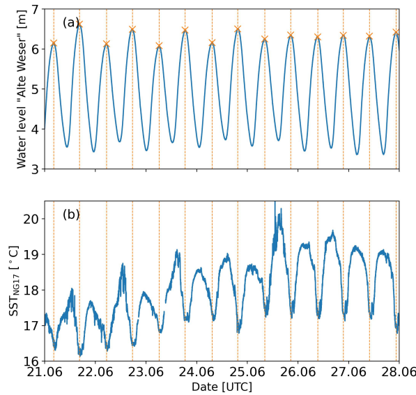
Figure A1. (a) Water level measured at the lighthouse Alte Weser (WSV, 2023). Maxima are detected with a peakfinder and marked (×). (b) Sea surface temperature measured at the wind turbine NG17 in the offshore wind farm Nordergründe with approx. 5.2 km distance to Alte Weser. Times of high tide detected in (a) are marked by vertical dashed lines.
