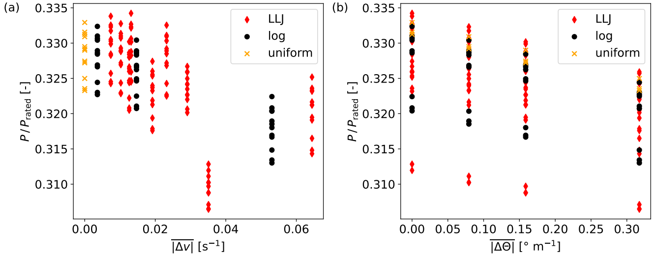
Figure 13. Simulated normalised power production over the shear (a) and veer (b) of the wind profiles across the rotor swept area for each of the simulated inflow profiles. Uniform wind profiles are depicted as orange crosses, logarithmic profiles as black circles and the LLJ profiles as red diamonds.
