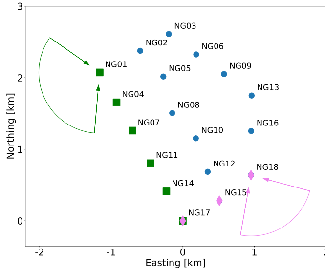
Figure 3. Layout of wind farm NG with turbine names. The turbines selected for further analysis are marked in green and magenta respectively and their corresponding wind direction sectors are specified as arrows with matching colours.
