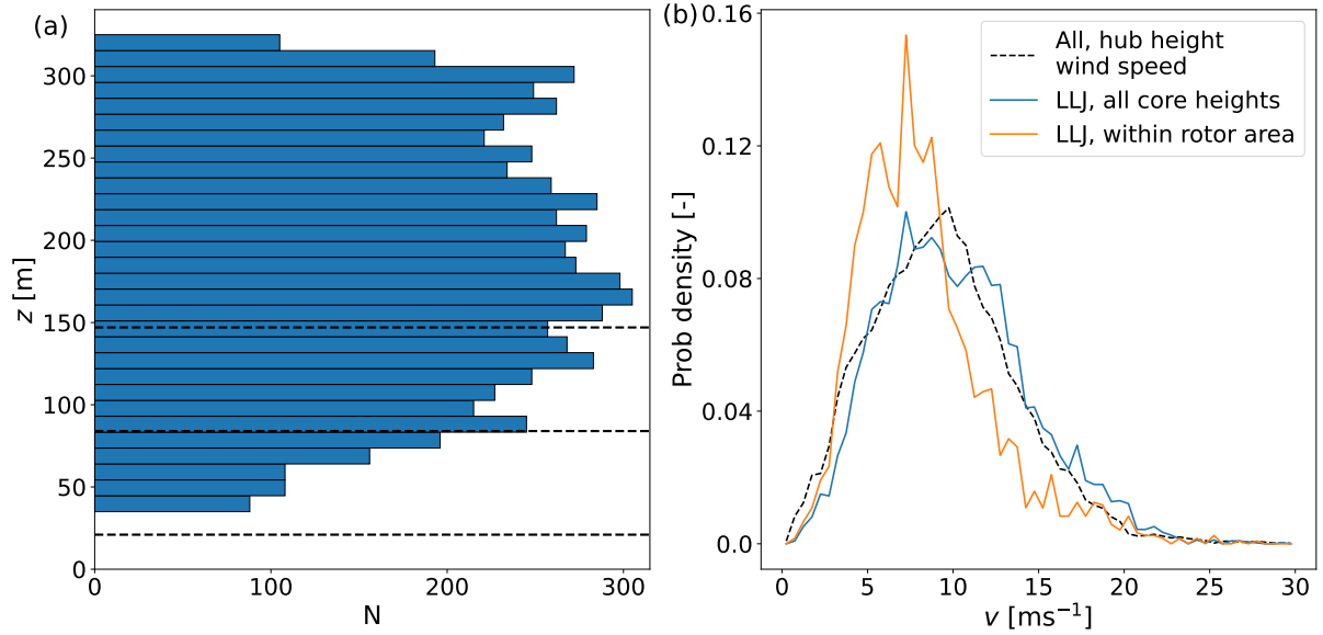
Figure 9. (a) Number ( N ) of measured LLJ cores across all heights. Lower tip, upper tip and hub height are marked by dashed lines. (b) Distributions of core speeds for all observed LLJs (blue), the data subset with core heights within the rotor area (orange) together with the hub height wind speed distribution of the whole data set (black dashed line).
