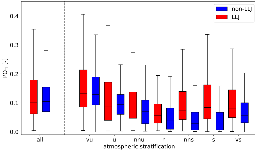
Figure 12. Box plots of the normalised standard deviation of the power production PO_{TI} for LLJ and non-LLJ situations, respectively, across all the different stability regimes. The boxes are limited by the first (Q1) and third quartile (Q3) respectively, with the whiskers representing Q_1 - 1.5 IQR and Q_3 + 1.5 IQR , with IQR the interquartile range. The horizontal black lines represent the median PO_{TI} .
