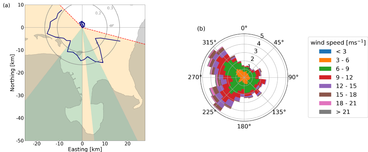
Figure 6. (a) Polar plot of the probability density of LLJ occurrences dependent on the wind direction (blue line) in the analysed wind direction sector (red dashed sector). For reference, the wind farm NG (blue markers) and coastlines (black) are shown. Further, the land and sea sectors are coloured in green and orange respectively. (b) Distribution of wind direction and corresponding wind speeds at hub height at the NG wind farm calculated from the nacelle anemometers of turbine NG17.
