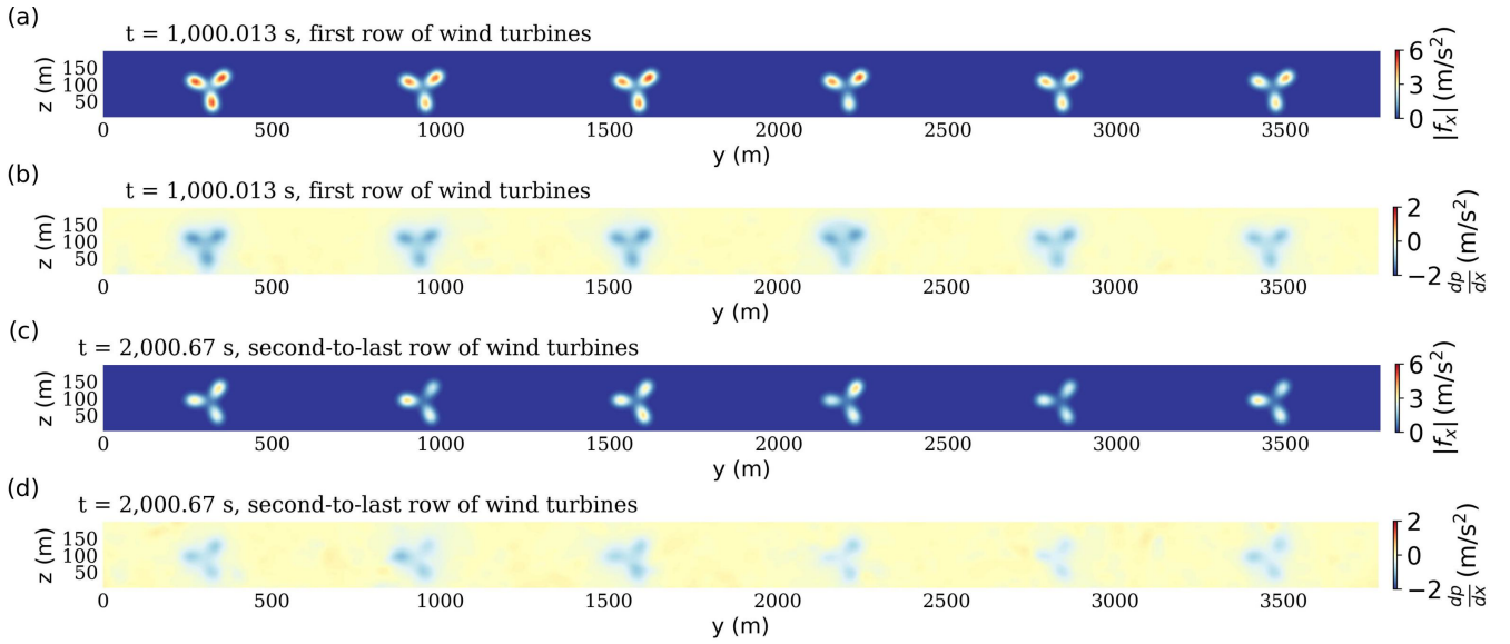
Figure 8. Instantaneous contours of turbine streamwise (i.e., x -component) force (as projected onto the LES grid using Gaussian smoothing as part of the ALM method) in y-z planes at (a) First row (i.e., Row 1, x = 12,348 m) and between the relevant vertical range z \in [2.5, 200] m, and (c) second-to-last row (i.e., Row 9, x = 19,404 m). Panels (b) and (d) show the x -direction pressure gradient distributions on the same planes, coincident with the turbines.
