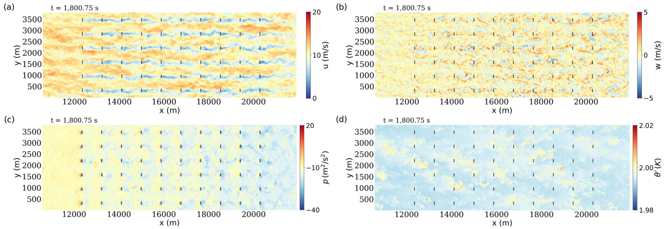
Figure 5. Contour plots of instantaneous flow field variables in part of the wind farm domain (here between x = 10,584 m and x = 21,921.375 m), at time t = 1,800.75 s. (a) the streamwise velocity u , (b) the vertical velocity w , (c) the pressure p , and (d) the potential temperature deviation \theta' . The short black lines represent the location of wind turbines.
