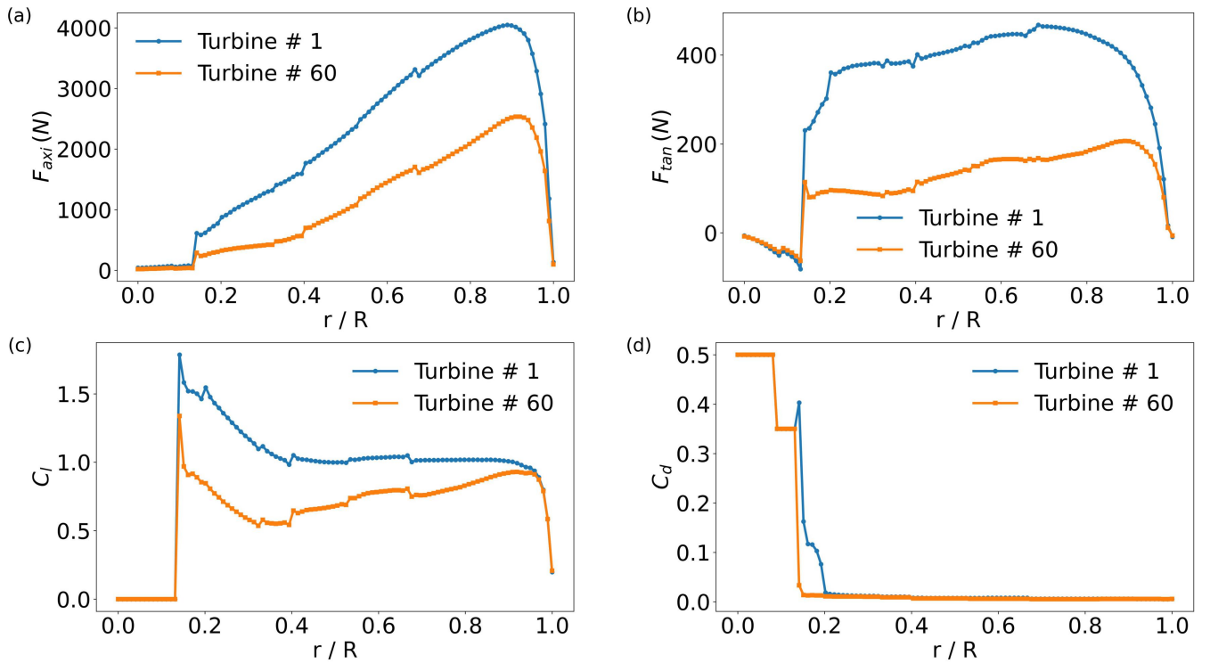
Figure 16. Distributions of ALM quantities along the turbine blade at a specific time ( t = 1,500 s for Blade #1 of Turbine #1, blue lines; and Blade # 1 of Turbine #60, orange lines): (a) Axial component of the local force (on each \Delta\ell = 0.615 m segment) F_{axi} , (b) Tangential component of the local force (on each \Delta\ell = 0.615 m segment) F_{tan} , (c) Lift coefficient C_l , (d) Drag coefficient C_d .
