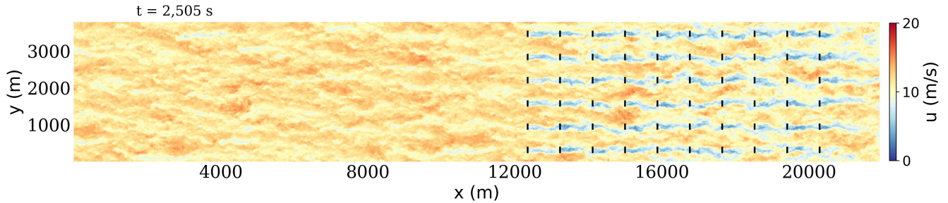
Figure 7. Contour plot of instantaneous streamwise velocity u in the entire database domain, ranging from x = 0 to x = 22,913.625 m, at time t = 2,505 s. It is noted that although the total length of the database domain is 10,584 + 12,348 = 22,932 m, the data resolution in x -direction is 18.375 m and the grid points are located at cell centers. Consequently, the last data point is located at 22,932 - 18.375 = 22,913.625 m. The short black lines represent the location of wind turbines.
