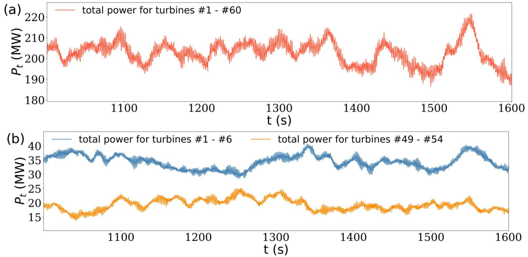
Figure 12. Time evolution of power from turbines during the 10-minute time interval, i.e., t \in [1000.33, 1600.33] s. (a) shows the total power from the entire wind farm, while (b) shows the power for the turbines in Row 1 (i.e., Turbines #1-#6) and in Row 9 (i.e., Turbines #49-#54).
