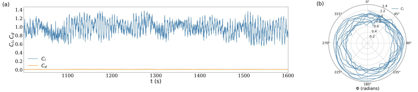
Figure 14. (a) Time evolution of lift and drag coefficients on an ALM point 80% along the span of Blade #3 for Turbine #28. (b) Polar plot of lift coefficient for that point as a function of blade angle along its rotation. For this turbine, the rotational speed is fixed at \Omega = 1.09 rad/s (as obtained from getTurbineData(...) ), corresponding to approximately 10.5 revolutions during a 60-second period.
