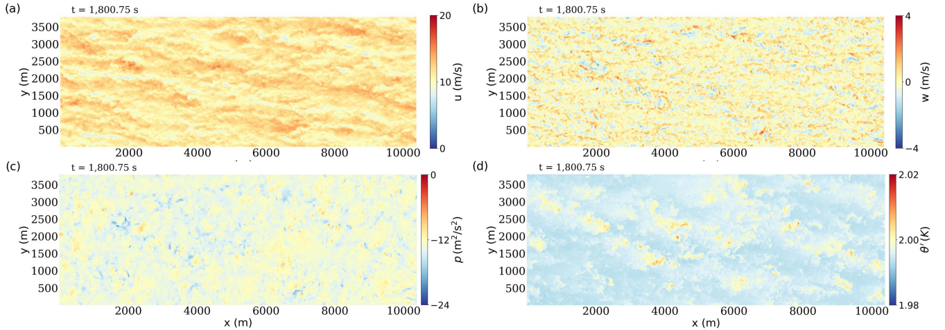
Figure 4. Contour plots of instantaneous flow field variables in part of the precursor domain (here between x = 0\text{m} and x = 10,381.875\text{m} ), at time t = 1,800.75\text{ s} . (a) the streamwise velocity u , (b) the vertical velocity w , (c) the pressure p , and (d) the potential temperature deviation \theta' .
