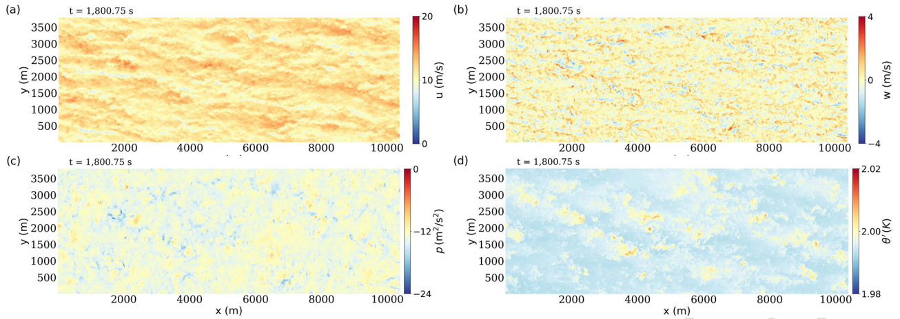
Figure 4. Contour plots of instantaneous flow field variables in part of the precursor domain (here between x = 0 m and x = 10381.875 m), at time t = 1800.75 s. (a) The streamwise velocity u , (b) the vertical velocity w , (c) the pressure p , and (d) the potential temperature deviation \theta' .
