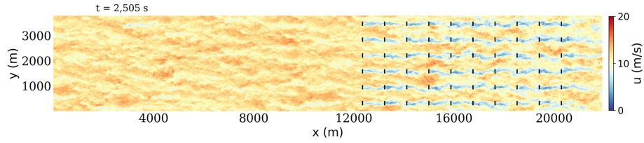
Figure 7. Contour plot of instantaneous streamwise velocity u in the entire database domain, ranging from x = 0 to x = 22913.625 m, at time t = 2505 s. It is noted that, although the total length of the database domain is 10584 + 12348 = 22932 m, the data resolution in the x direction is 18.375 m and the grid points are located at cell centers. Consequently, the last data point is located at 22932 - 18.375 = 22913.625 m. The short black lines represent the location of wind turbines.
