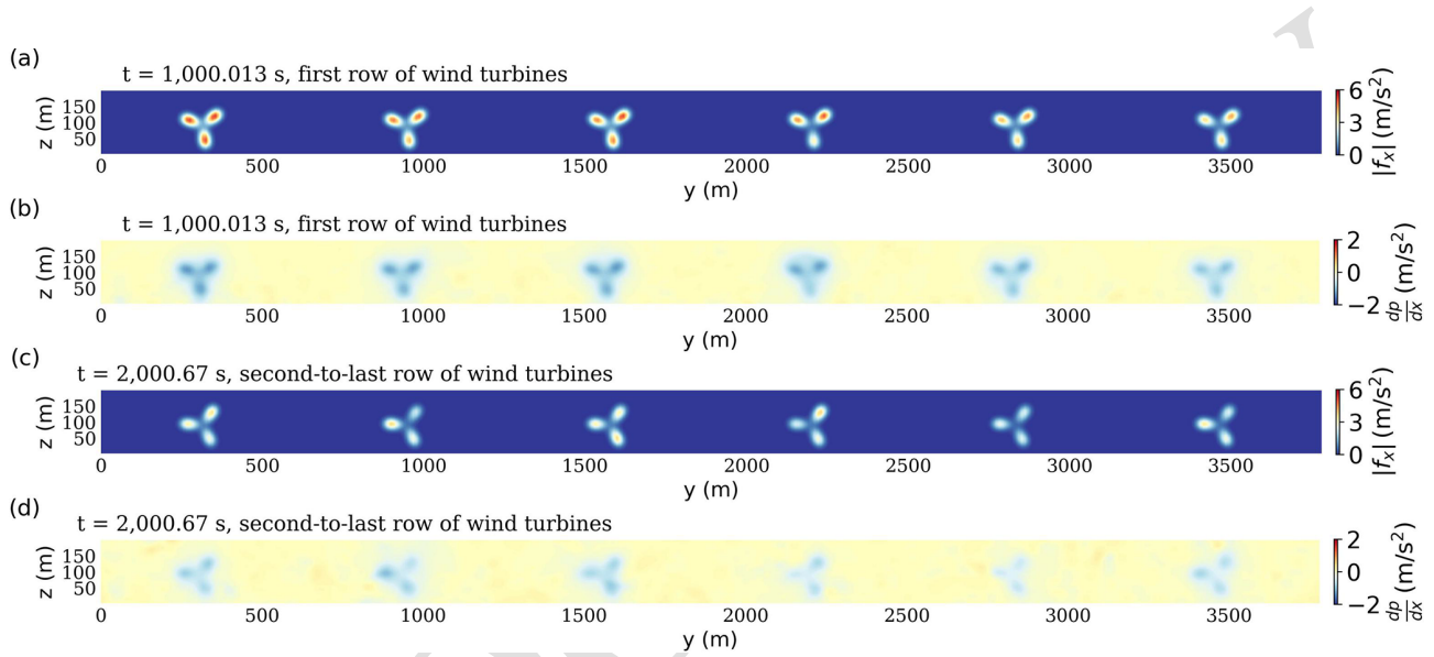
Figure 8. Instantaneous contours of turbine streamwise (i.e., x -component) force (as projected onto the LES grid using Gaussian smoothing as part of the ALM method) in the y - z planes (a) in the first row (i.e., Row 1, x = 12348 m) and between the relevant vertical range z \in [2.5, 200] m and (c) in the second-to-last row (i.e., Row 9, x = 19404 m). Panels (b) and (d) show the x -direction pressure gradient distributions on the same planes, coincident with the turbines.
