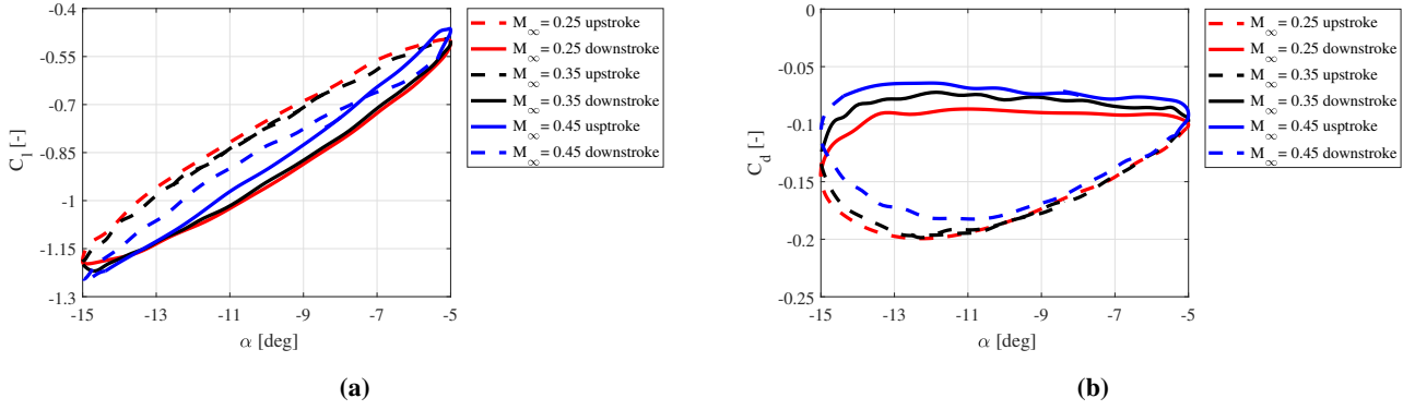
Figure 11. (a) Lift coefficient as a function of the effective angle of attack for M_\infty=0.25 , M_\infty=0.35 , M_\infty=0.45 ; k=0.6 and Re=9 \times 10^6 : downstroke (solid line), upstroke (dashed line). (b) Drag coefficient as a function of the effective angle of attack for M_\infty=0.25 , M_\infty=0.35 , M_\infty=0.45 ; k=0.6 and Re=9 \times 10^6 : downstroke (solid line), upstroke (dashed line).
