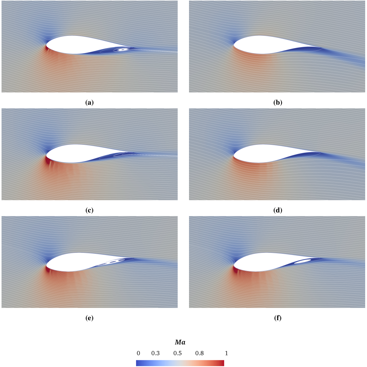
Figure 9. Instantaneous streamlines and contour maps of local Mach number; Re = 9 \times 10^6 , k=0.6 and M_\infty = 0.45 : (a) \alpha = -7.5^\circ downstroke, (b) \alpha = -7.5^\circ upstroke and (c) \alpha = -12^\circ downstroke, (d) \alpha = -12^\circ upstroke, (e) \alpha = -15^\circ downstroke (f) \alpha = -15^\circ upstroke.
