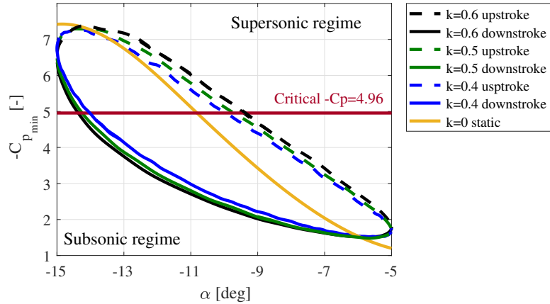
Figure 4. Minimum pressure coefficient as a function of the effective angle of attack, for k = 0.4 (blue lines), k = 0.5 (green lines), k = 0.6 (black lines), k = 0 (yellow line): downstroke (solid lines), upstroke (dashed lines); M_\infty = 0.35 and Re = 9 \times 10^6 .
