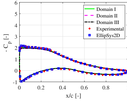
Figure A1. Mean pressure coefficient distribution, for varying domain size, at \alpha = 7.99^\circ and \text{Re} = 1.8 \times 10^6 , compared to reference data (Bertagnolio et al., 2001). This image is taken by (Vitulano et al., 2025).
