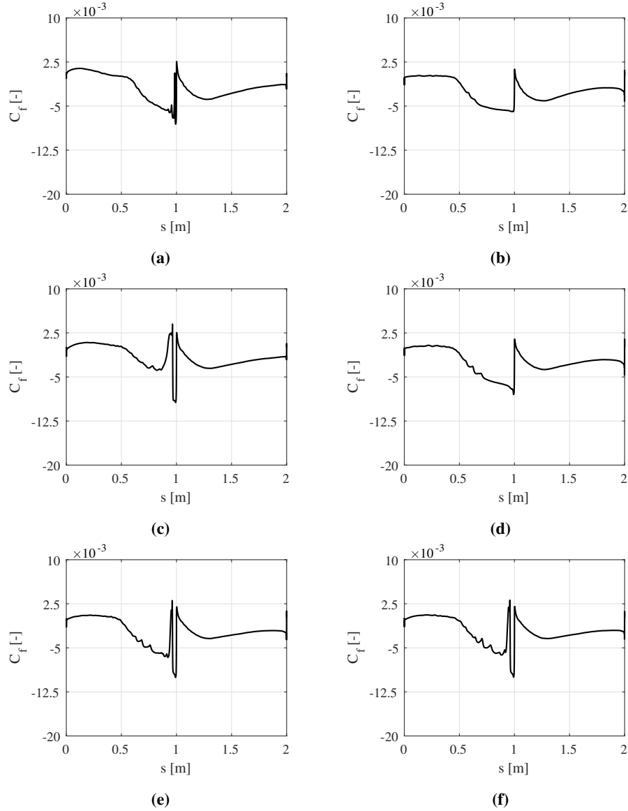
Figure 10. Instantaneous skin friction coefficient distribution; Re = 9 \times 10^6 , k=0.6 and M_\infty = 0.45 : (a) \alpha = -7.5^\circ downstroke, (b) \alpha = -7.5^\circ upstroke and (c) \alpha = -12^\circ downstroke, (d) \alpha = -12^\circ upstroke, (e) \alpha = -15^\circ downstroke (f) \alpha = -15^\circ upstroke.
