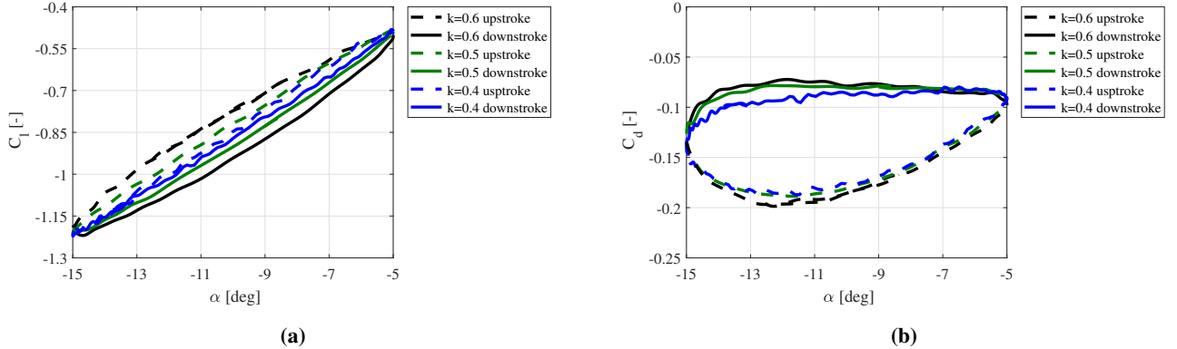
Figure 5. (a) Lift coefficient as a function of the effective angle of attack for k=0.4 (blue line), k=0.5 (green line), and k=0.6 (black line); M_\infty=0.35 and Re=9 \times 10^6 : downstroke (solid line), upstroke (dashed line). (b) Drag coefficient as a function of the effective angle of attack for k=0.4 (blue line), k=0.5 (green line), and k=0.6 (black line); M_\infty=0.35 and Re=9 \times 10^6 : downstroke (solid line), upstroke (dashed line).
