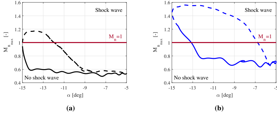
Figure 13. Maximum normal Mach number coefficient as a function of the effective angle of attack: (a) M_\infty=0.35 and (b) M_\infty=0.45 ; k=0.6 and Re=9 \times 10^6 , solid line: downstroke, dashed line: upstroke.
