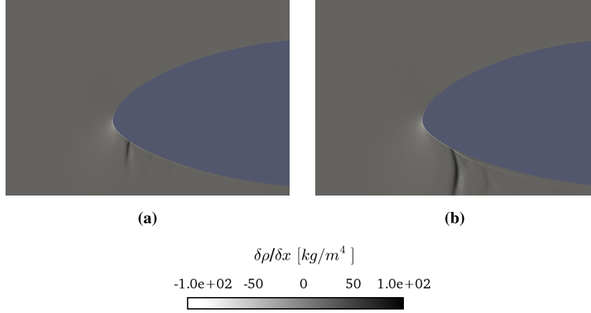
Figure 15. Instantaneous (numerical) Schlieren images: (a) \alpha = -14^\circ downstroke and (b) \alpha = -14^\circ upstroke; M_\infty=0.45 ; k = 0.6 and \text{Re} = 9 \times 10^6 .
