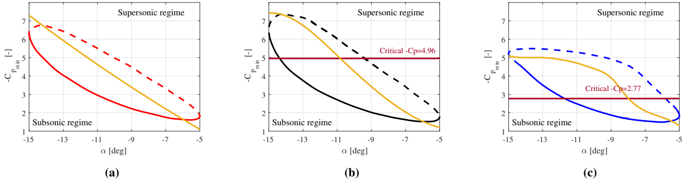
Figure 8. Minimum pressure coefficient as a function of the effective angle of attack for M_\infty = 0.25 (a), 0.35 (b), and 0.45 (c); k=0.6 and Re=9 \times 10^6 : downstroke (solid line), upstroke (dashed line). The yellow line corresponds to the fixed airfoil.
