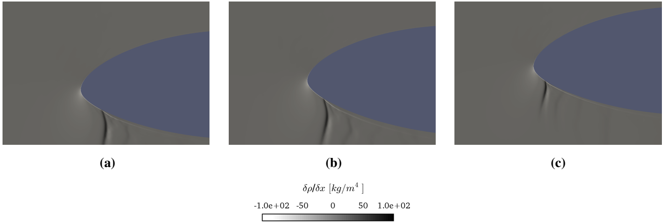
Figure 16. Instantaneous (numerical) Schlieren images: (a) \alpha = -14^\circ , (b) \alpha = -12^\circ and (c) \alpha = -8.5^\circ upstroke; M_\infty=0.45 , k = 0.6 and \text{Re} = 9 \times 10^6 .
