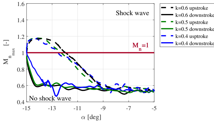
Figure 6. Maximum normal Mach number coefficient as a function of the effective angle of attack for k=0.4 (blue line), k=0.5 (green line), and k=0.6 (black line); M_\infty=0.35 and Re=9 \times 10^6 : downstroke (solid line), upstroke (dashed line).
