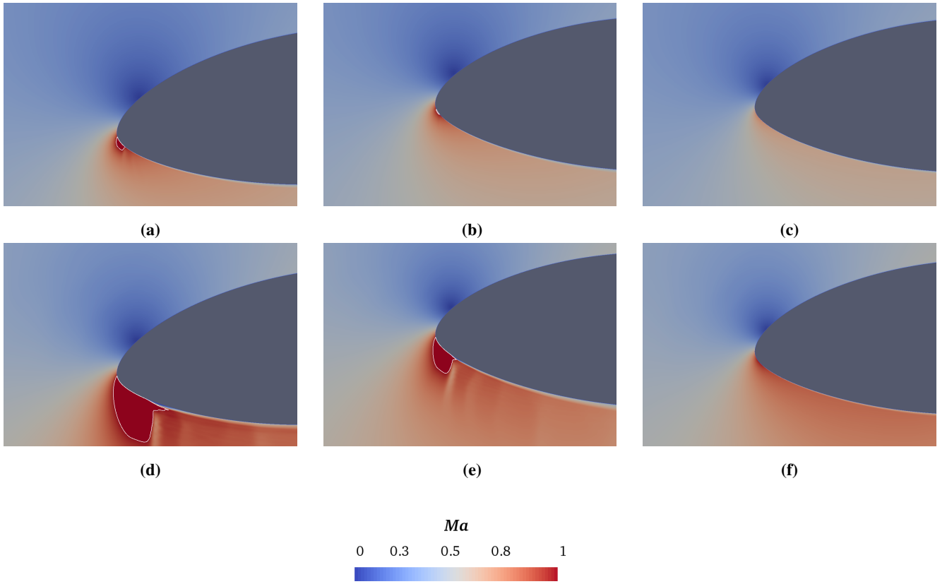
Figure 12. Instantaneous contour maps of local Mach number at Re = 9 \times 10^6 and k=0.6 for varying free-stream velocity: M_\infty = 0.35 at (a) \alpha = -15^\circ , (b) \alpha = -10^\circ upstroke and (c) \alpha = -10^\circ downstroke; M_\infty = 0.45 at (d) \alpha = -15^\circ , (e) \alpha = -10^\circ upstroke and (f) \alpha = -10^\circ downstroke. The iso-line corresponds to Ma=0.99 .
