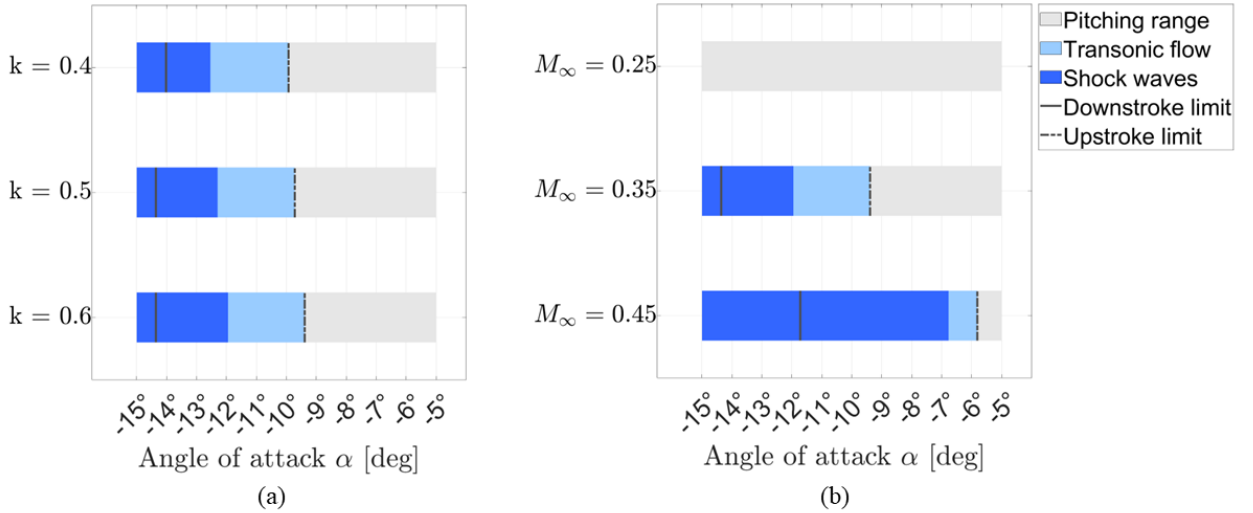
Figure 17. Flow regimes during pitching motion as a function of (a) reduced frequency, (b) inflow Mach number, highlighting the angles of attack of the full pitching period (gray), in which transonic flow occurs (light blue), and shock waves appear (dark blue). The transonic limits of the downstroke (solid line) and upstroke (dashed line) are indicated for reference.
