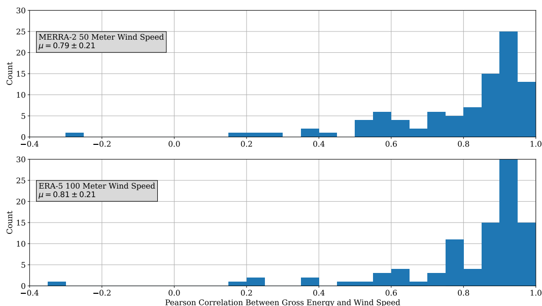
Figure 2. Histogram of the correlation between the monthly gross energy production and each of the monthly MERRA-2 50 m wind speed (top) and ERA-5 100 m wind speed (bottom) for each wind plant for the nearest available coordinate.
