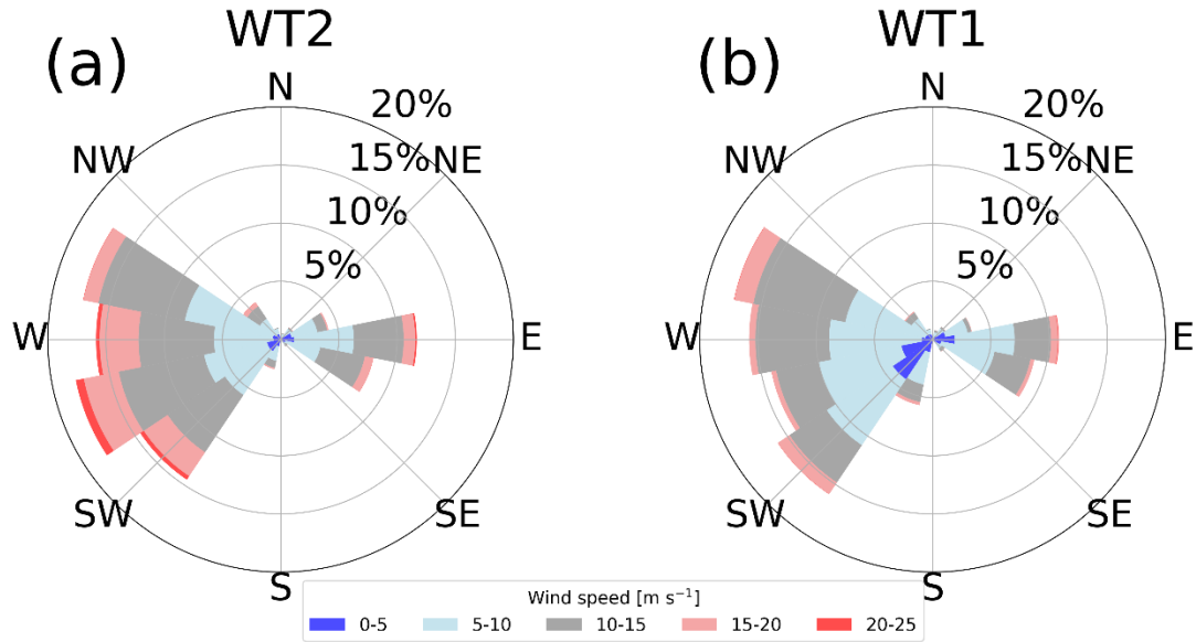
Figure 3. Wind roses derived from the SCADA data of (a) WT2 and (b) WT1. The frequencies are shown at every 5 \text{ m s}^{-1} with different colors. Wind direction is defined as the direction from which the wind blows.
