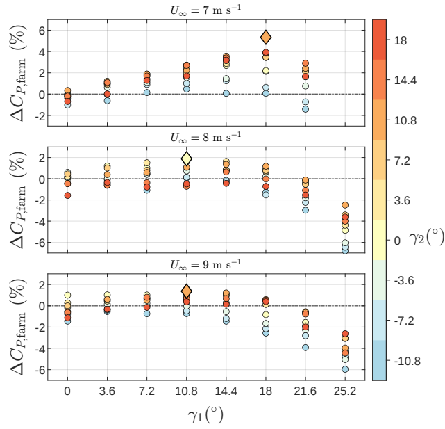
Figure 17. Farm power coefficient, normalized with its value in the greedy configuration, in three experiments with different free-stream velocities: (a) U_\infty = 7 \text{ m s}^{-1} , (b) U_\infty = 8 \text{ m s}^{-1} and (c) U_\infty = 9 \text{ m s}^{-1} . The abscissa and the color scheme denote the misalignment angles of the first and second rows, respectively. The diamonds indicates the respective farm-optimal configurations.
