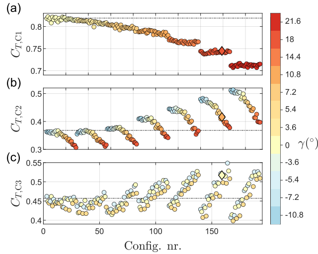
Figure 14. Thrust coefficient of turbines C1 (a), C2 (b) and C3 (c), measured during EXP2. The horizontal axis identifies the configuration number, following the chronological order in which the configurations were tested. The color scheme represents the value of \gamma of the corresponding turbine. The horizontal line indicates the thrust in the greedy configuration, while the diamond symbol denotes the farm-optimal configuration.
