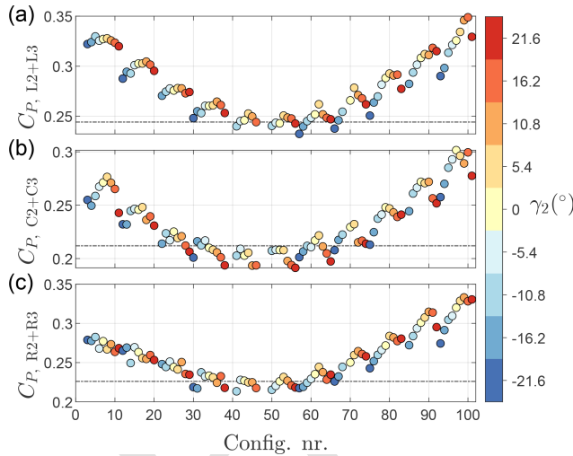
Figure 10. Sum of the C_P of the two downstream turbines in the left (a) , central (b) and right column (c) . The abscissas identify the configuration number in chronological order, as in Fig. 8. The colour scheme represents the yaw angle of the turbines in the second row. The horizontal dash-dotted lines represent the corresponding values in the greedy configuration.
