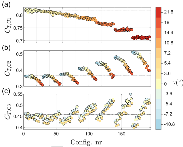
Figure 14. Thrust coefficient of turbines C1 (a), C2 (b), and C3 (c), measured during EXP2. The horizontal axis identifies the configuration number, following the chronological order in which the configurations were tested. The colour scheme represents the value of \gamma of the corresponding turbine. The horizontal dash-dotted lines indicate the thrust in the greedy configuration, while the diamond symbol denotes the farm-optimal configuration.
