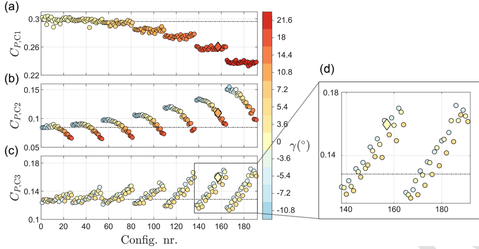
Figure 13. C_p of the central turbines C1 (a), C2 (b), and C3 (c). The abscissa identifies the configuration number, following the chronological order in which the configurations were tested. The colour scheme represents the value of \gamma of the corresponding turbine. The horizontal dash-dotted lines indicate the C_p value in the greedy configuration, while the diamond symbol denotes the farm-optimal configuration. (d) Magnified view of C_{p,C3} in the two last subgroups of configurations, in which \gamma_1 = 18^\circ and \gamma_1 = 21.6^\circ .
