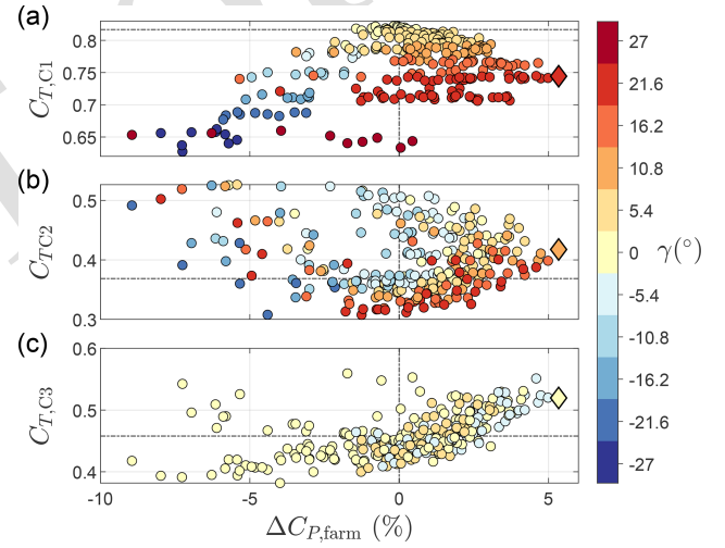
Figure 15. Thrust coefficient of turbines C1 (a), C2 (b), and C3 (c) versus the change in farm-power coefficient. The data from both EXP1 and EXP2 are included. The colour scheme represents the value of \gamma of the corresponding turbine. The horizontal dash-dotted lines indicate the T value in the greedy configuration, while the diamonds denote the farm-optimal case.
