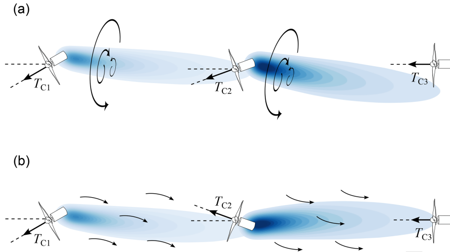
Figure 9. Qualitative representation of the most relevant flow phenomena in the two types of yaw configuration: (a) Type 1, in which both \gamma_1 and \gamma_2 are positive; and (b) Type 2, in which \gamma_1 > 0^\circ and \gamma_2 < 0^\circ .
