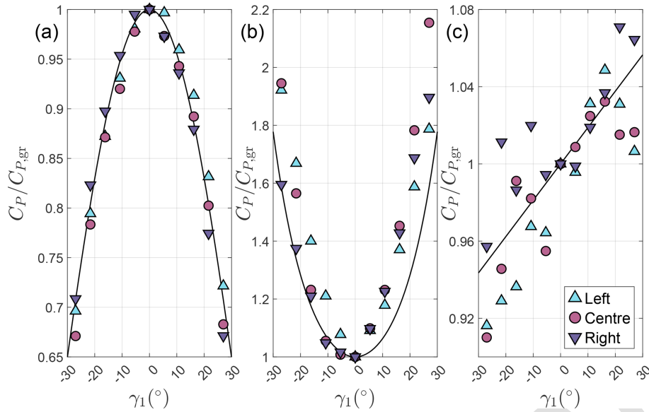
Figure 11. Variation of the power coefficients of the turbines in the first (a), second (b), and third row (c), normalized with the corresponding value in the greedy configuration and plotted as a function of \gamma_1 . The size of the symbols is representative of the uncertainty related to the zero alignment of the turbines, here assumed to be a single step of the stepper motors, i.e. 1.8^\circ . The solid lines in panels (a), (b), and (c) represent the functions \cos^3 \gamma_1 , an arbitrary even function, and a linear least-square fit, respectively. Note that the latter two are only used to assist the visualization.
