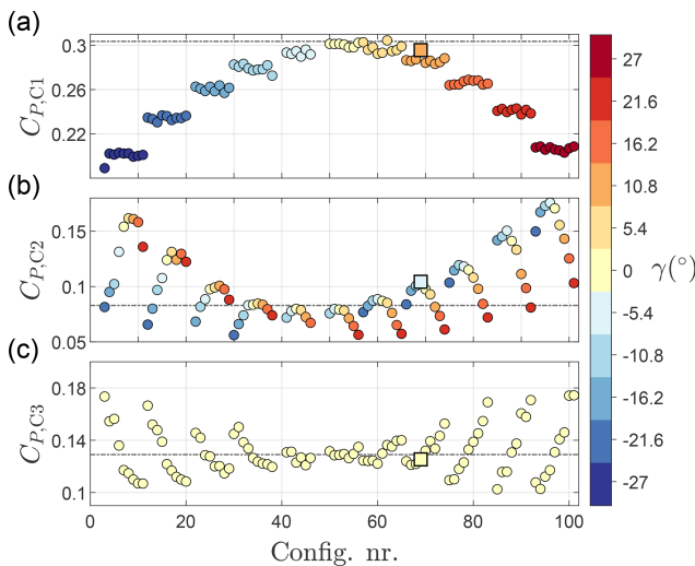
Figure 8. C_P of the central turbines C1 (a), C2 (b) and C3 (c). The abscissa denotes the configuration number, following the chronological order in which the configurations were tested. The colour scheme represents the value of \gamma of the corresponding turbine. The horizontal dash-dotted lines indicate the C_P value in the greedy configuration. The square symbols highlight an example of a high-performing Type 2 configuration.
