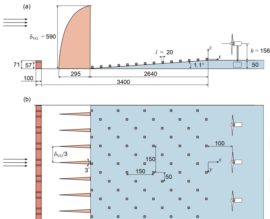
Figure 1. Side view (a) and top view (b) of the wind-tunnel test section (not to scale). The flow is from left to right. The castellated barrier is placed at the inlet of the test section, and the vortex generators are aligned with the castellations. The roughness elements are wooden cubes arranged in rows that are staggered in the lateral direction. Panel (a) also shows the foam boards positioned over the test section floor, with the concealed stepper motor installed at the base of the turbine tower depicted with a dashed line. All quotes are in millimetres.
