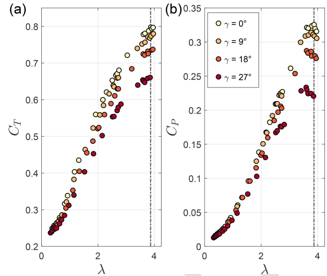
Figure 6. Thrust (a) and power (b) coefficient curves, as a function of the tip-speed ratio and of the yaw angle for turbine C3. The vertical dashed-dotted lines denote the optimal tip-speed ratio for \gamma = 0^\circ .
