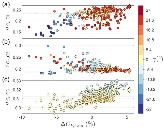
Figure 16. Standard deviation of the thrust coefficient time signals versus the change in farm-power coefficient. The data correspond to turbine C1 (a), C2 (b), and C3 (c). Both EXP1 and EXP2 are included. The colour scheme represents the value of \gamma of the corresponding turbine. The horizontal dash-dotted lines indicate the \sigma_T value in the greedy configuration, while the diamonds denote the farm-optimal case.
