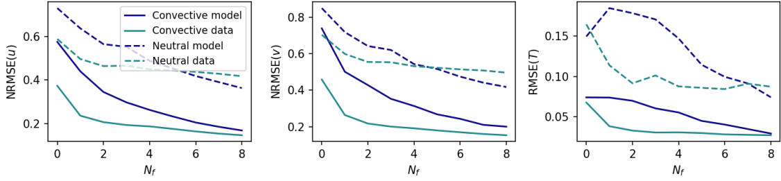
Figure 7. Median values of the NRMSE error metrics as a function of N_f for u' (left), v' (center), and T' (right). NRMSE is shown for velocity components; RMSE (K) is shown for temperature.
