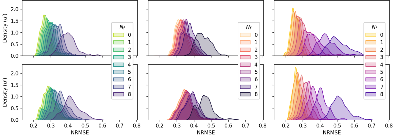
Figure 13. Distributions of the reconstruction error for AT retrievals of the u' component of velocity considering the convective (top row) and neutral (bottom row) flow cases. Error distributions correspond to use of the numerical correlation functions (left column), correlations from the respective precursor flows (center), and the modeled correlation functions (right column).
