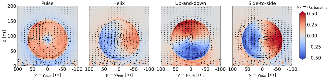
Figure 11. Phase-averaged, baseline-subtracted velocity fields at (x - x_{hub})/D = 0.1 . Phase averaging within the Strouhal cycle is performed with a 10^\circ bin centered on 0^\circ . After the phase averaging is performed for all cases, both the streamwise and lateral components of velocity are baseline-subtracted to yield the colored contours and the vector fields, respectively. The dashed lines outline the turbine rotor disk.
