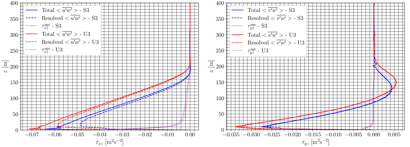
Figure 10. Comparison of total, resolved, and SGS fluxes of \overline{u'w'} (left) and \overline{v'w'} (right) for both S3 and U3 meshes.
