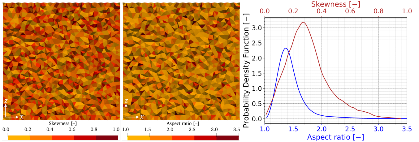
Figure 11. From left to right: XZ skewness plane at Y = 200\text{m} , XZ aspect ratio planes at Y = 200\text{m} , probability density function (PDF) of the skewness and the aspect ratio distribution for U3 mesh.
