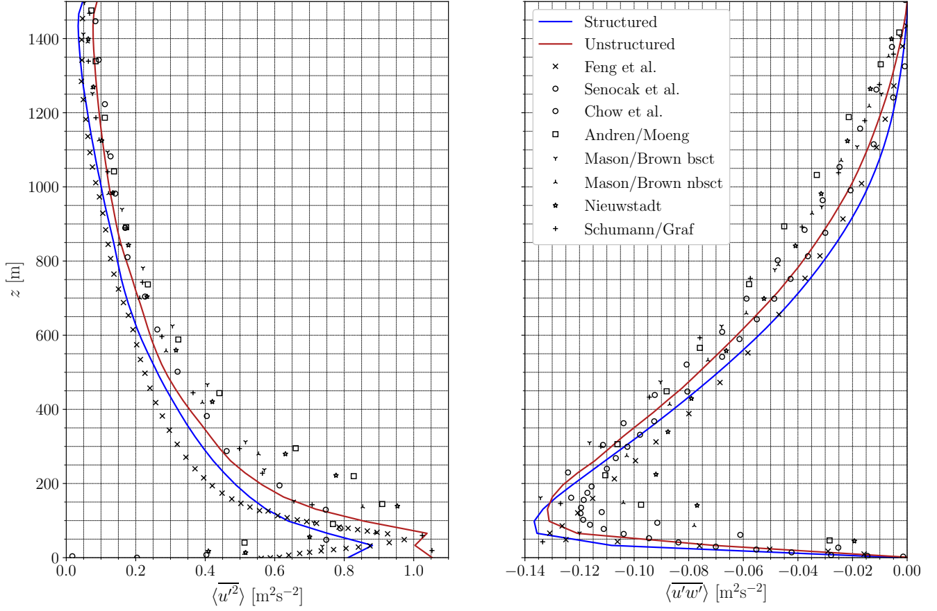
Figure 3. Time- and horizontally-averaged streamwise velocity variance and momentum flux profile of the Andrén case gathered on 28 h.
