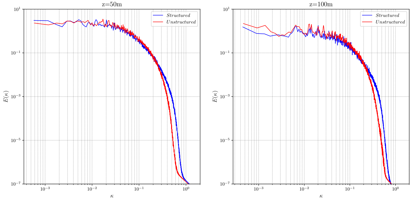
Figure 8. Energy spectra for structured (S3) and unstructured (U3) meshes at two different heights: z = 50 m (left) and z = 100 m (right).
