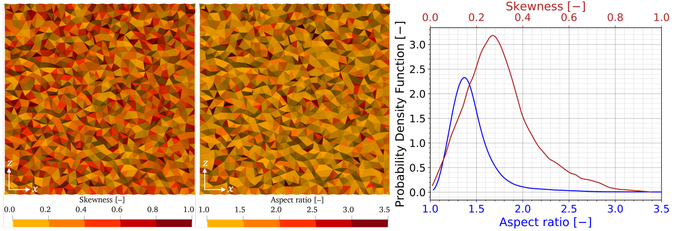
Figure 11. From left to right: x-z skewness plane at y = 200\text{m} , x-z aspect ratio planes at y = 200\text{m} , probability density function (PDF) of the skewness and the aspect ratio distribution for U3 mesh.
