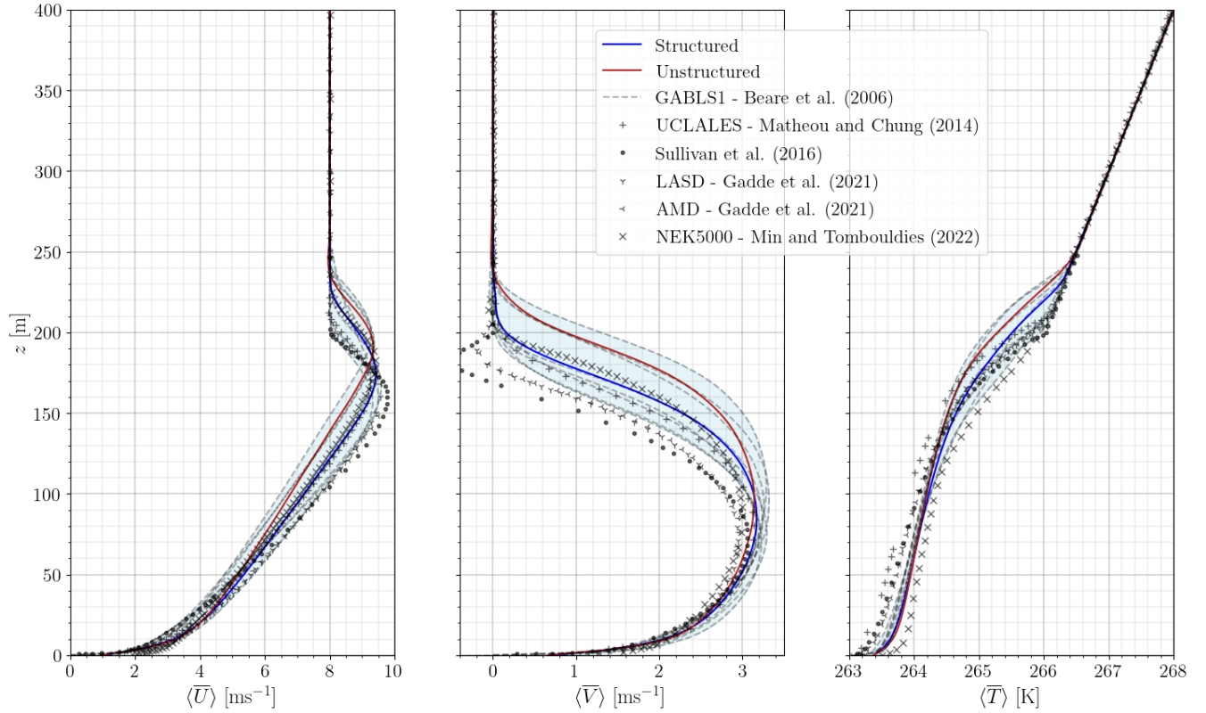
Figure 6. Time- and horizontally-averaged streamwise velocity, tangential velocity and temperature profiles, for meshes S3 and U3 with cell size \Delta x = 3.125 m. Blue shaded area stands for the original GABLS1 study results dispersion (Beare et al., 2006) and symbols for more recent studies (Matheou and Chung, 2014; Sullivan et al., 2016; Gadde et al., 2021; Min and Tomboulides, 2022).
