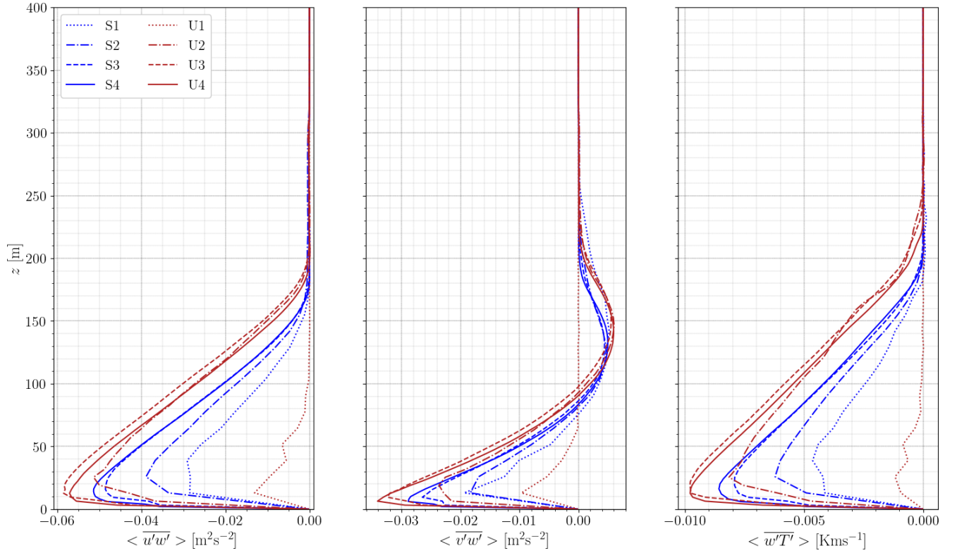
Figure 16. Time- and horizontally-averaged momentum and heat fluxes profiles.
