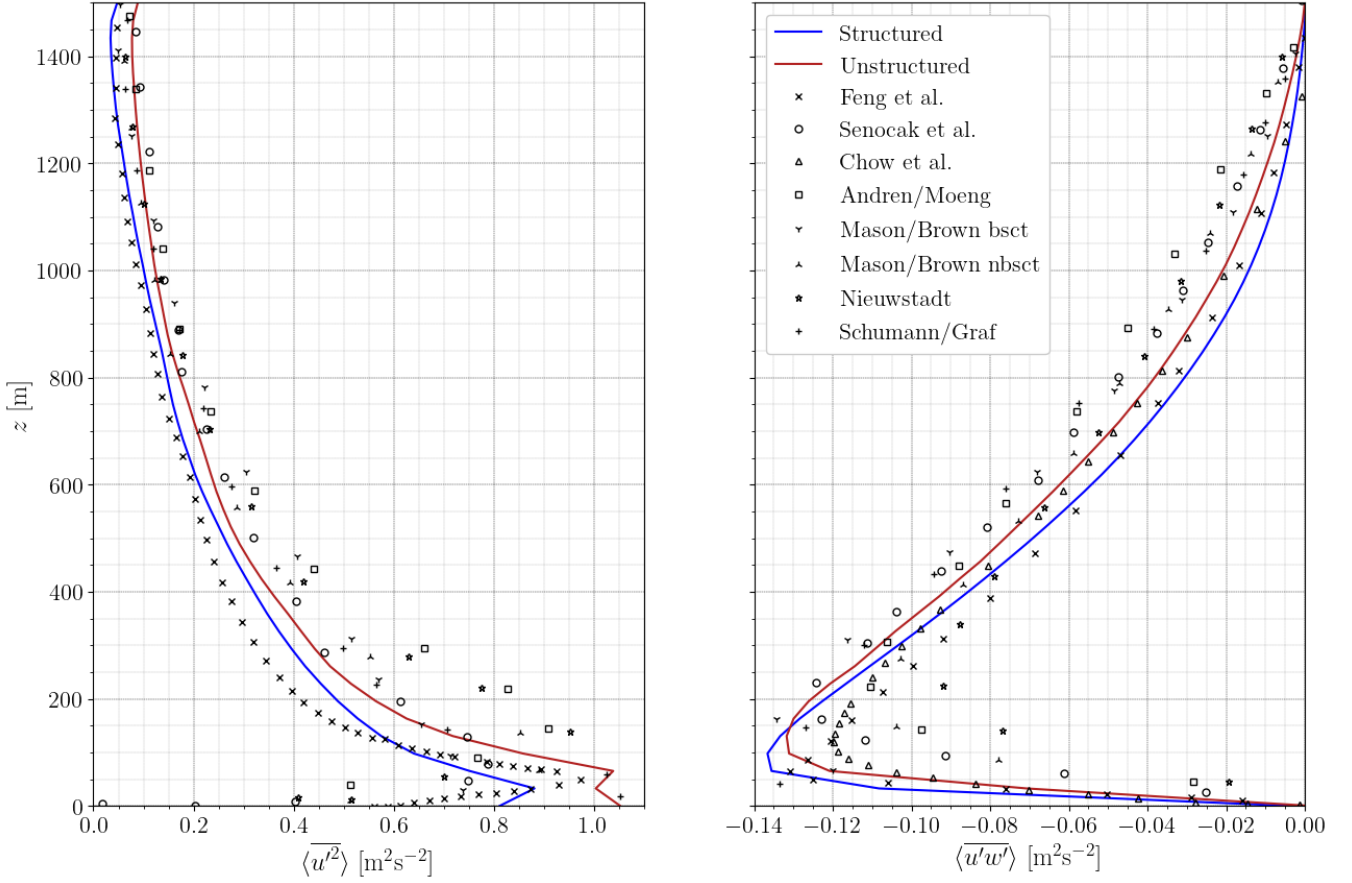
Figure 3. Time- and horizontally-averaged streamwise velocity variance and momentum flux profile of the Andren case gathered on 28 h.
