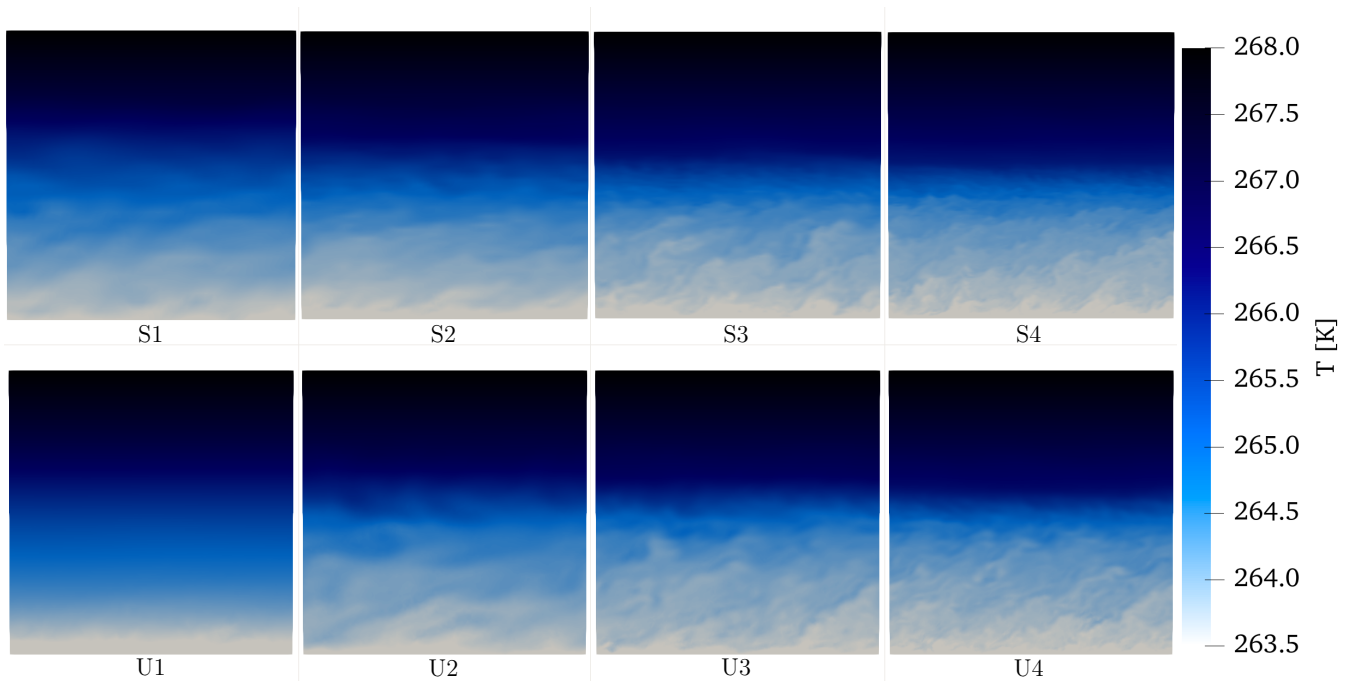
Figure 14. x-z temperature planes at y = 200\text{m} . Top: structured cases, bottom: unstructured cases. From left to right mesh resolution increases.
