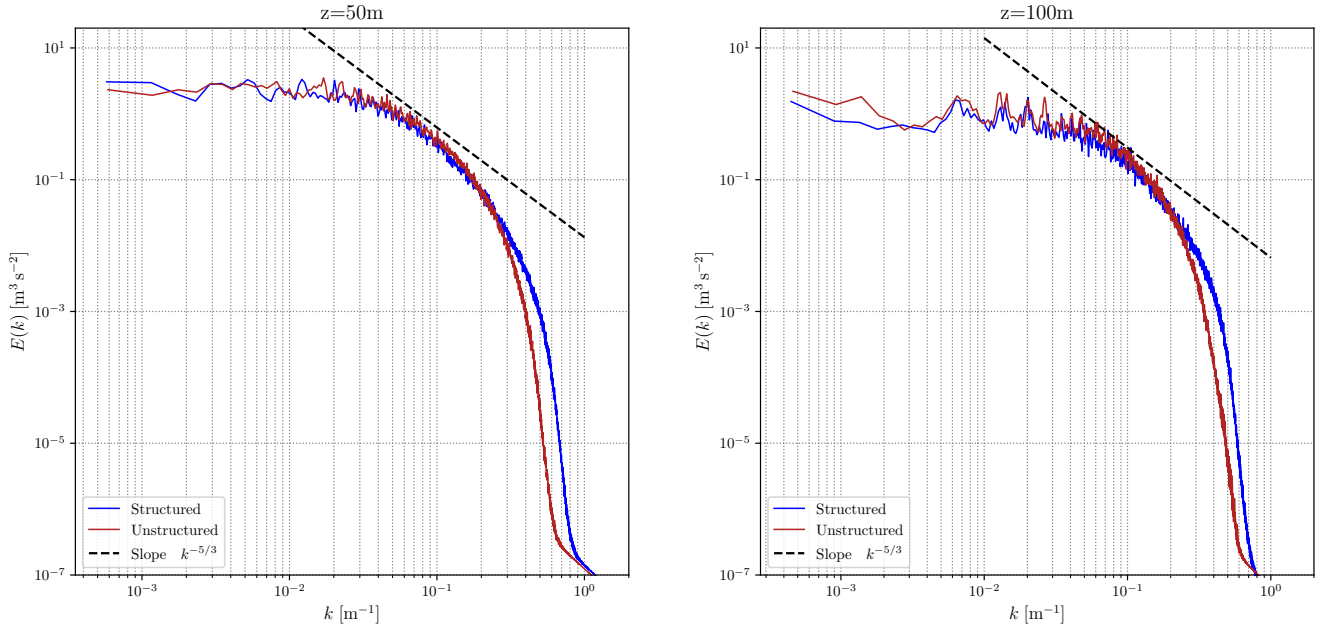
Figure 8. Energy spectra for structured (S3) and unstructured (U3) meshes at two different heights: z = 50 m (left) and z = 100 m (right). The Kolmogorov -5/3 reference slope is plotted to identify the inertial subrange.
