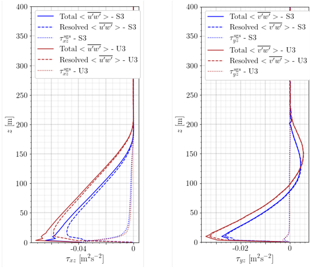
Figure 10. Comparison of total, resolved, and SGS fluxes of \langle \overline{u'w'} \rangle (left) and \langle \overline{v'w'} \rangle (right) for both S3 and U3 meshes.
