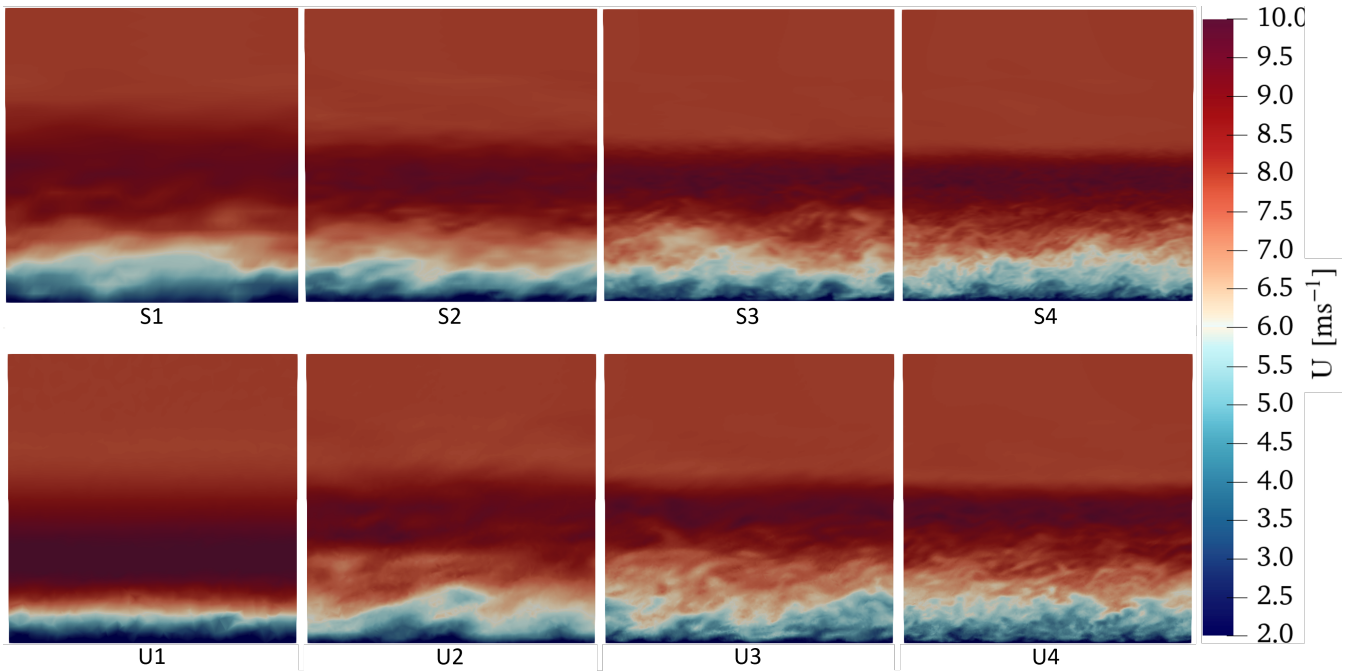
Figure 13. x – z velocity planes at y = 200 m. Top: structured cases, bottom: unstructured cases. From left to right mesh resolution increases.
