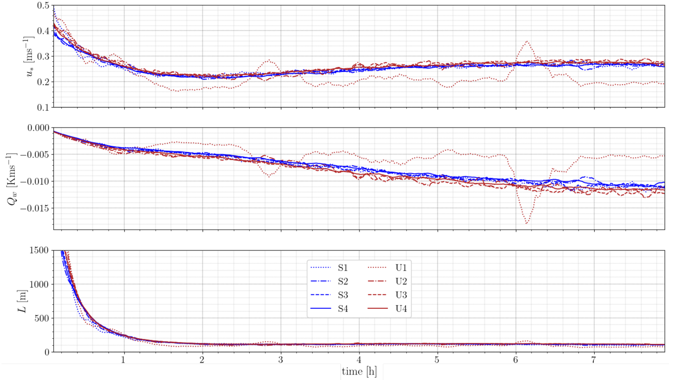
Figure 12. Friction velocity, wall heat flux, and Monin–Obukhov length time series.
