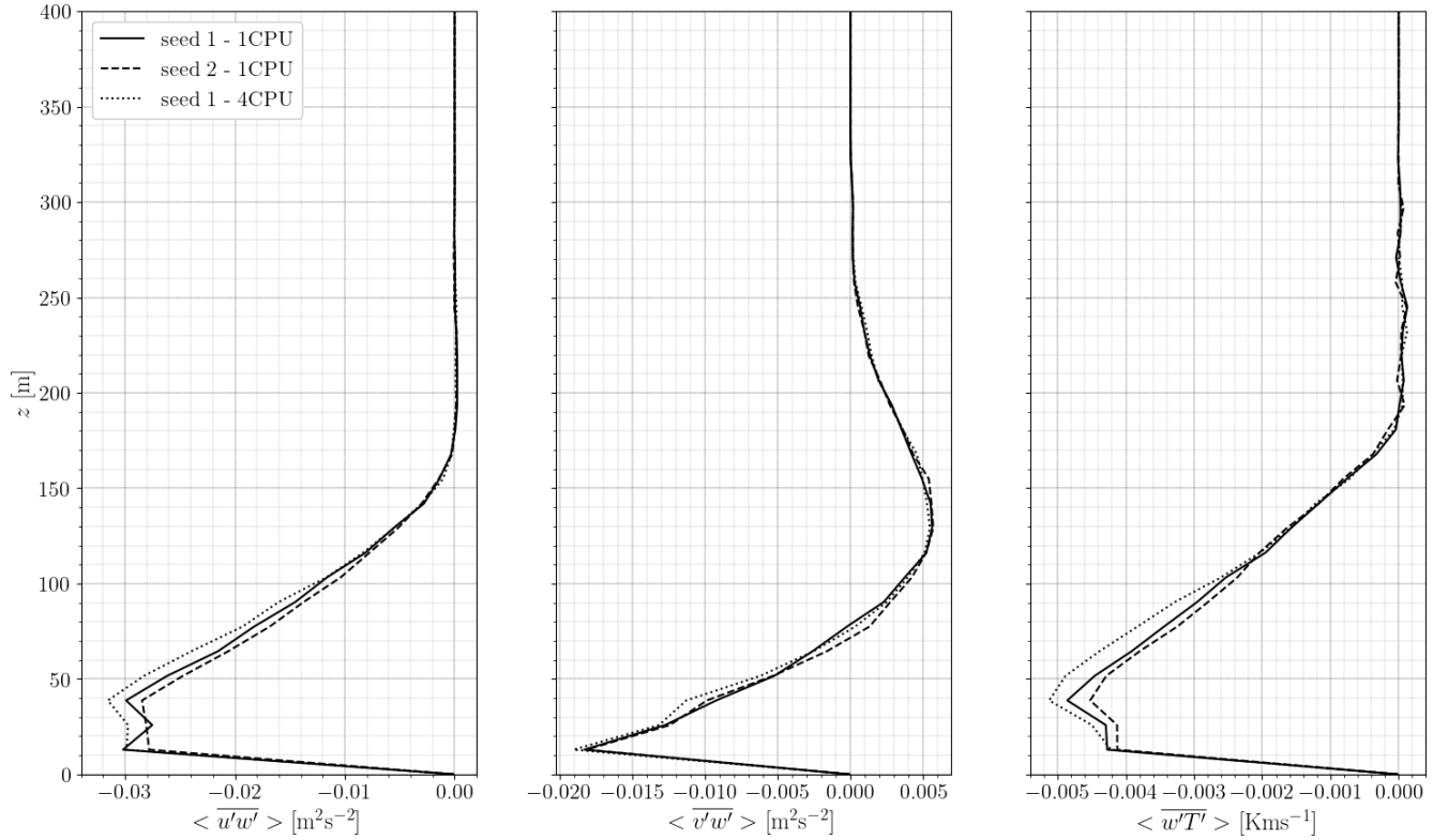
Figure B1. Time- and horizontally-averaged momentum and heat fluxes profiles on S1 mesh. Results with seed 1 and 1 CPU core (black solid line), seed 2 and 1 CPU Core (black dashed line) and seed 1 and 4 CPU cores (black dotted line).
