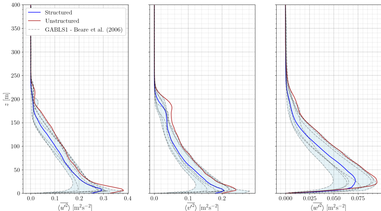
Figure 7. Time- and horizontally-averaged streamwise, tangential and vertical velocity variances profiles with S3 and U3 of cell size \Delta x = 3.125 m. Blue shading stands for the original GABLS1 study results dispersion (Beare et al., 2006).
