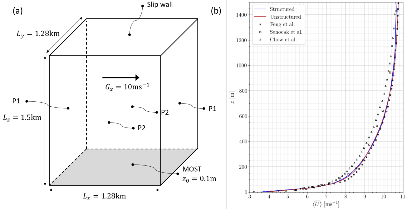
Figure 2. (a): Andren setup configuration scheme. P1 and P2 for periodic boundaries in pairs. (b): Average velocity profile of the Andren case gathered on 28 h.
