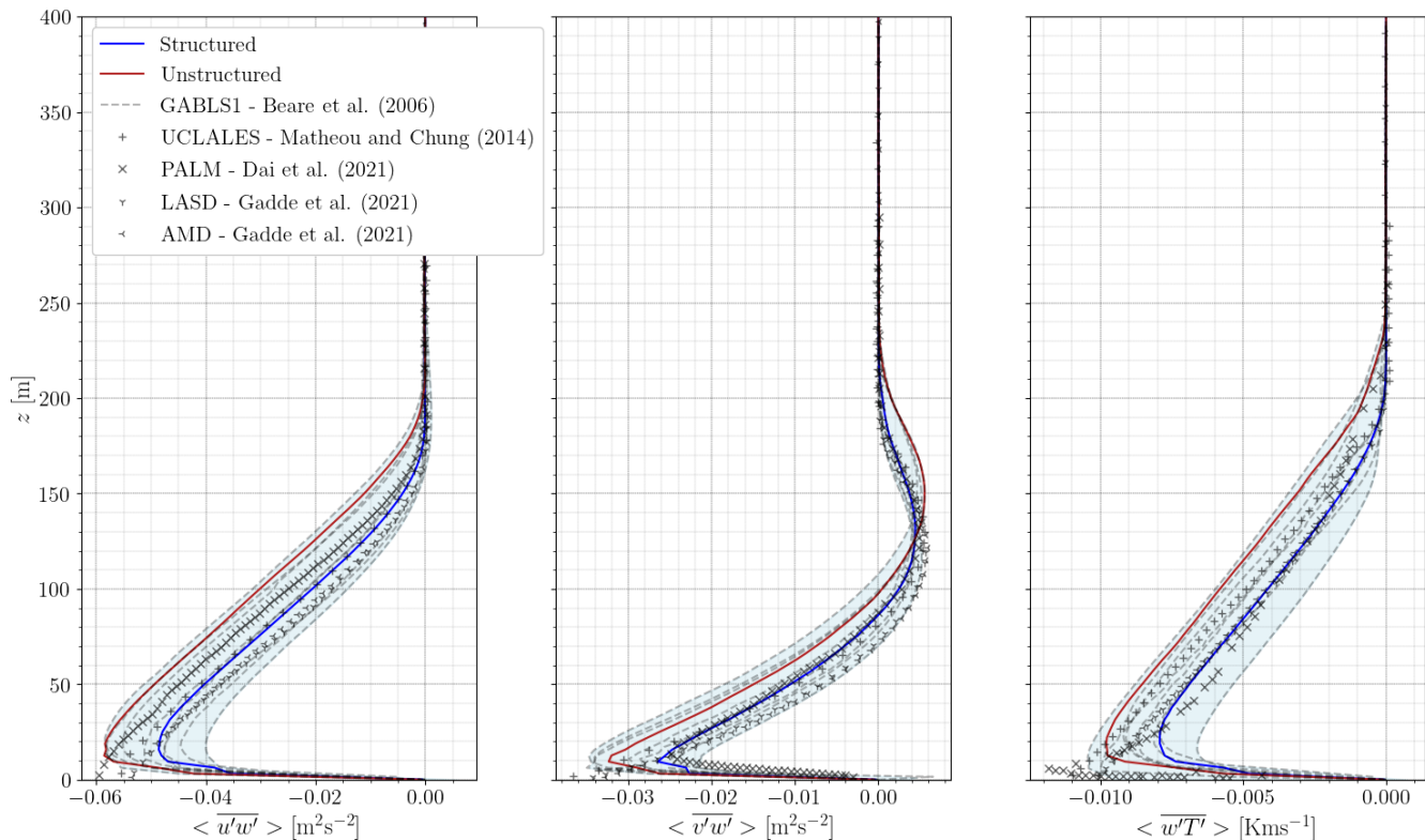
Figure 9. Time- and horizontally-averaged momentum and heat fluxes profiles for meshes S3 and U3 with cell size \Delta x = 3.125 m. Blue shading stands for the original GABLS1 study results dispersion (Beare et al., 2006) and symbols for more recent studies (Matheou and Chung, 2014; Dai et al., 2021; Gadde et al., 2021).
