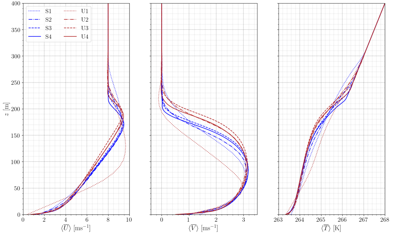
Figure 15. Time- and horizontally-averaged streamwise velocity, tangential velocity and temperature profiles.
