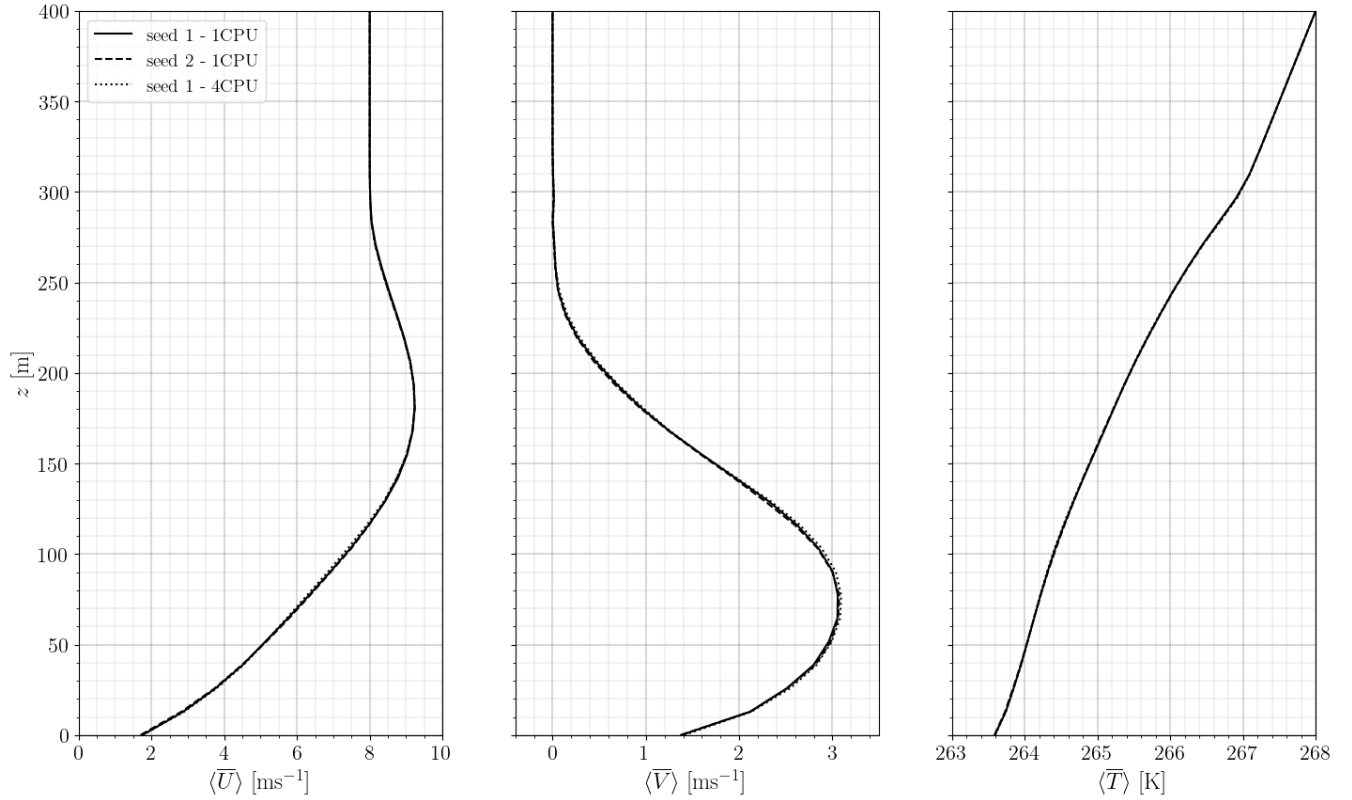
Figure A1. Time- and horizontally-averaged streamwise velocity, tangential velocity and temperature profiles on S1 mesh. Results with seed 1 and 1 CPU core (black solid line), seed 2 and 1 CPU Core (black dashed line) and seed 1 and 4 CPU cores (black dotted line).
