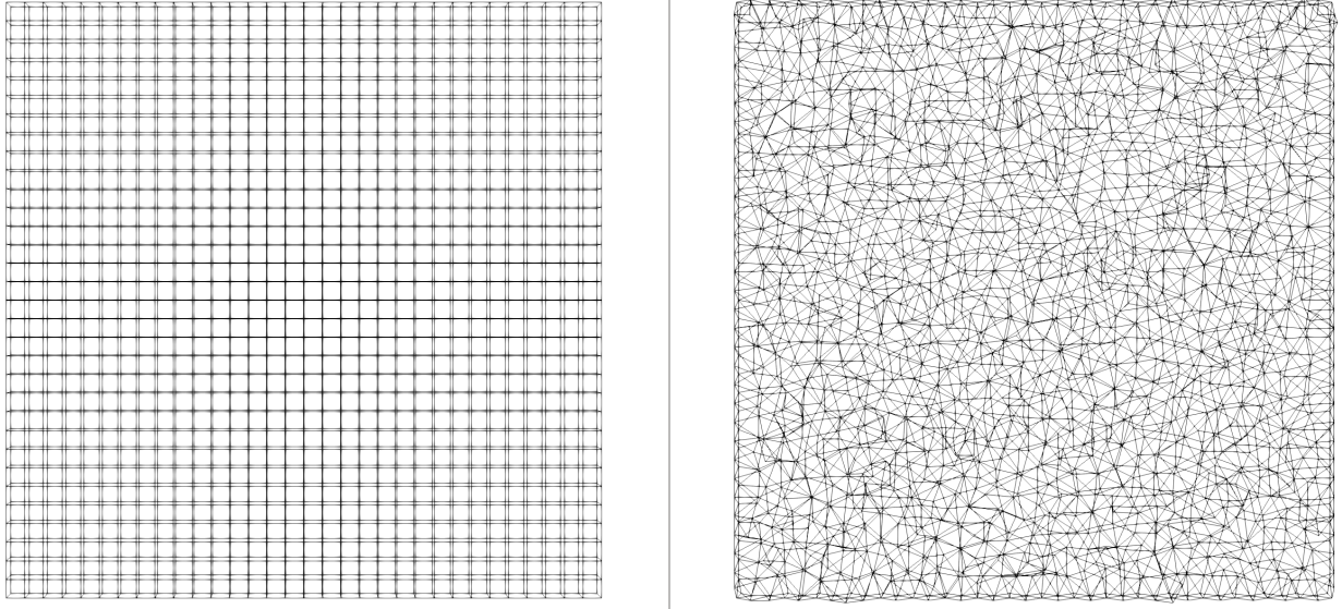
Figure 1. x-z crinkle slice at y = 200\text{m} for the \Delta x = 12.5\text{m} cell size mesh used in Section 4. Left: structured grid, Right: unstructured grid.
