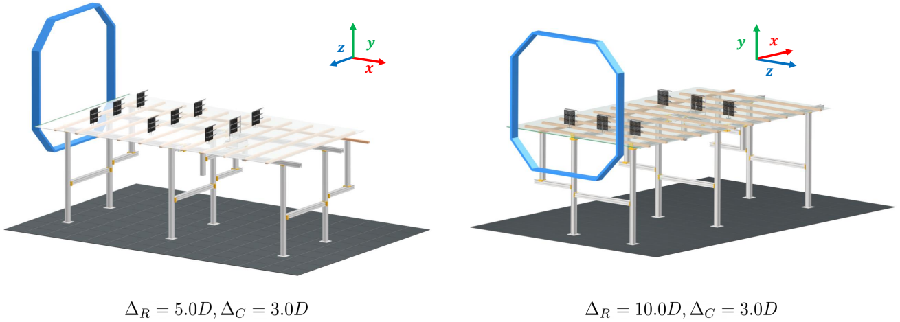
Figure 2. Illustration of the experimental setups for the regenerative wind farms with the aligned layout. The left panel shows a wind farm with a row spacing of \Delta_R = 5.0D and MRSLs in the Up-Washing configuration ( UW-05 ). The right panel shows a wind farm with \Delta_R = 10.0D and MRSLs in the Down-Washing configuration ( DW-10 ). The blue octagons represent the wind tunnel outlet. Note that the force measurement devices are installed in the last row of each setup.
