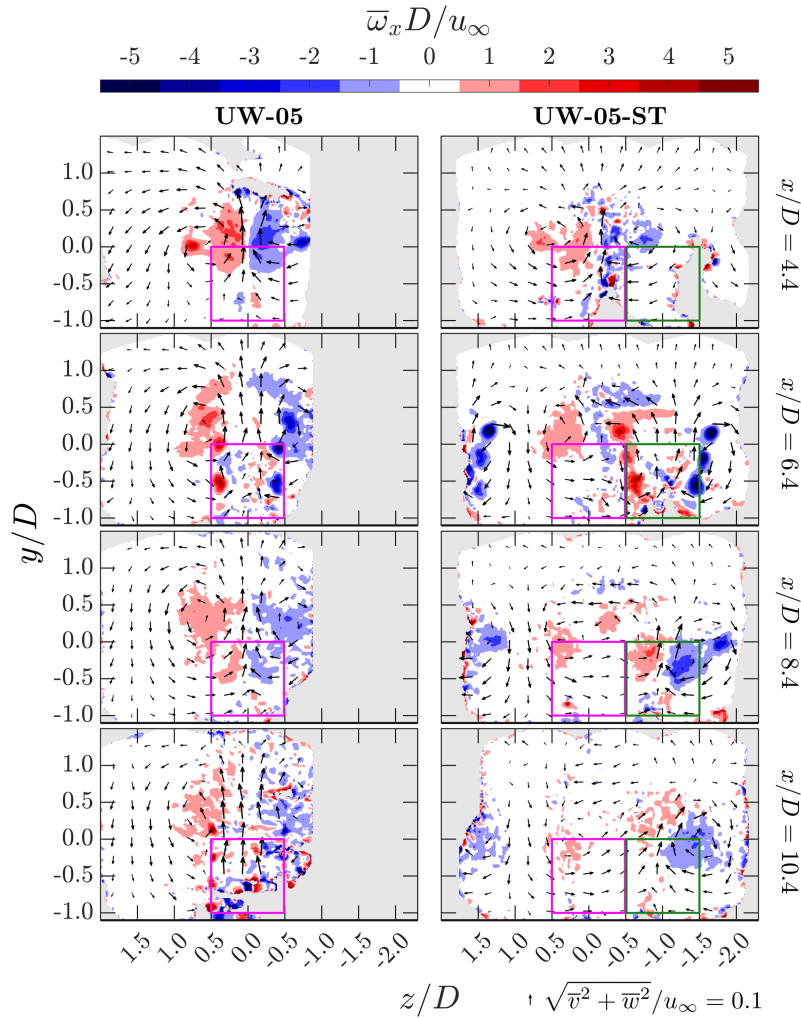
Figure 22. Contours of the time-averaged streamwise vorticity \bar{w}_x at selected x -planes for the two up-washing cases. The case with the aligned layout (case UW-05 ) and the staggered layout (case UW-05-ST ) are presented in the left and right column, respectively. The corresponding x -positions are indicated on the right side of each row. For the aligned case, MRSL projection areas are marked with magenta squares. For the staggered case, the projection areas of the 1 st - and 2 nd -row MRSLs (see Figure 7) are shown in magenta and dark green squares, respectively. In-plane velocity directions are represented by arrows scaled by their magnitude, with the reference scale provided at the bottom-right corner of the figure.
