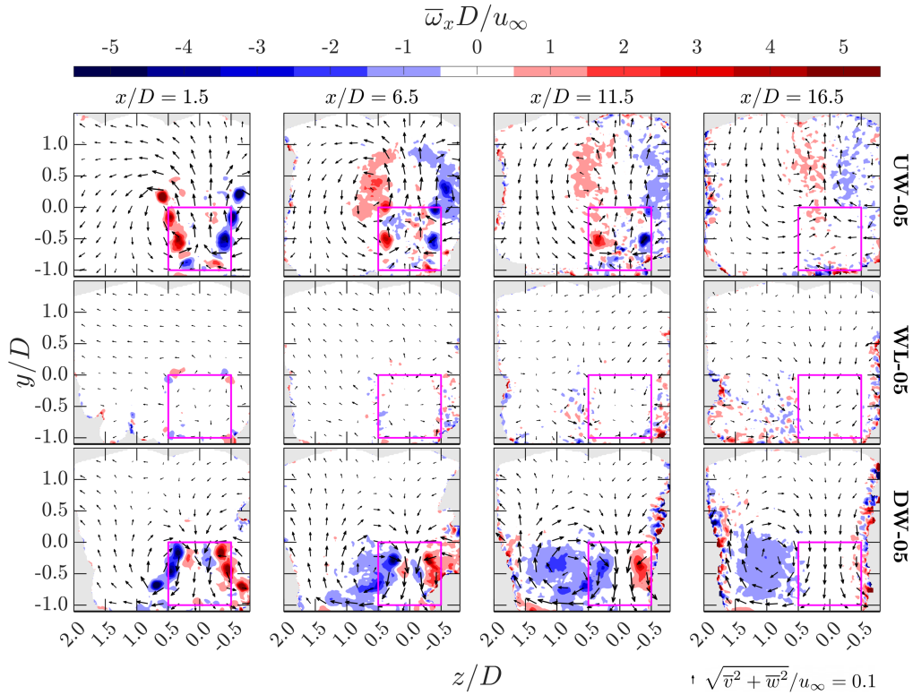
Figure 17. Contours of time-averaged streamwise vorticity ( \bar{\omega}_x ) for cases with a row spacing of 5D at several x -planes. Case labels are indicated on the right side of each row, and the corresponding x -positions are labeled at the top of each column. The projected areas of the MRSLs are marked with magenta squares. In-plane velocity directions are illustrated by arrows, scaled according to their magnitudes. The reference scale for the arrows is provided in the bottom-right corner of the figure. Note that the data have been filtered by spatial averaging over a spherical volume with a radius of 0.06D .
