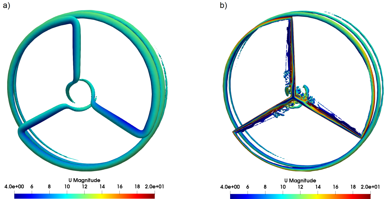
Figure 7. Isosurfaces of the Q-criterion for a) the LES-AL ( Q = 0.2 \text{ s}^{-2} ) and b) the LES-BL ( Q = 1.2 \text{ s}^{-2} ) visualised with the flow velocity.
