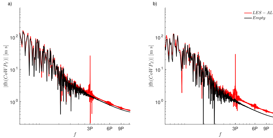
Figure 18. FFT of the CoWP in LES 200 m downstream the inflow (figure 17) ( 3P = 0.605 Hz).
