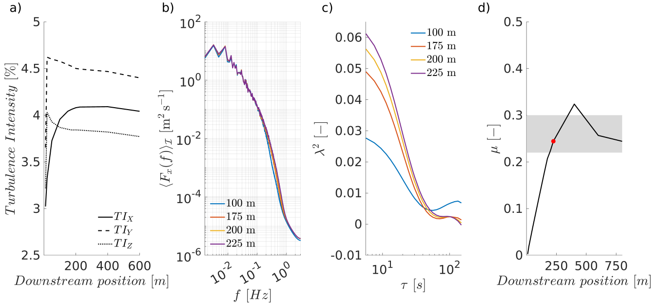
Figure 14. Analysis of turbulence without a turbine. Turbulence intensity over downstream position a) Energy spectrum of different downstream positions b) Shape parameters of the two-point statistics over the increment size c). Downstream development of the intermittency parameter \mu .
