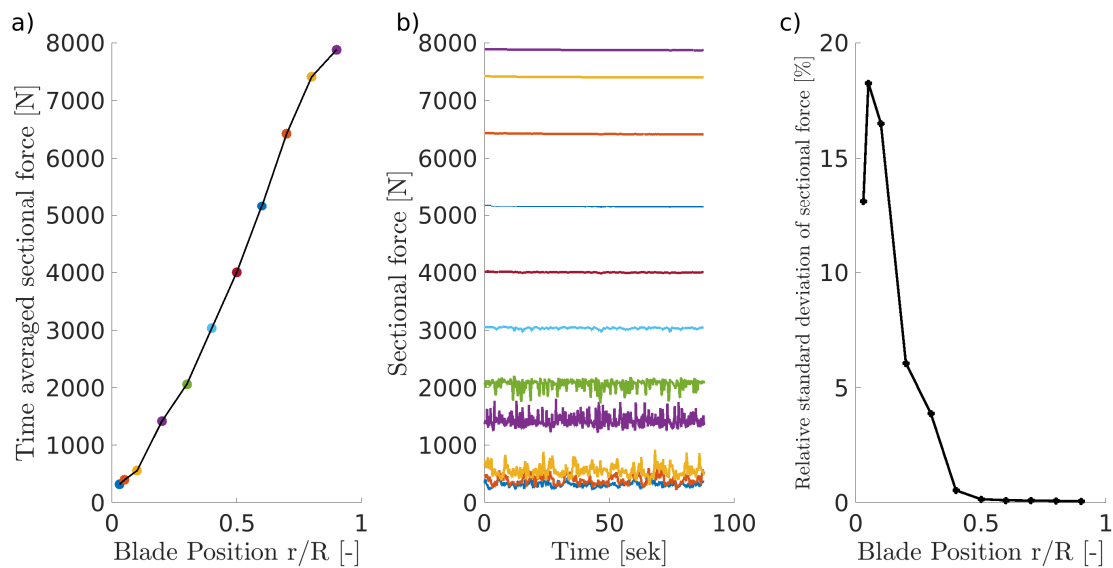
Figure 8. Sectional forces of a blade resolved simulation with laminar inflow. Time-averaged sectional forces over blade radius a). Time-series of the sectional forces b). Relative standard deviation of the sectional forces over blade radius.
