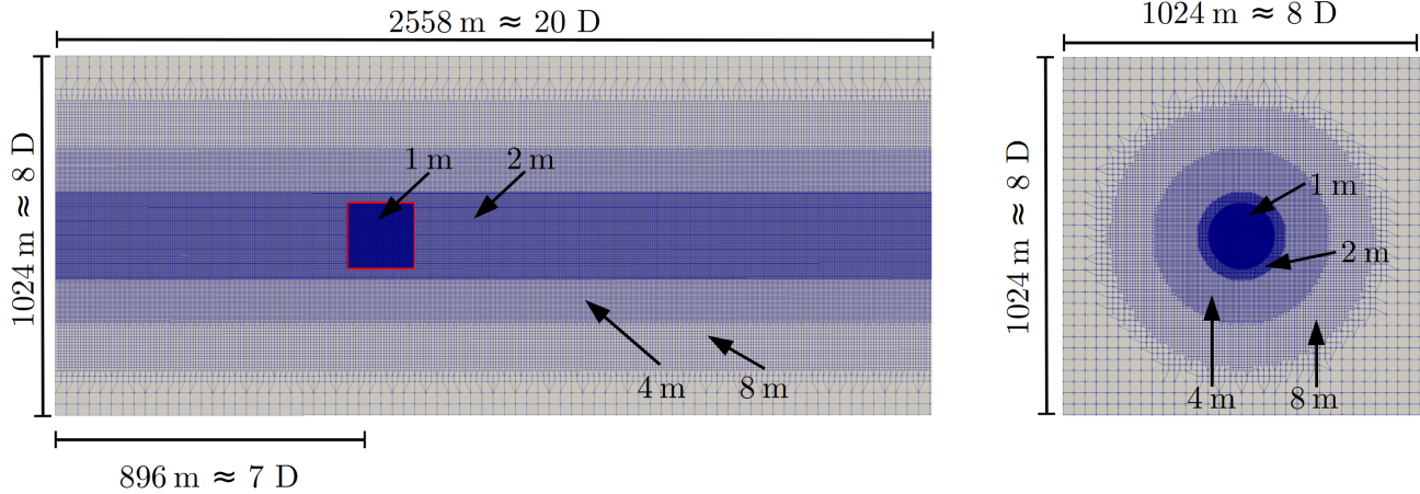
Figure 2. Cutting slices of the grid.
