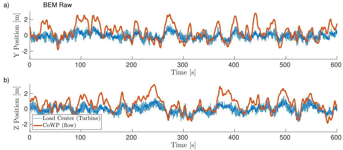
Figure 11. Time-series of the CoWP from the synthetic inflow field and the Load center of the BEM simulation. Y component in a) and Z component in b).
