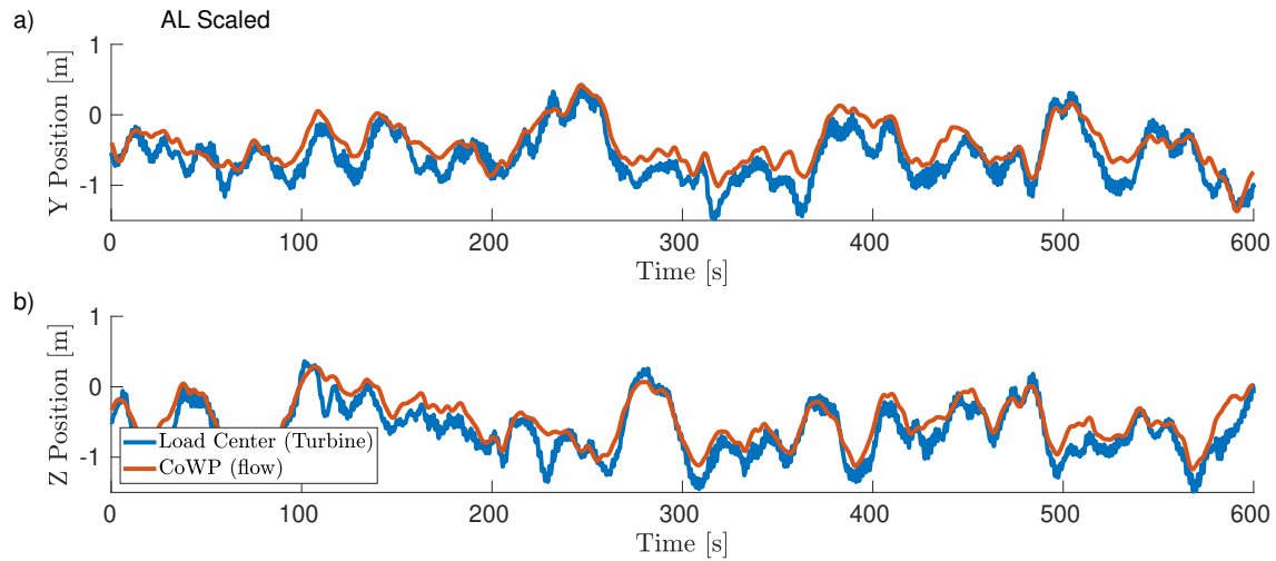
Figure 20. Time-series of the scaled CoWP from LES in the rotor plane and the filtered Load center of the LES-AL. Y component in a) and Z component in b). r_{Pearson} = 0.908 .
