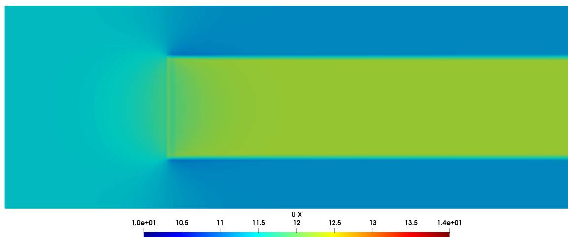
Figure C1. Time-averaged velocity field from a LES with velocity jump achieved by an actuator.
