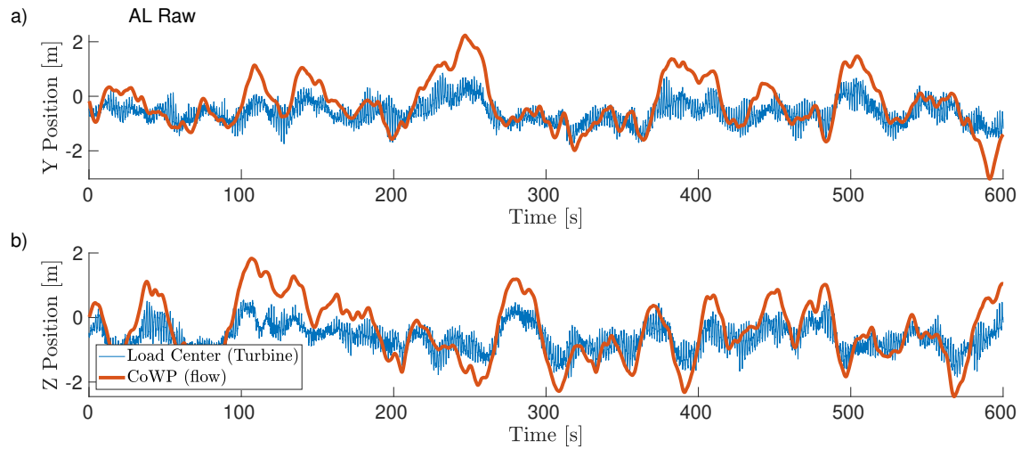
Figure 19. Time-series of the CoWP from LES in the rotor plane and the Load center of the LES-AL. Y component in a) and Z component in b).
