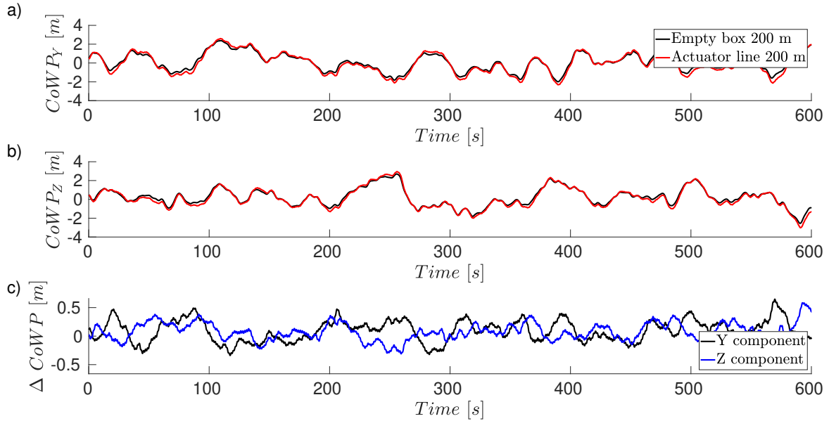
Figure 17. Time-series of the CoWP 200 m downstream the inflow without turbine (black) and with LES-AL modelled turbine (red) in a) and b). Absolute difference between the simulation with and without turbine in c).
