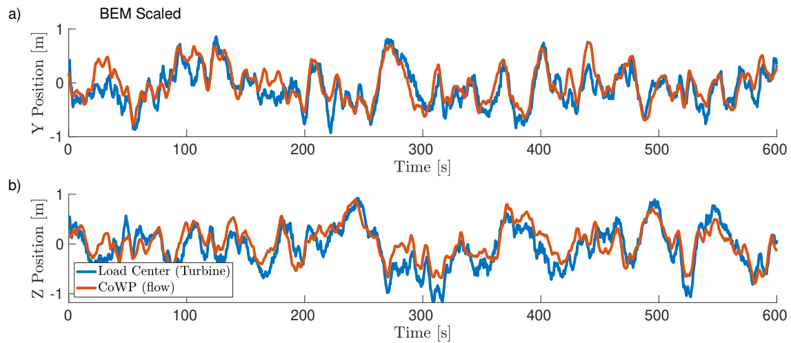
Figure 12. Time-series of the scaled CoWP from the synthetic inflow field and the filtered Load center of the BEM simulation. Y component in a) and Z component in b). r_{Pearson} = 0.814 .
