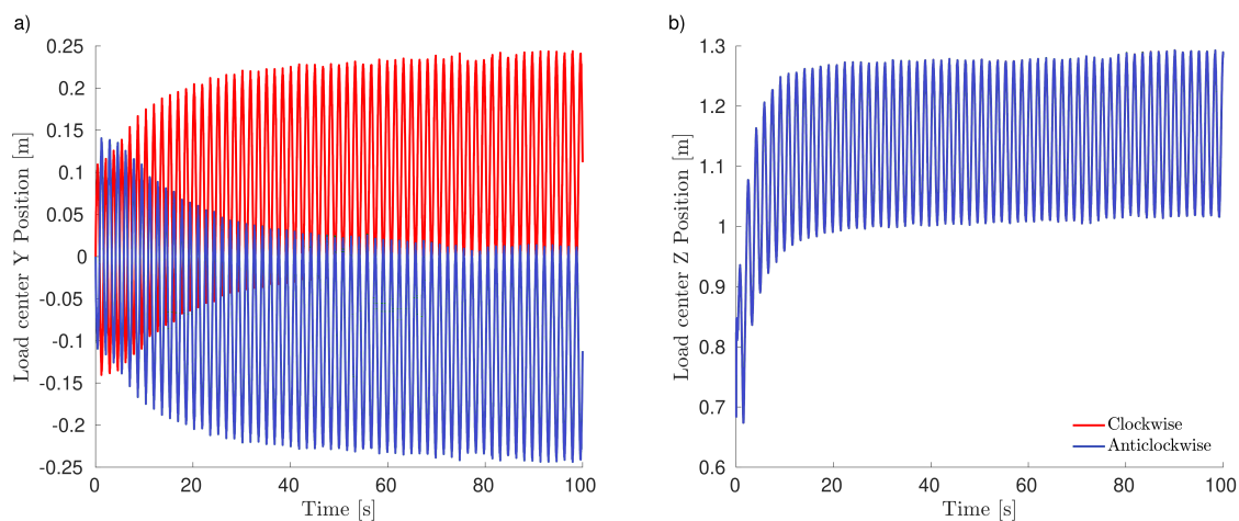
Figure B1. Time series of the Load center for LES-AL simulations with different rotational directions.
