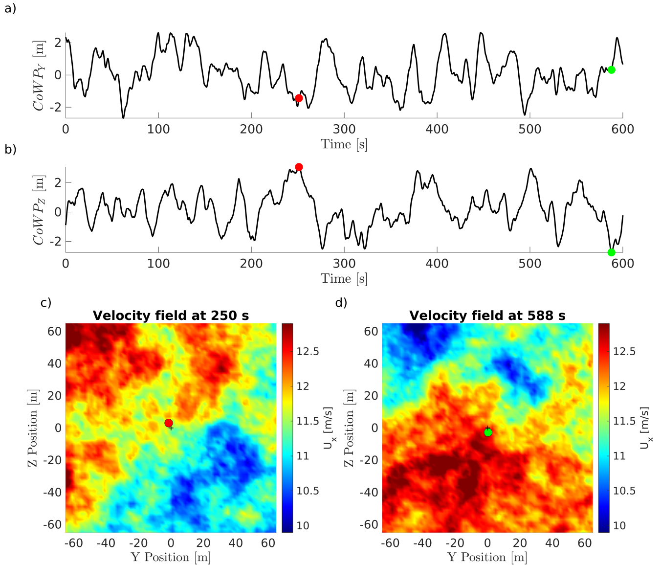
Figure 1. Time series of the CoWP a) and b). Slice of a field generated by a synthetic turbulence model in c) and d). The CoWP locations are shown by the red and green dots. The center of the slice is shown by the black cross.
