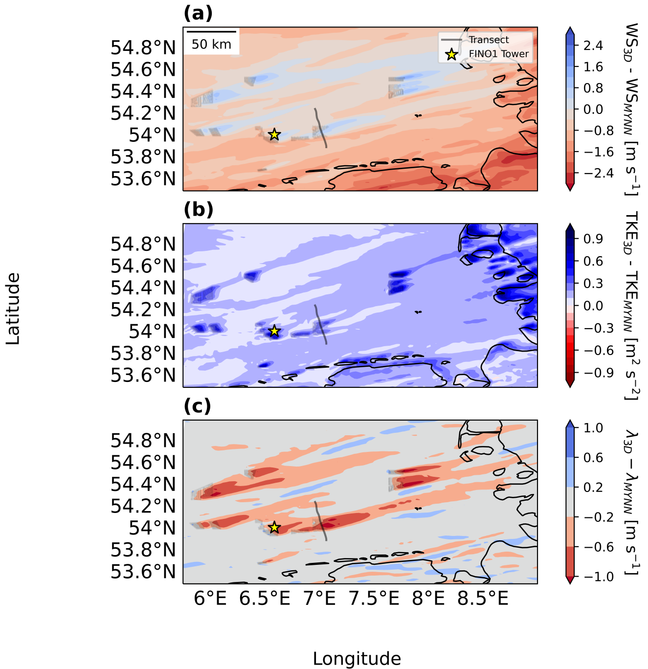
Figure 8. Difference fields for inner region at a 100 m hub height . (a) 3fa_025 - mfa_025 WS; (b) 3fa_025 - mfa_025 TKE; (c) 3fa_025 - mfa_025 wake deficit. Turbines are marked with black circles, the FINO1 tower is marked with a yellow star, and the first transect path is marked with a solid line.
