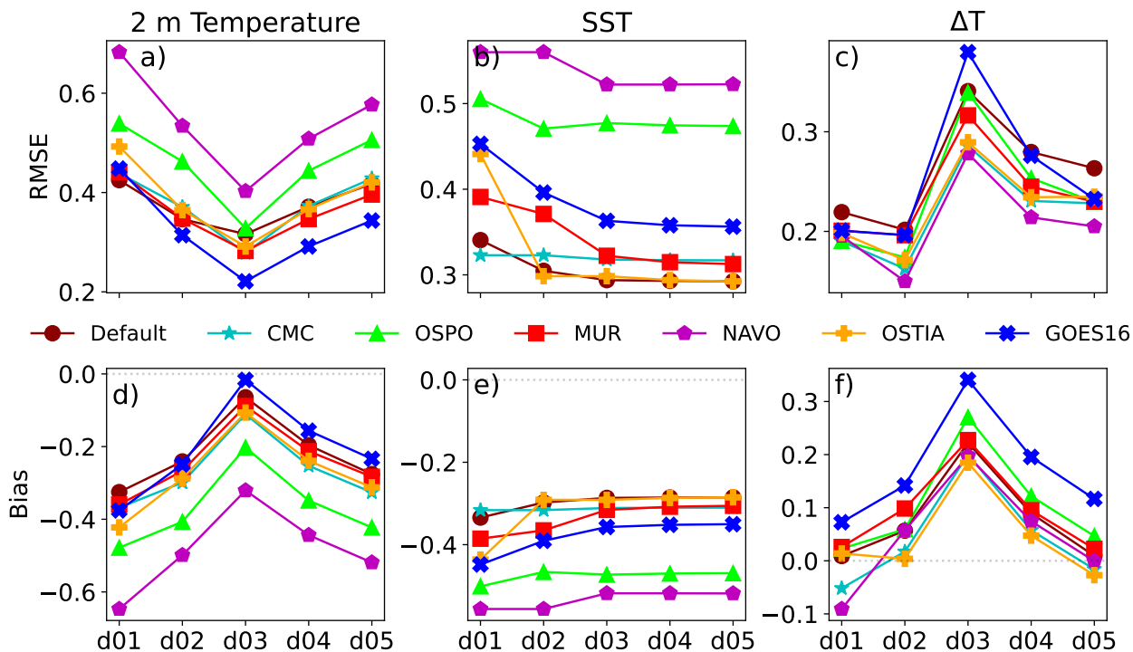
Figure 12. Same as Figure 11 but for 2-m temperature, SST, and \Delta T .
