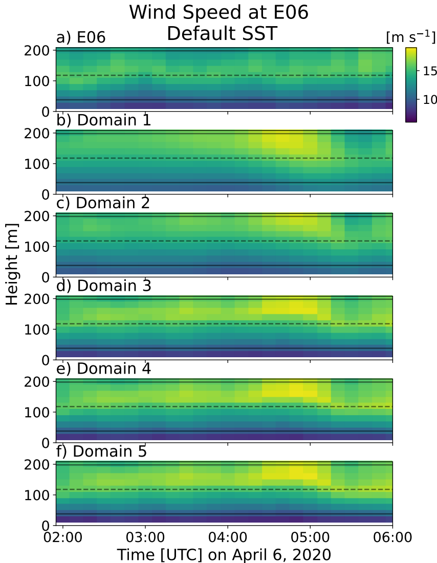
Figure 5. Vertical profiles of wind speed with time for observations (a), and domains 1, 2, 3, 4, and 5 (b–f, respectively) for the Default SST setup during the period of interest. The assumed hub height (dashed line) and rotor layer (between the solid lines) in this study are also shown.
