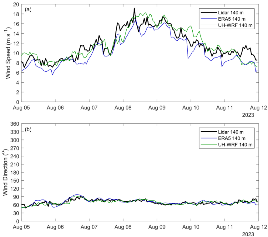
510 Figure 17. Observed and modelled (a) wind speeds and (b) wind directions at the lidar buoy location during the August 2023 Hawai'i wind event.
