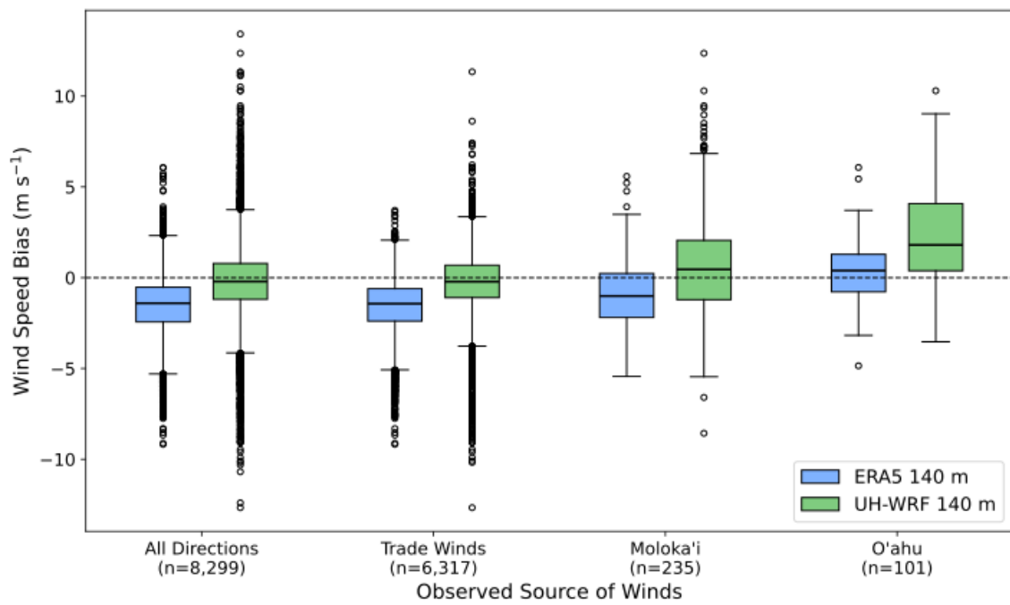
Figure 9. ERA5 and UH-WRF wind speed bias according to observed 140 m wind direction. The trade winds are defined as sourcing between 50° and 100°; Moloka'i-sourced winds are defined between 110° and 150°; O'ahu winds are defined between 230° and 300°. Data counts for each source are shown below their labels.
