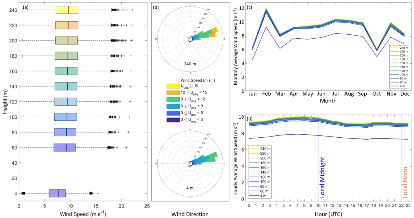
Figure 2. Observed (a) wind speed, (b) wind direction, (c) monthly average wind speed, and (d) hourly average wind speed by height a.s.l. from the Hawai'i lidar buoy during 1 January 2023 – 15 December 2023. Measurements at 60 m and higher source from the onboard lidar system (DOE, 2025a) while measurements at 4 m source from the onboard surface meteorological station (DOE, 2025b).
