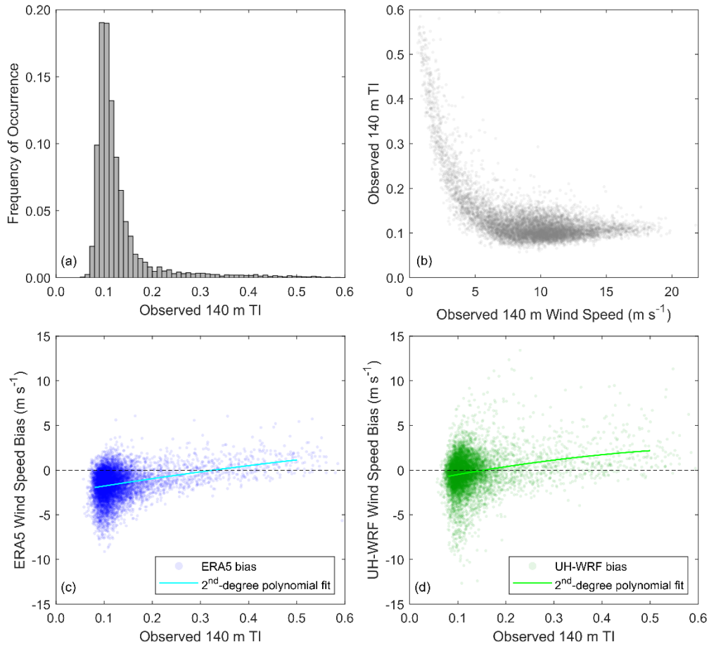
340 Figure 10. (a) Distribution of TI at 140 m during the Hawai’i lidar buoy deployment, (b) observed TI according to observed 140 m wind speed, and (c) ERA5 and (d) UH-WRF 140 m wind speed bias according to observed TI.
