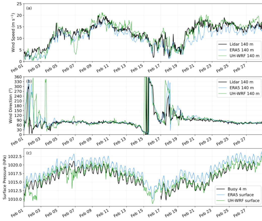
Figure 15. Observed and modelled (a) wind speeds and (b) wind directions and at 140 m; (c) observed 4 m surface air pressure at the lidar buoy location during February 2023- for buoy observation, ERA5, and UH-WRF.
