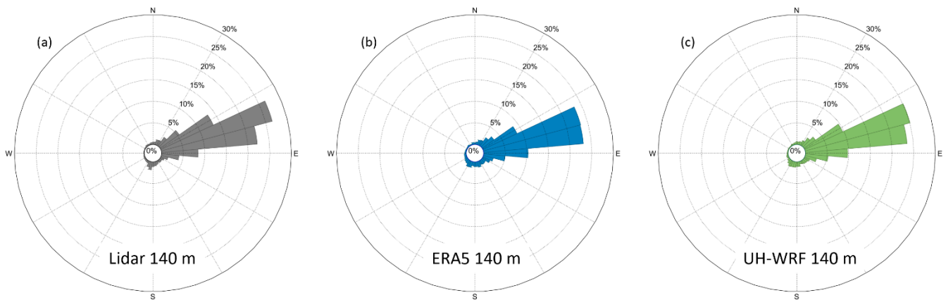
305 Figure 8. Wind direction distributions at 140 m from (a) the O'ahu lidar buoy, (b) ERA5, and (c) UH-WRF between 1 January and 15 December 2023.
