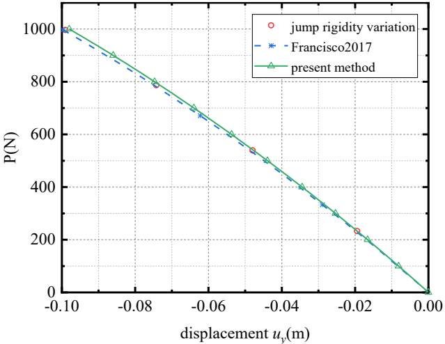
(b) u_y Displacement at node 13
