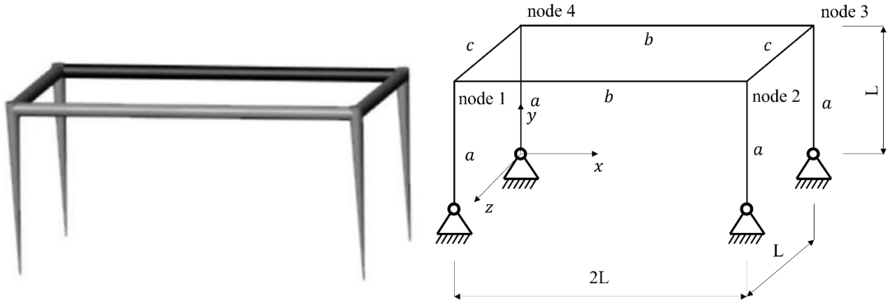
Figure 12: Frame displacement at node 13 (Murín, 2002)
