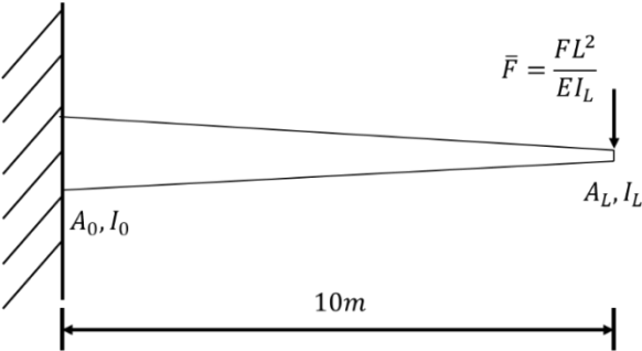
Figure 7: Conical beam
