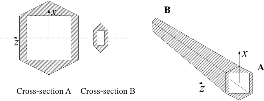
Figure 10: Column geometry
