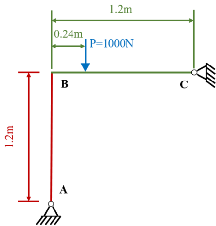
Figure 9: Frame scheme
