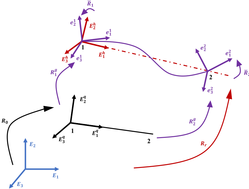
Figure 2: Beam kinematics and coordinate systems
