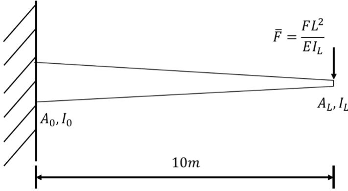
Figure 7. Conical beam
