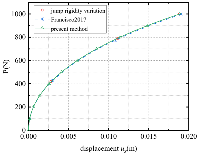
(a) u_x Displacement at node 13
