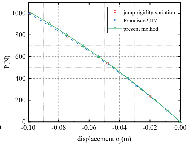
(b) u_y Displacement at node 13
