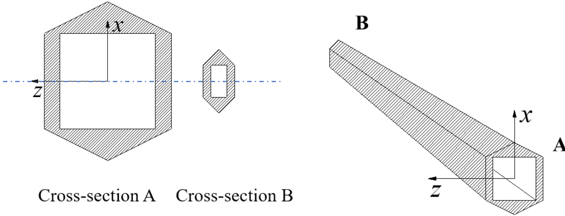
378 Figure 10. Column geometry
