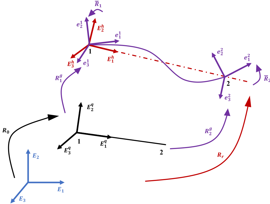
Figure 2: Beam kinematics and coordinate systems
