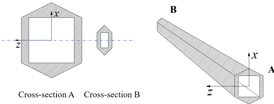
Figure 10: Column geometry
