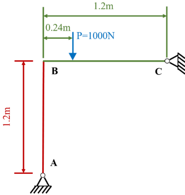
Figure 9: Frame scheme
