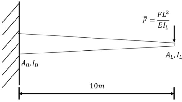
Figure 7: Conical beam
