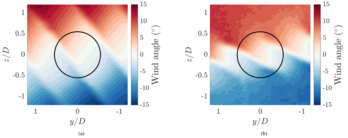
Figure 19. Flow characterization contours of variation of wind veer in the yz -plane at x/D = 0 (a) Veer 10^\circ ; (b) Veer 20^\circ . The solid circle represents the frontal projection of the porous disc.
