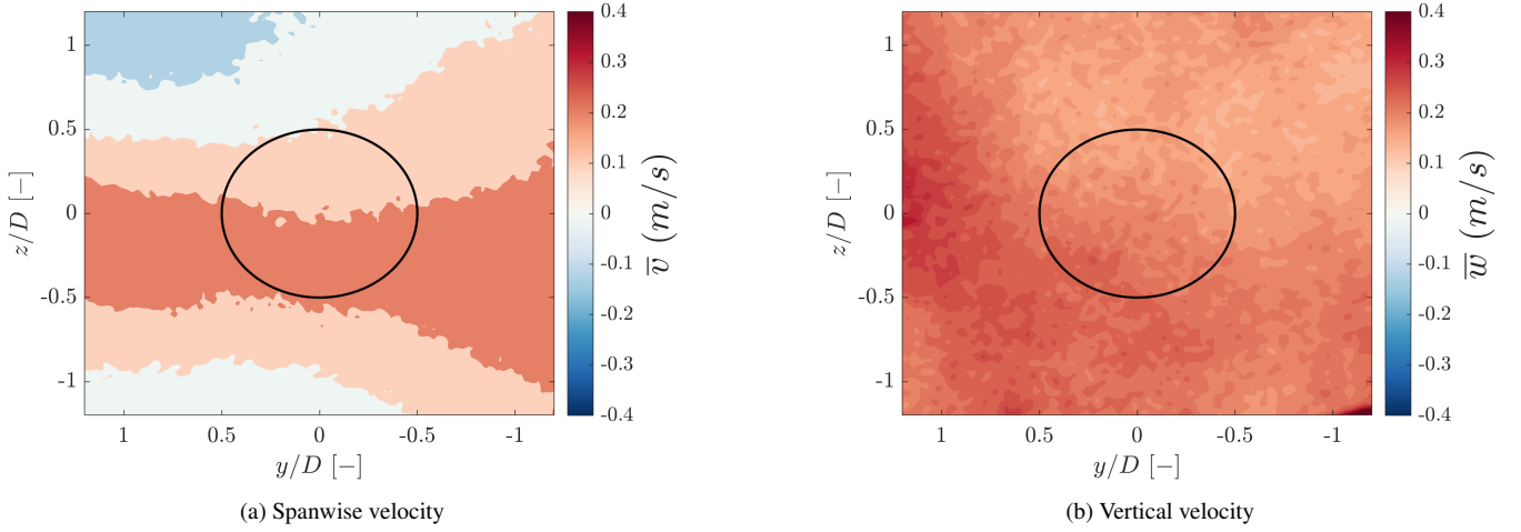
Figure A1. Flow characterization contours in the yz -plane for the clean case in the absence of porous disc at x/D = 0 : (a) Spanwise velocity; (b) Vertical velocity. The solid circle represents the frontal projection of the disc.
