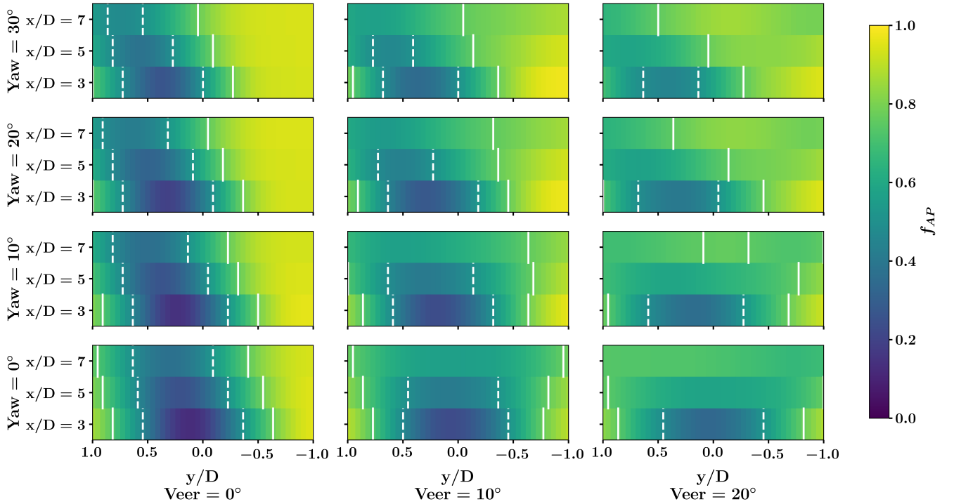
Figure 18. Filled contour of available power distribution (Eq. 11) for all cases at three different downstream locations. f_{AP} is computed by integrating U^3 over the frontal projection area of the porous disc centered at y/D and normalizing by the corresponding integral of the inflow U^3 over the same area. The disc projection is then traversed laterally across the wake to produce the distributions shown. The solid vertical line represents the locations where f_{AP} is 0.75 and the dashed vertical line represents locations where f_{AP} is 0.5.
