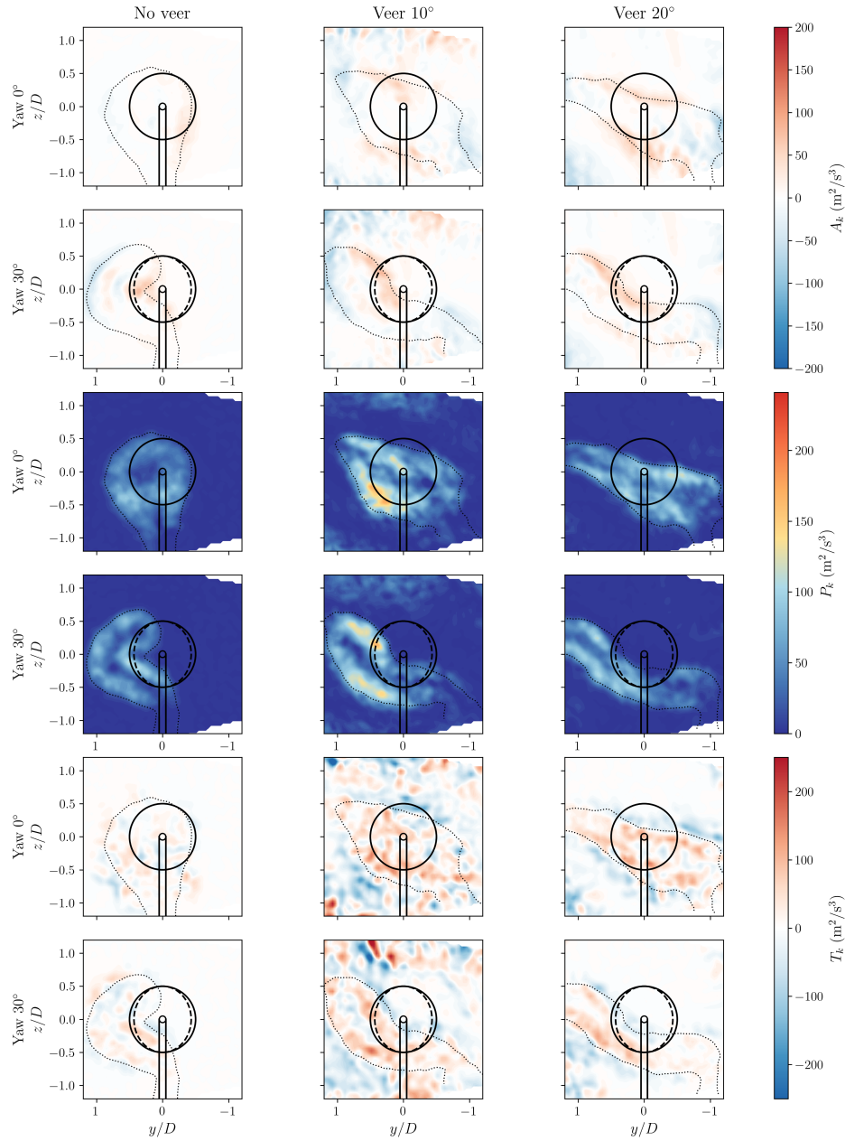
Figure 16. Spatial distribution of terms in Eq. 10 at x/D = 5 . The solid circle represents the frontal projection of the yawed porous disc, whereas the dashed circle represents the yawed disc of 30^\circ . The dotted line indicates the wake boundary where u/U_{ref} = 0.9 .
