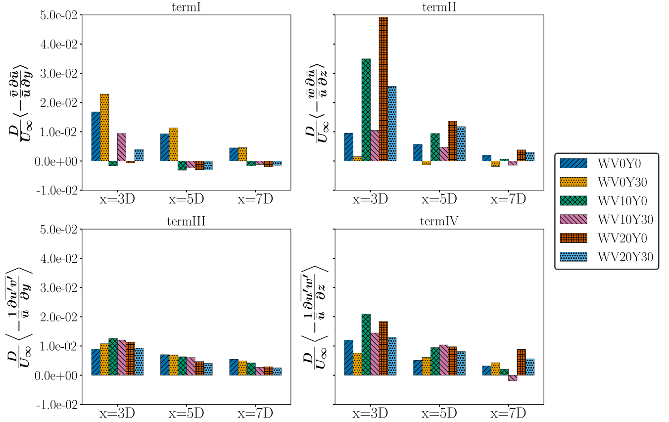
Figure 14. Terms of streamwise momentum budget equation 8 integrated over the wake region defined as where Ux/U_\infty = 0.9 . Each term is shown at three different cross-stream locations x/D = 3, 5 , and, 7 for three different inflows and yaw angles of 0^\circ and 30^\circ .
