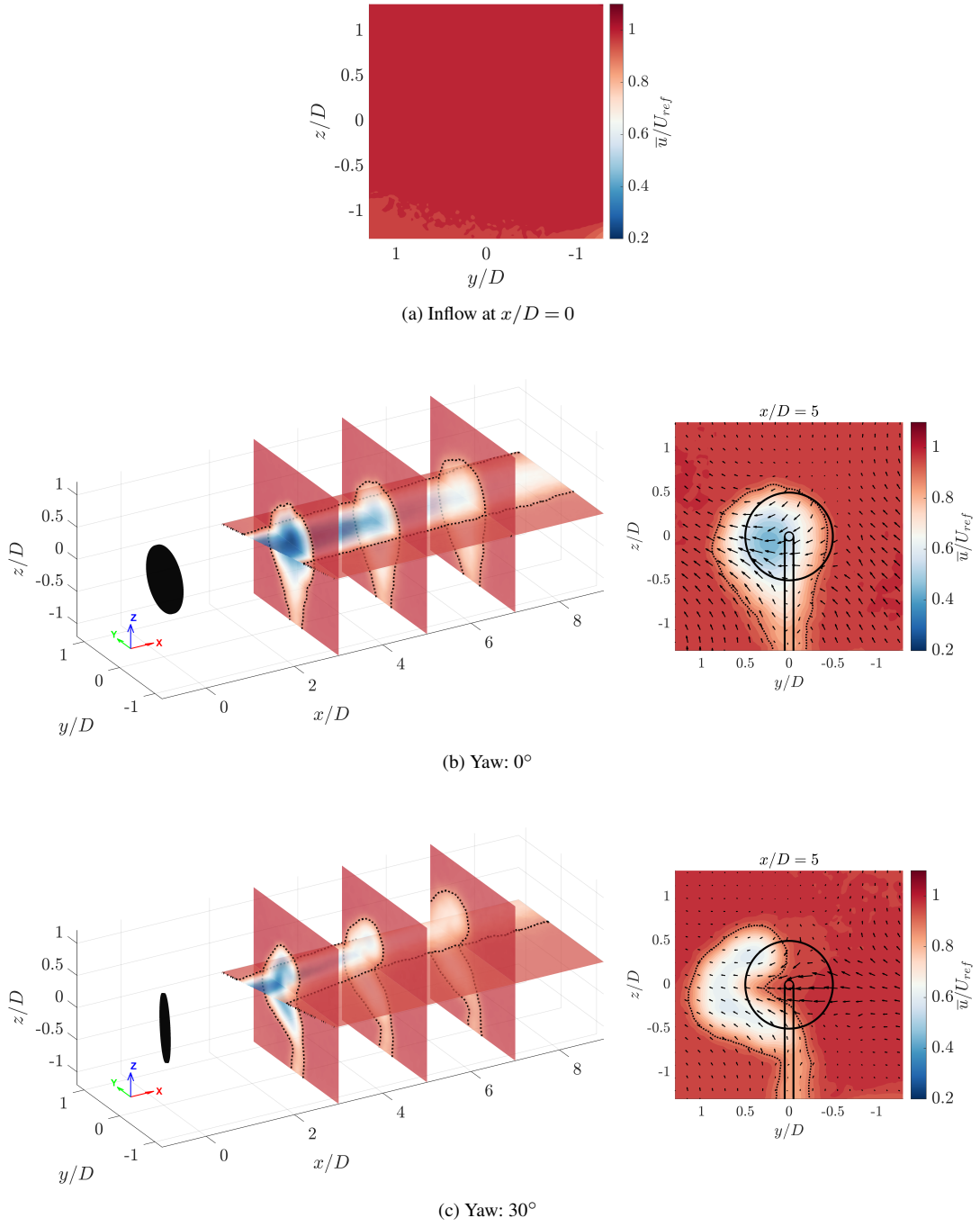
Figure 5. Normalized streamwise velocity wake contours for the uniform inflow case for yaw angles of 0^\circ and 30^\circ . For reference, the inflow at the disc location ( x/D = 0 ) is shown in the top panel. The middle and the bottom panels present combined cross-sectional planes overlaid on the streamwise plane for the yaw angles of 0^\circ and 30^\circ , respectively. The streamwise velocity contour at the cross-stream location x/D = 5 is also included, with quivers indicating the in-plane velocity vectors. The solid circle represents the disc span, while the yawed disc is shown by a dashed line. The dotted black line depicts the wake boundary, defined as the contour where \bar{u}/U_\infty = 0.9 .
