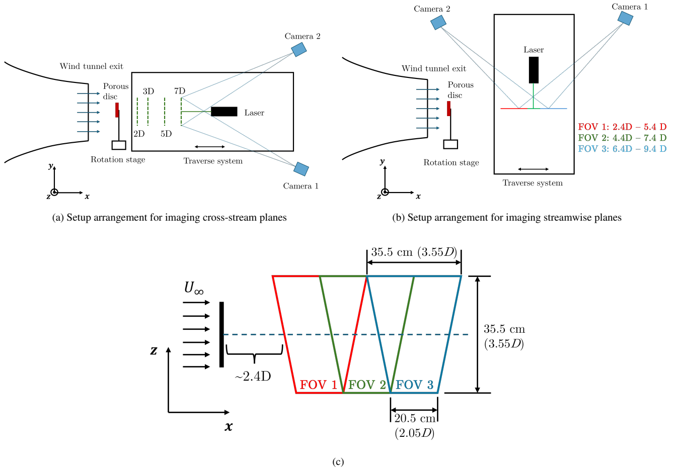
Figure 1. Top view of the SPIV experimental setup for imaging (a) cross-stream planes ( yz - planes ) and (b) streamwise planes ( xz ). The cross-stream positions where measurements are taken are indicated by green dashed lines in Fig. 1a. In total, measurements were performed at four cross-stream planes ( x/D = 2, 3, 5, \text{ and } 7 ). Measurements-Streamwise measurements were also performed in the horizontal-plane xz -plane to capture wake evolution , and the imaging locations-planes are indicated by the solid-red , green, and blue lines, with some overlap between consecutive planes lines. The laser sheet is coming out of the plane in both figures. (c) The dimensions of the field of view (FOV) are indicated here. For streamwise FOVs, an overlap of 1D is applied at the center of the trapezoid. A Gaussian function is applied to stitch the streamwise FOVs. It should be noted that the dimensions of the FOV remain the same for both cross-stream and streamwise measurements.
