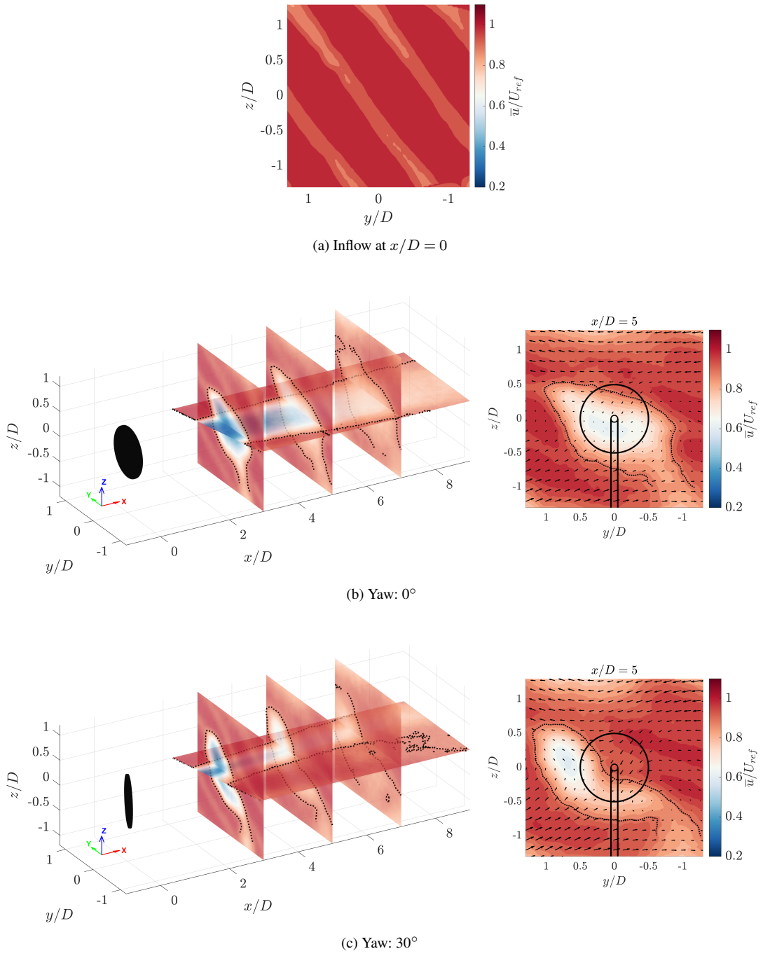
Figure 6. Normalized streamwise velocity wake contours for the veered inflow case with a 10^\circ veer. The rest of the caption is the same as Fig. 5.
