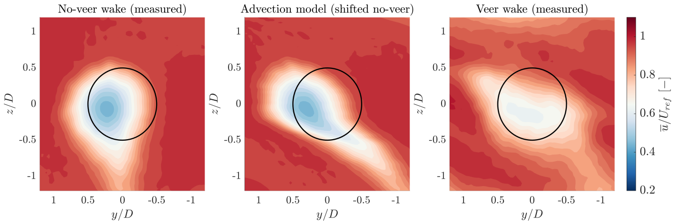
Figure C1. Comparison of a simple model advection with the experimental results of veer wake at x/D = 5 . The leftmost plot corresponds to the case of WV0Y0, the middle plot is obtained from the simple advection model, and the rightmost plot is the measured case of WV10Y0.
