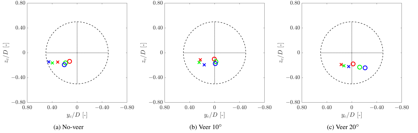
Figure 8. Wake center for three inflow cases corresponding to yaw angles of 0^\circ (represented as circles) and 30^\circ (represented as crosses). The red, green, and blue colors represent the cross-stream plane location ( x/D ) of 3, 5, and 7, respectively.
