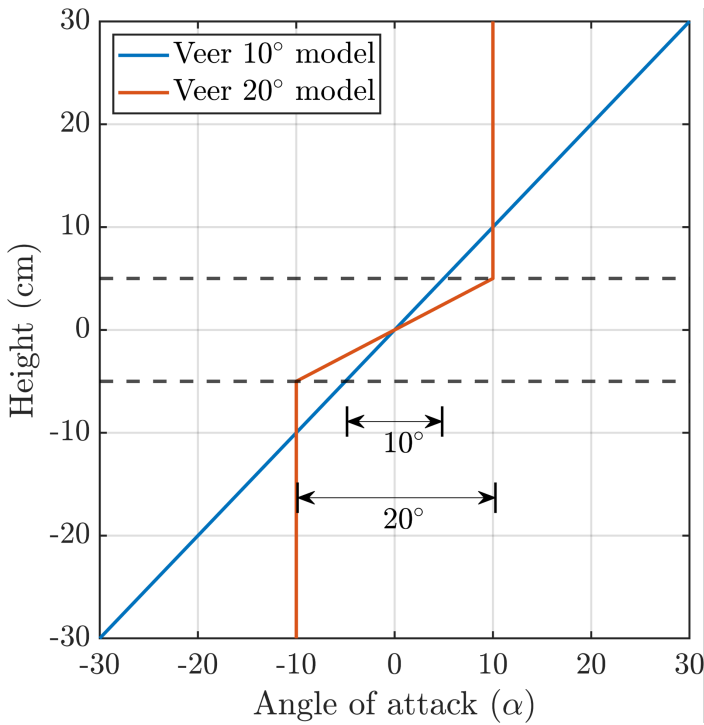
Figure 3. (Left figure) Variation of angle of attack of the NACA airfoil for wind veer model of 10^\circ (blue line) and 20^\circ (red line). The dashed horizontal line represents the top and bottom extent of the disc, such that a total of 10^\circ and 20^\circ veer is generated from the two models, respectively; (Right figure) Wind-Different views of the wind veer model for generating a veer of 10^\circ across the porous disc-installed at the exit of the wind tunnel. The leading-edge portion of the model is located inside the wind tunnel, while the trailing-edge portion extends outside. A similar model that generates a wind veer of 20^\circ (not shown here) is also tested.
