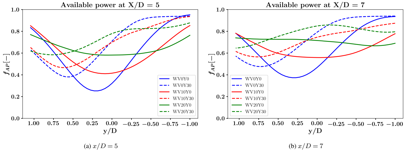
Figure 17. Coefficient of available power as calculated using Eq. 11 at two downstream locations (a) x/D = 5 and (b) x/D = 7 for different cases. The legend notation is WV\phi Y\theta , where \phi denotes the wind veer angle (in degrees) and \theta denotes the yaw angle (in degrees). For example, WV10Y30 corresponds to a 10^\circ wind veer inflow and a 30^\circ yaw misalignment of the disc.
