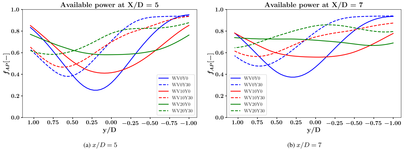
Figure 17. Coefficient of available power as calculated using Eq. 11 at two downstream locations (a) x/D = 5 and (b) x/D = 7 for different yaw and veering cases.
