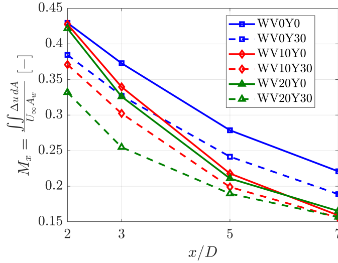
Figure 9. Integral analysis of wake deficit in the wake area for all three inflow conditions and yaw angles of 0^\circ and 30^\circ . The legend notation is WV \phi Y \theta , where \phi denotes the wind veer angle (in degrees) and \theta denotes the yaw angle (in degrees). For example, WV10Y30 corresponds to a 10^\circ wind veer inflow and a 30^\circ yaw misalignment of the disc.
