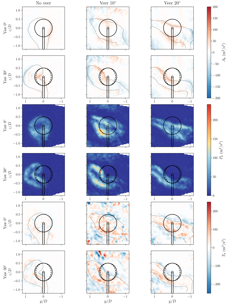
Figure 16. Spatial distribution of terms in Eq. 10 at x/D = 5 . The solid circle represents the frontal projection of the unyawed porous disc, whereas the dashed circle represents the yawed disc of 30^\circ . The dotted line indicates the wake boundary where u/U_{ref} = 0.9 .
