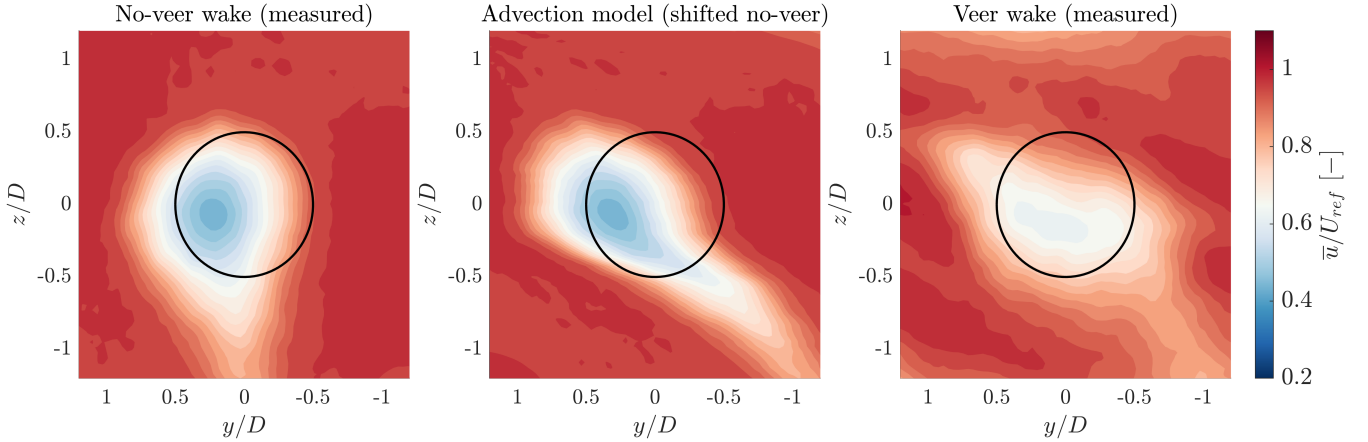
Figure C1. Comparison of a simple model advection with the experimental results of veer wake at x/D = 5 . The leftmost plot corresponds to the case of WV0Y0, the middle plot is obtained from the simple advection model, and the rightmost plot is the measured case of WV10Y0.
