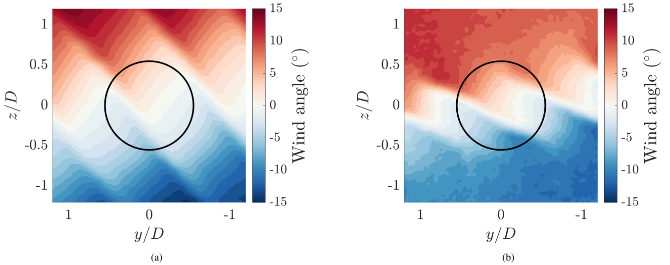
Figure 19. Flow characterization contours of variation of wind veer in the yz -plane at x/D = 0 (a) Veer 10^\circ ; (b) Veer 20^\circ . The solid circle represents the frontal projection of the porous disc.
