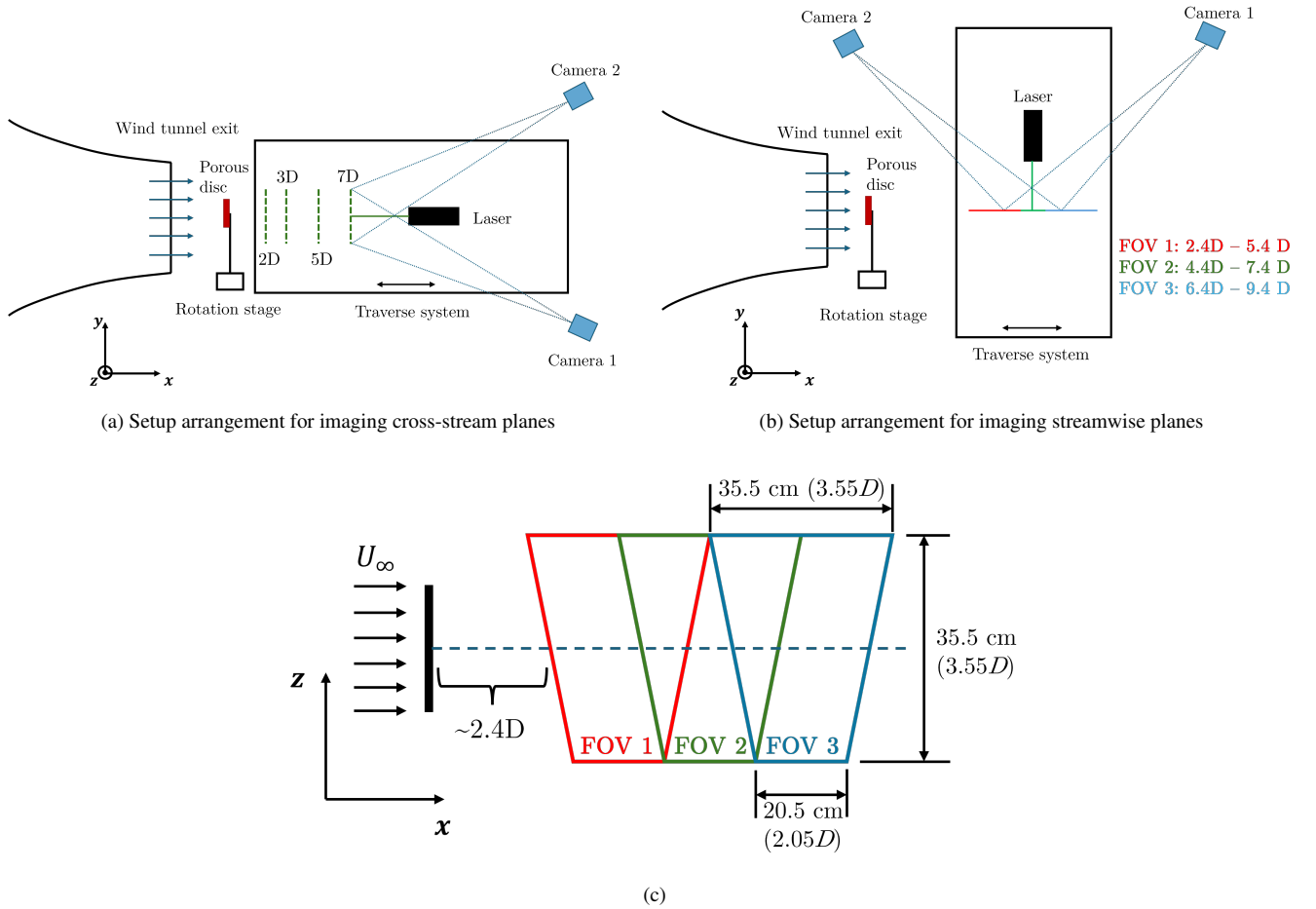
Figure 1. Top view of the SPIV experimental setup for imaging (a) cross-stream planes ( yz ) and (b) streamwise planes ( xz ). The cross-stream positions where measurements are taken are indicated by green dashed lines in Fig. 1a. In total, measurements were performed at four cross-stream planes ( x/D = 2, 3, 5 , and 7 ). Streamwise measurements were also performed in the xz -plane to capture wake evolution, and the imaging planes are indicated by the red, green, and blue lines, with some overlap between consecutive lines. The laser sheet is coming out of the plane in both figures. (c) The dimensions of the field of view (FOV) are indicated here. For streamwise FOVs, an overlap of 1D is applied at the center of the trapezoid. A Gaussian function is applied to stitch the streamwise FOVs. It should be noted that the dimensions of the FOV remain the same for both cross-stream and streamwise measurements.
