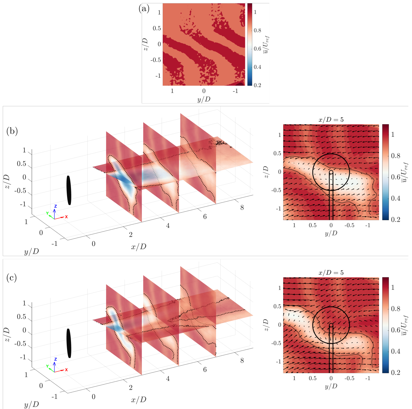
Figure 7. Normalized streamwise velocity wake contours for the veered inflow case with a 20^\circ veer. The rest of the caption is the same as Fig. 5.
