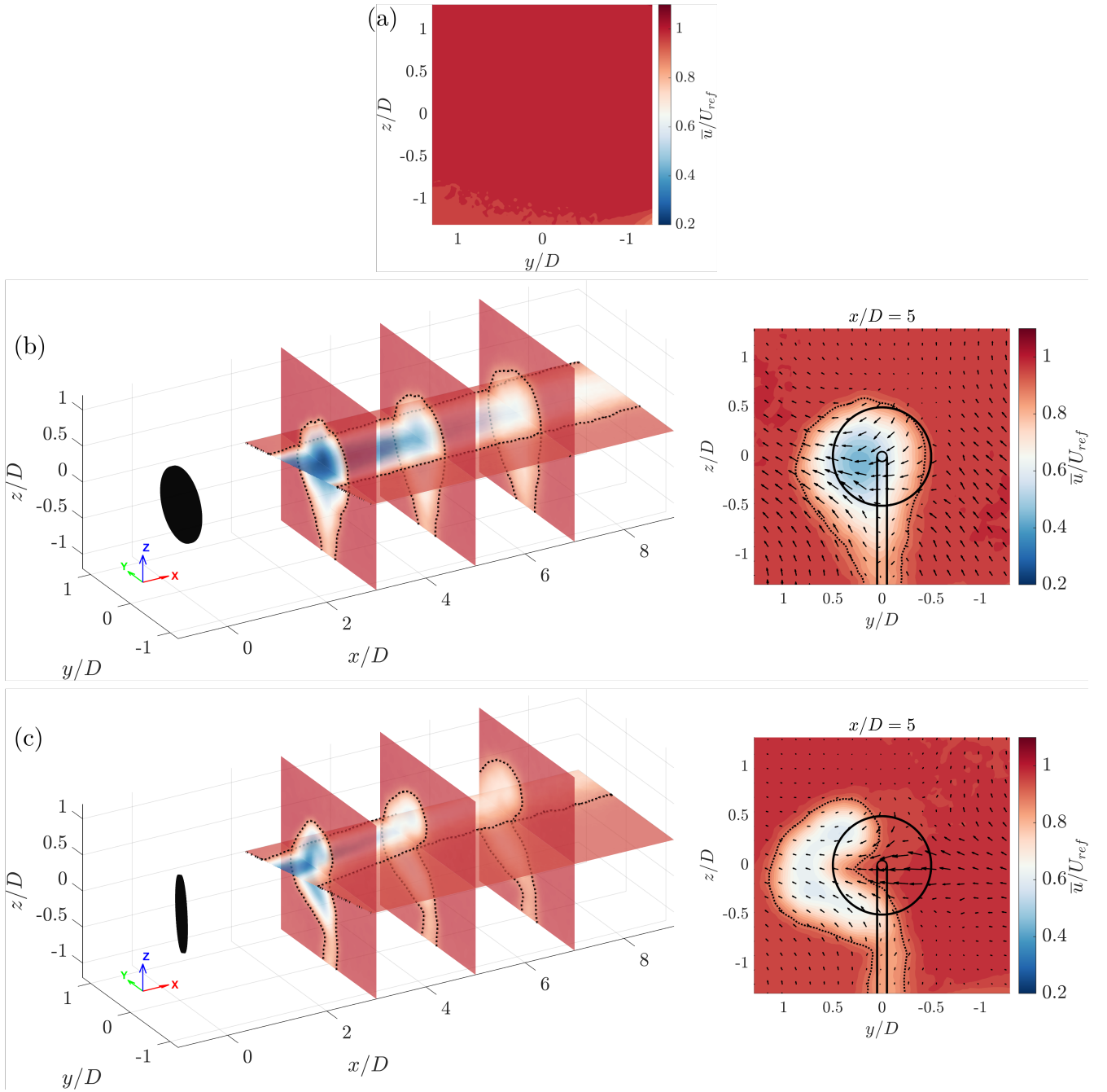
Figure 5. Normalized streamwise velocity wake contours for the uniform inflow case for yaw angles of 0^\circ and 30^\circ . (a) Inflow at the disc location ( x/D = 0 ), shown for reference. (b,c) Combined cross-sectional planes overlaid on the streamwise plane for the yaw angles of 0^\circ and 30^\circ , respectively. The streamwise velocity contour at the cross-stream location x/D = 5 is also included, with quivers indicating the in-plane velocity vectors. The solid circle represents the disc span. The dotted black line depicts the wake boundary, defined as the contour where \bar{u}/U_\infty = 0.9 .
