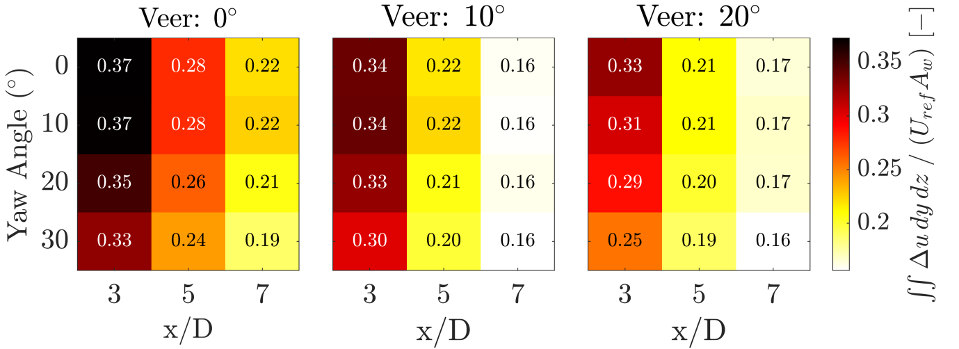
Figure 10. Integrated velocity deficit heat map under yaw angles of 0^\circ , 10^\circ , 20^\circ , and 30^\circ under all three inflow conditions at different downstream cross-sectional planes of x/D = 3, 5 , and 7 .
