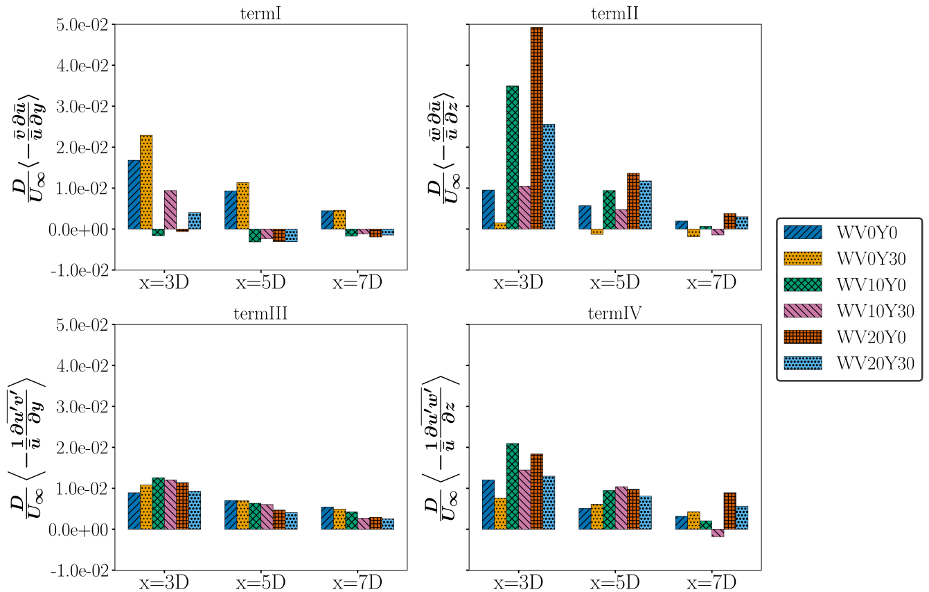
Figure 14. Terms of streamwise momentum budget equation 8 integrated over the wake region defined as where u/U_\infty = 0.9 . Each term is shown at three different cross-stream locations x/D = 3, 5 , and 7 for three different inflows and yaw angles of 0^\circ and 30^\circ .
