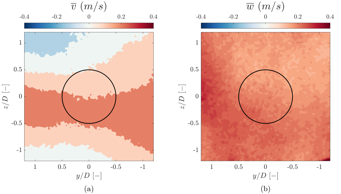
Figure A1. Flow characterization contours in the yz -plane for the clean case in the absence of the porous disc at x/D = 0 : (a) Spanwise velocity; (b) Vertical velocity. The solid circle represents the frontal projection of the disc.
