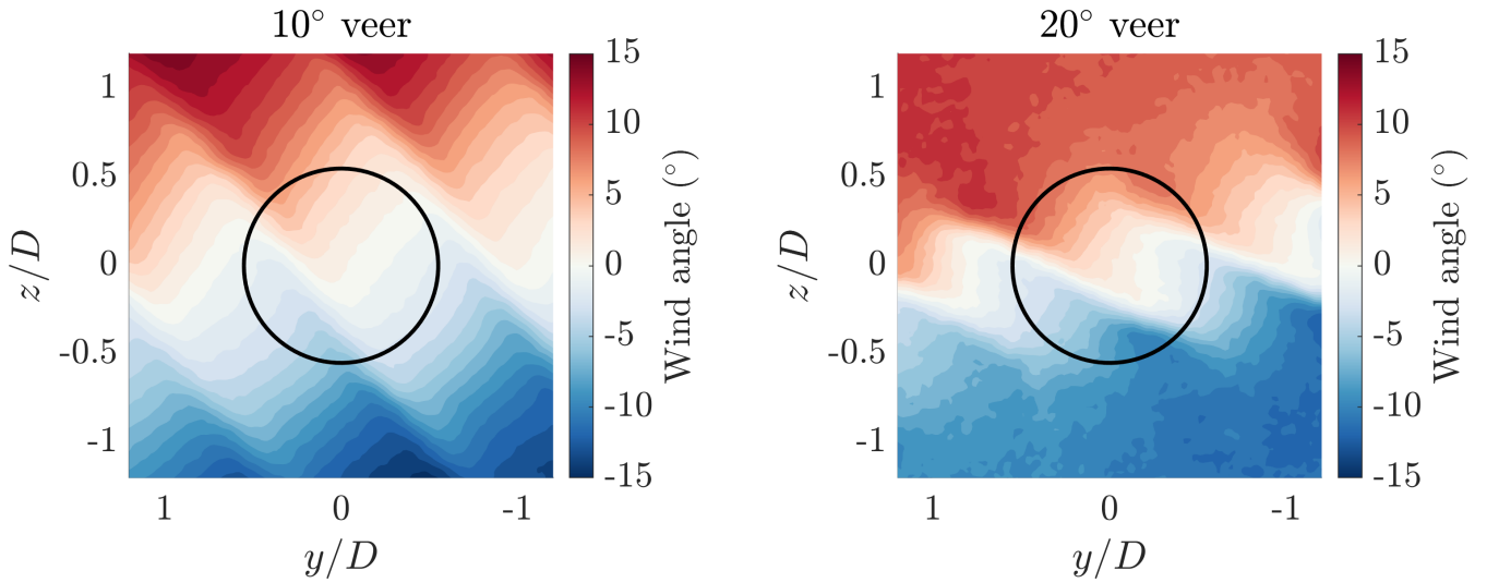
Figure 19. Flow characterization contours of variation of wind veer in the yz -plane at x/D = 0 for the 10^\circ (left) and 20^\circ (right) veer cases. The solid circle represents the frontal projection of the porous disc.
