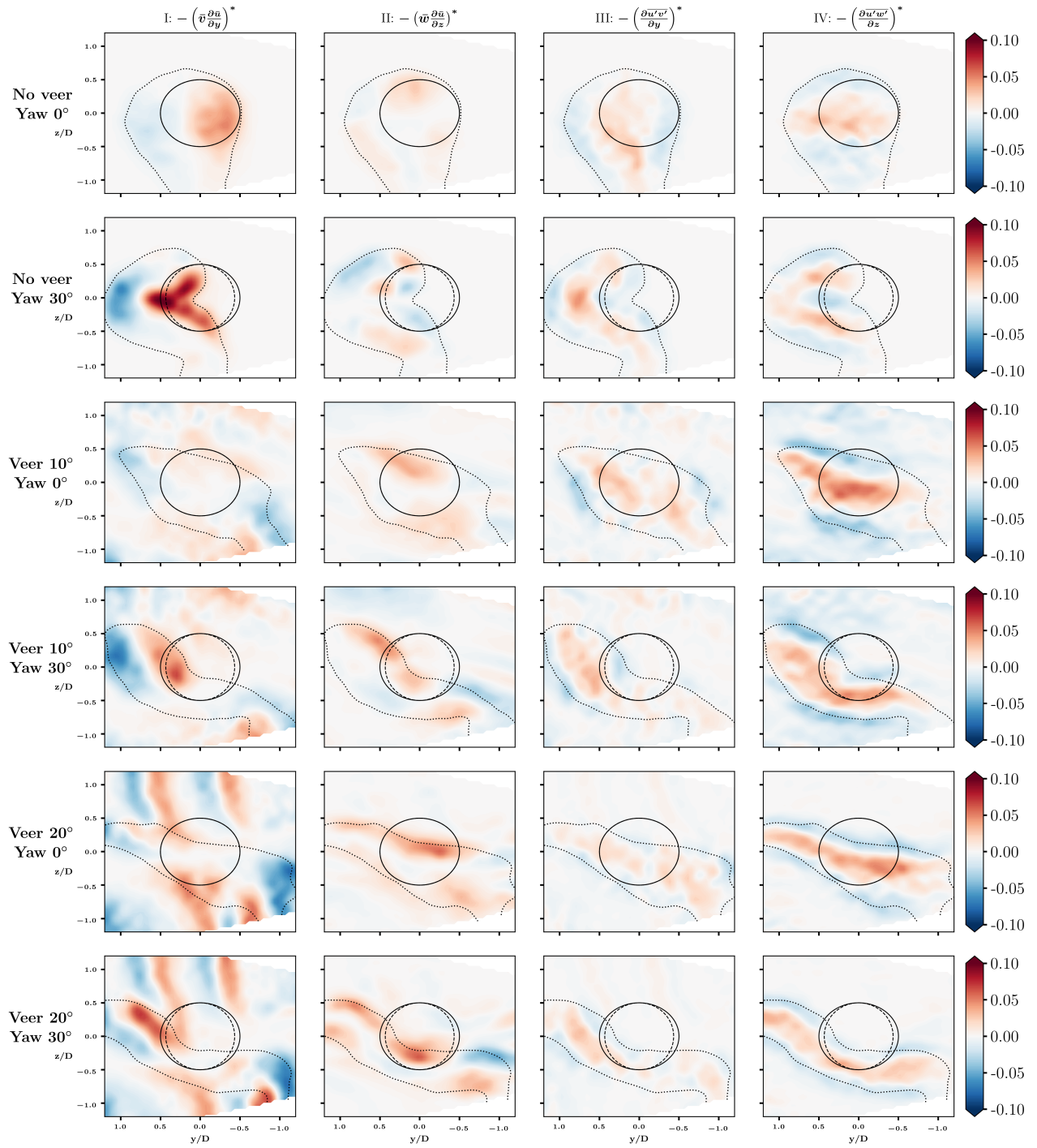
Figure 13. Measured terms of Eq 7 at X/D = 5 . The disc projection is represented by a solid circle, whereas the projection of the yawed disc is shown as a dashed line. The wake contour is shown as a dotted line where U_x/U_\infty = 0.9 . The asterisk indicates that each term is normalized by the factor D/U_\infty^2 .
