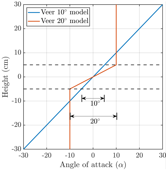
Figure 3. (Left figure) Variation of angle of attack of the NACA airfoil for wind veer model of 10^\circ (blue line) and 20^\circ (orange line). The dashed horizontal line represents the top and bottom extent of the disc, such that a total of 10^\circ and 20^\circ veer is generated from the two models, respectively; (Right figure) Different views of the wind veer model for generating a veer of 10^\circ installed at the exit of the wind tunnel. The leading-edge portion of the model is located inside the wind tunnel, while the trailing-edge portion extends outside. A similar model that generates a wind veer of 20^\circ (not shown here) is also tested.
