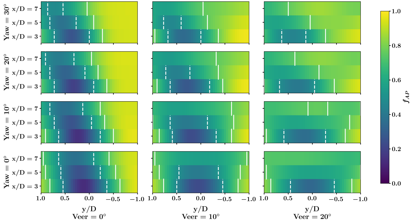
Figure 18. Filled contour of available power distribution (Eq. 11) for all cases at three downstream locations. f_{AP} is computed by integrating U^3 over the frontal projection area of the porous disc centered at y/D and normalizing by the corresponding integral of the inflow U_{in}^3 over the same area. The disc projection is then traversed laterally across the wake to produce the distributions shown. The solid vertical line represents the locations where f_{AP} is 0.75 and the dashed vertical line represents locations where f_{AP} is 0.5.
