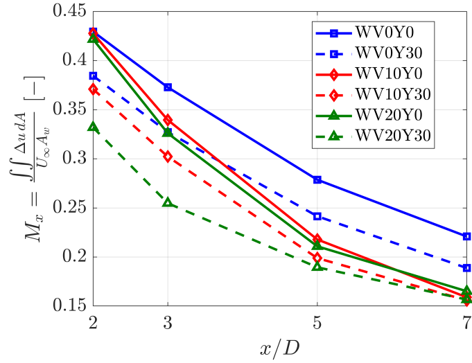
Figure 9. Integral analysis of wake deficit in the wake area for all three inflow conditions and yaw angles of 0^\circ and 30^\circ . The legend notation is WV\phi Y\theta , where \phi denotes the wind veer angle (in degrees) and \theta denotes the yaw angle (in degrees). For example, WV10Y30 corresponds to a 10^\circ wind veer inflow and a 30^\circ yaw misalignment of the disc.
