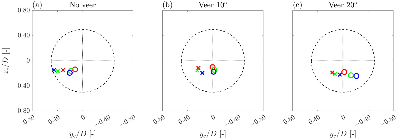
Figure 8. Wake centers for three inflow cases: (a) no veer, (b) 10^\circ veer, and (c) 20^\circ veer, each at yaw angles of 0^\circ (circles) and 30^\circ (crosses). Red, green, and blue denote the streamwise location x/D of the cross-stream plane at 3, 5, and 7, respectively. The dashed circle indicates the projection of the porous disc, and the dotted lines mark the hub height and disc axis. Coordinates are normalized by the disc diameter D .
