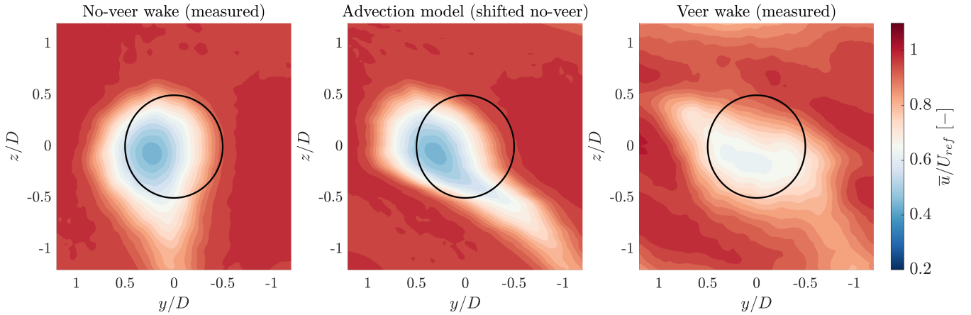
Figure C1. Comparison of a simple advection model with the experimental results of veer wake at x/D = 5 . The leftmost plot corresponds to the case of WV0Y0, the middle plot is obtained from the simple advection model, and the rightmost plot is the measured case of WV10Y0.
