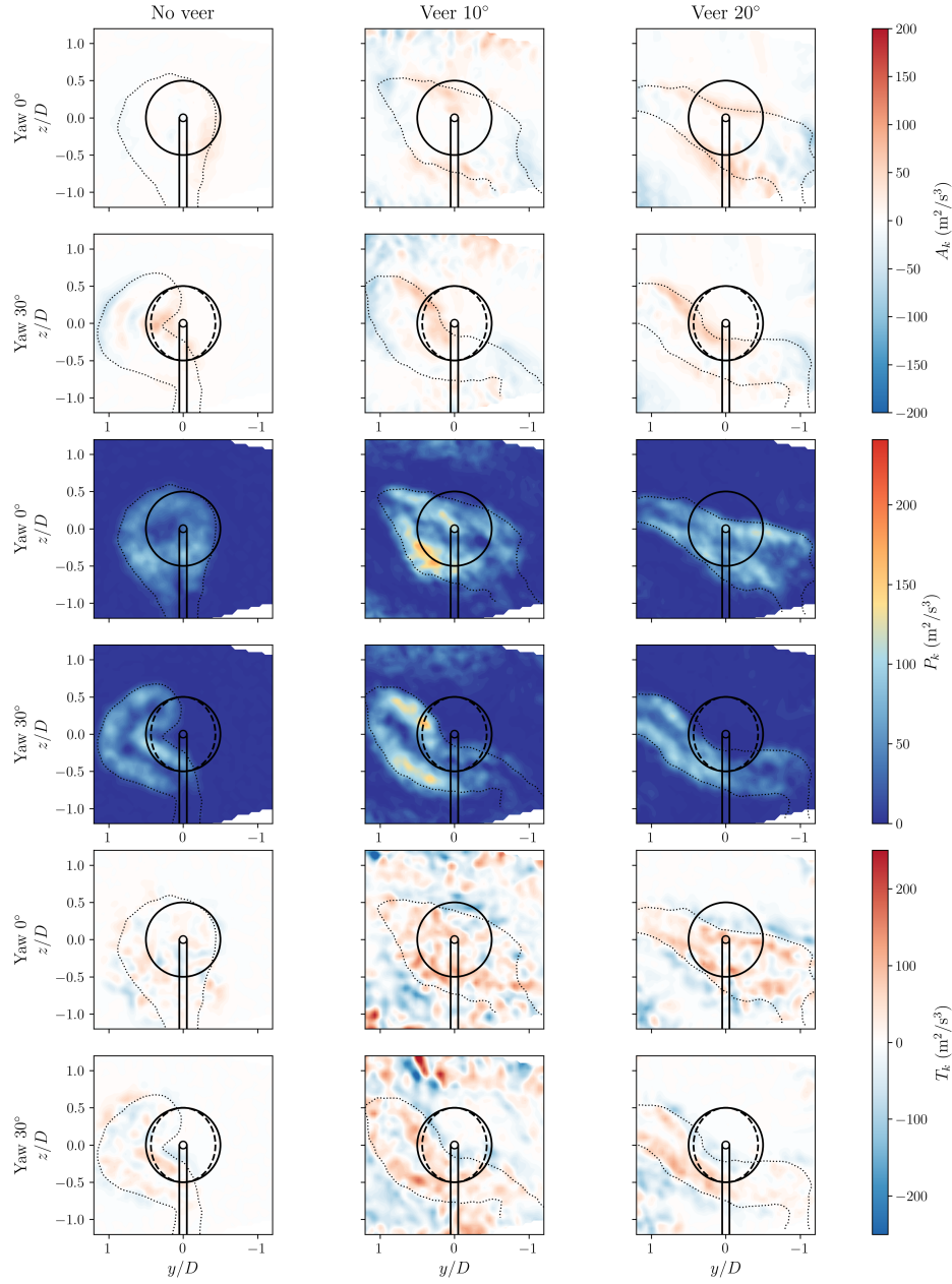
Figure 16. Spatial distribution of terms in Eq. 10 at x/D = 5 . The solid circle represents the frontal projection of the non-yawed porous disc, whereas the dashed circle represents the yawed disc of 30^\circ . The dotted line indicates the wake boundary where u/U_\infty = 0.9 .
