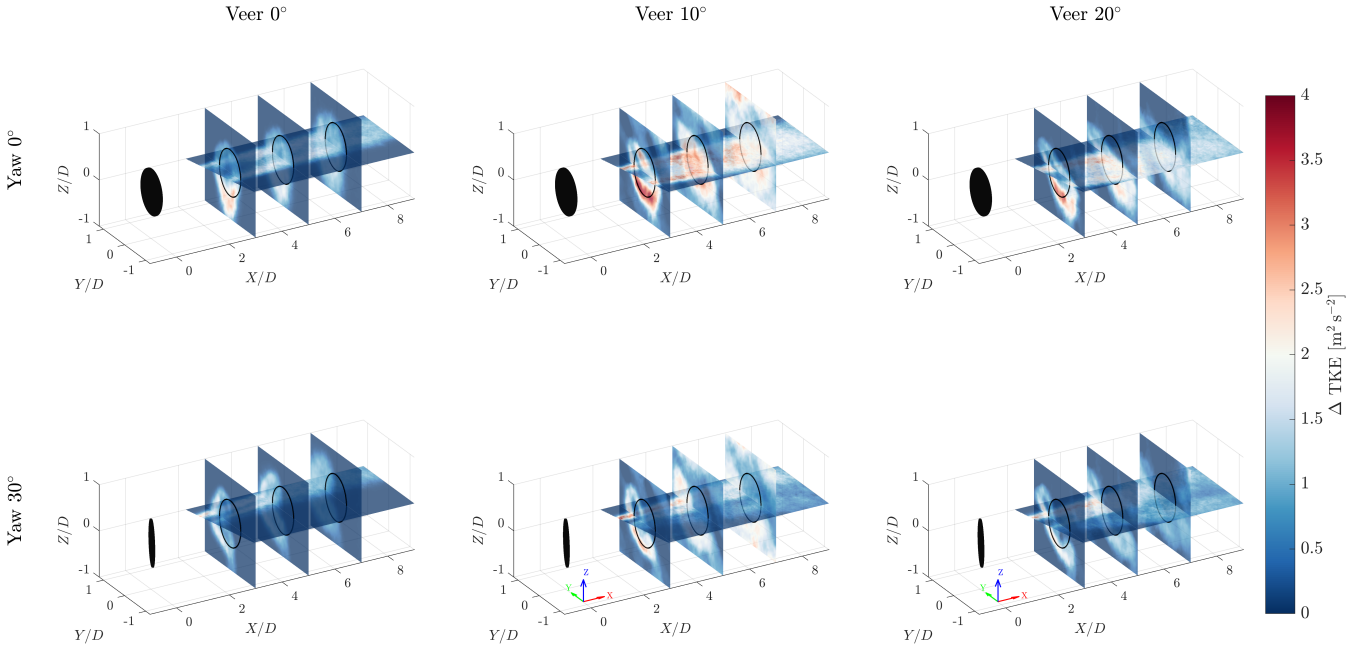
Figure 15. Distribution of wake-added turbulent kinetic energy for the three different inflows. The figures on the left correspond to the no-veer inflow, the middle figures to the 10° veer inflow, and the right figures to the 20° veer inflow. The figures in the top panel are for the yaw angle of 0°, whereas the figures in the bottom panel are for the yaw angle of 30°. The solid circle on the cross-stream plane represents the projection of the non-yawed disc.
