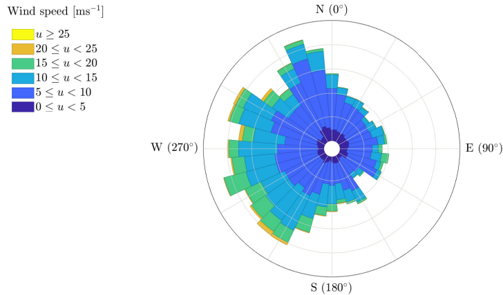
Figure 3. Polar plot showing the 10-min mean nacelle positions of all the front-row turbines in A/HS from 10-01-2021 till 17-03-2022. The plot differs slightly from the ten year mean wind rose (not shown here) due to the period of analysis.
