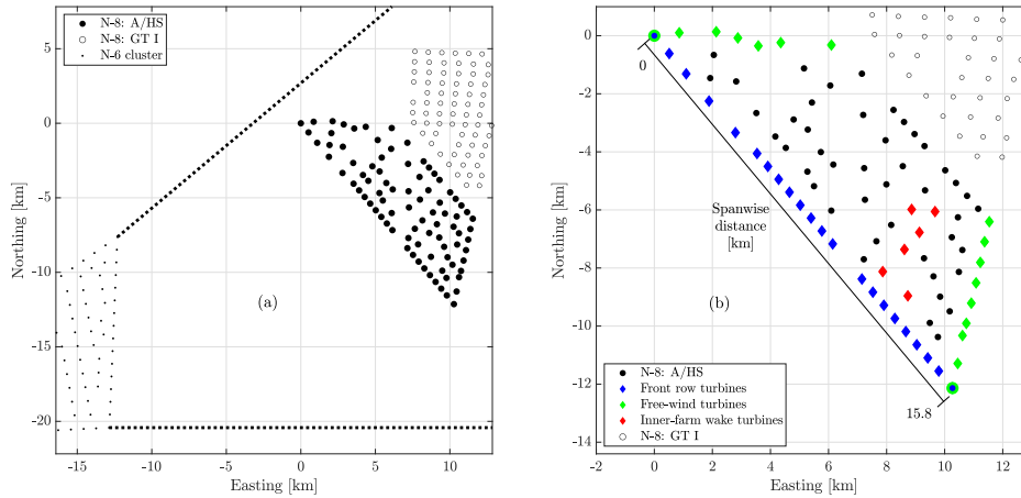
Figure 2. (a) Region of the N-6 cluster (dots) and the N-8 cluster (filled and empty circles). The wind direction sector considered for N-6 cluster wake analysis spanning from 230^\circ to 270^\circ is indicated by dashed lines. (b) A/HS wind farm in the N-8 cluster with highlighted turbines for analysis: front-row turbines to the southwest (blue diamonds), reference turbines in free inflow (green diamonds) and turbines in inner-farm wake conditions (red diamonds). The origin of the coordinate system is the front-row turbine in the northwestern corner. The span-wise distance along the front row of turbines is also indicated, starting from the north east corner at [0,0] until the turbine at the southern corner, 15.8 km away from it.
