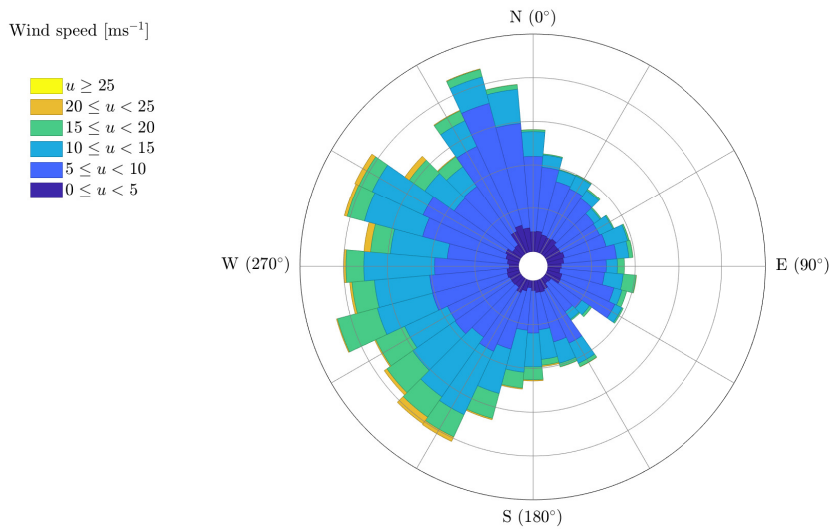
Figure 3. Polar plot showing the 10-min mean nacelle positions of all the turbines in A/HS from 10-01-2021 till 17-03-2022. The plot differs slightly from the ten year mean wind rose (not shown here) due to the period of analysis.
