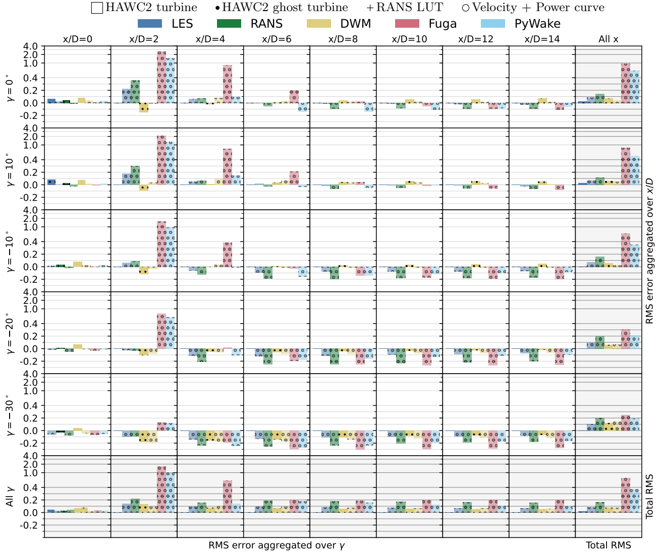
Figure 6. Relative power error \epsilon = (P - P_{\text{LES}})/P_{\text{LES}} compared to LES for the first turbine as well as for several ghost turbines placed at different downstream locations in the wake. For the first turbine, results for a real turbine with coupling to the inflow are shown using untextured bars (indicated by an empty square in the legend) for the HAWC2 turbine in the LES/DWM simulations and a plus symbol for the corresponding RANS LUT result; these data are only available for the first row, as the remaining turbines are ghost turbines. Consequently, for the first turbine the LES reference is a HAWC2 turbine, whereas HAWC2 ghost turbines are used as the LES reference for the waked turbines. Results for all yaw angles and models are shown. The aggregated error is given by \epsilon_{\text{RMS}} = \sum \sqrt{\epsilon^2} . A symlog scale is used on the y-axis, such that values with |\epsilon| < 0.5 are shown on a linear scale and larger values on a logarithmic scale.
