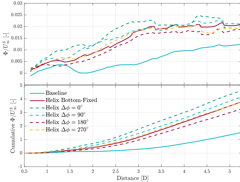
Figure 7. Local (top) and cumulative (bottom) results of the energy entrainment analysis using the phase-averaged measurement data. The flux \Phi has been normalized using the freestream inflow velocity U_\infty .
