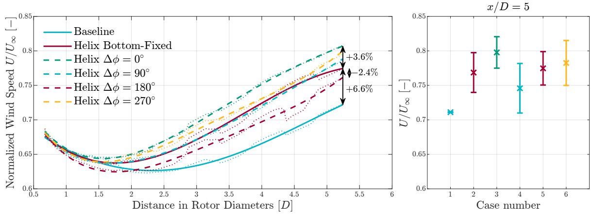
Figure 5. Rotor-average wind speed as perceived by a hypothetical downstream turbine in the wake. The thin dotted lines show the results as measured per individual measurement domain. This data is approximated using fourth-order polynomials (thick lines), removing the jumps in data between individual measurements. The solid lines represent the results without yaw motion, and the dashed lines represent the results when the turbine is undergoing yaw motion. The right-hand side of the figure shows the mean wind speed for each case at a distance of 5D . The error bars indicate the standard deviation of the rotor-averaged wind speed over a single Helix cycle.
