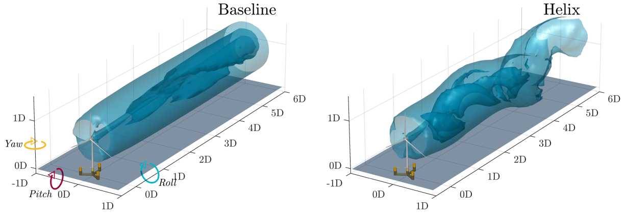
Figure 1. Model of the IEA 15MW turbine mounted on the VoltturnUS-S floater, with the left figure showing the wake when using a baseline controller, and on the right figure the distorted wake when the Helix method is enabled. The visualised wakes feature iso-surfaces of the streamwise velocity taken from large eddy simulation results by Frederik et al. (2020b).
