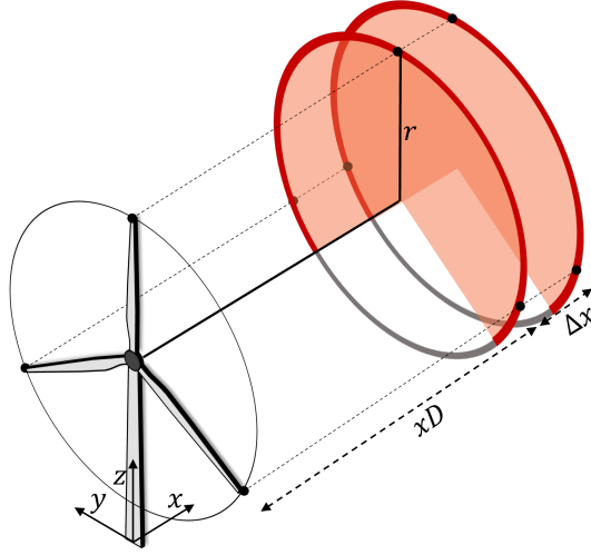
Figure 6. Schematics of the entrainment calculation in the radial direction over a control volume. We consider a ring (bright red) of radius r located a distance of xD from the turbine, over which the mean flux of kinetic energy is calculated per downstream distance \Delta x . The Cartesian velocity components are first transformed to a cylindrical coordinate frame.
