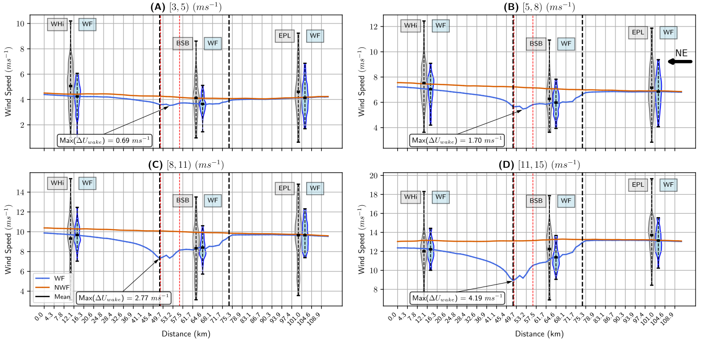
Figure 13. WRF-assessed hub-height wind speed along the WHi, BSB, and EPL transect for NE wind directions, with wind direction calculated as the mean across the three lidar sites. Vertical lines mark the Belgian-Dutch cluster (black) and the Belgian-only wind-farm areas (red). The wind speed range on the y-axis varies across classes to highlight class-specific distributions, and the maximum wind speed deficit value within the Belgian-Dutch zone is depicted.
