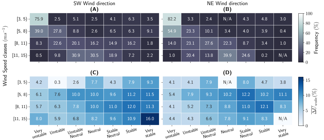
Figure 14. Frequency of the ABL stability conditions for each wind speed regime, under SW (A), and NE (B) wind directions. Averaged wake magnitude under the different ABL conditions and wind speed classes for SW (C) and NE (D) wind directions.
