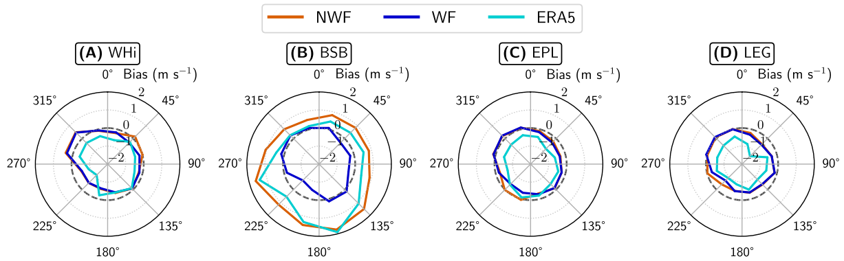
Figure 7. Wind speed bias under different wind direction sectors, evaluated against lidar observations. All values are interpolated to hub height. The deviation from the black dashed line indicates the degree of misalignment with the observations.
