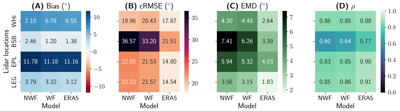
Figure 6. Evaluation metrics for wind directions against lidar data: Bias (A), cRMSE (B), EMD (C), and r (D) scores. All values are interpolated to hub height. Darker colors signify poorer alignment with the observations.
