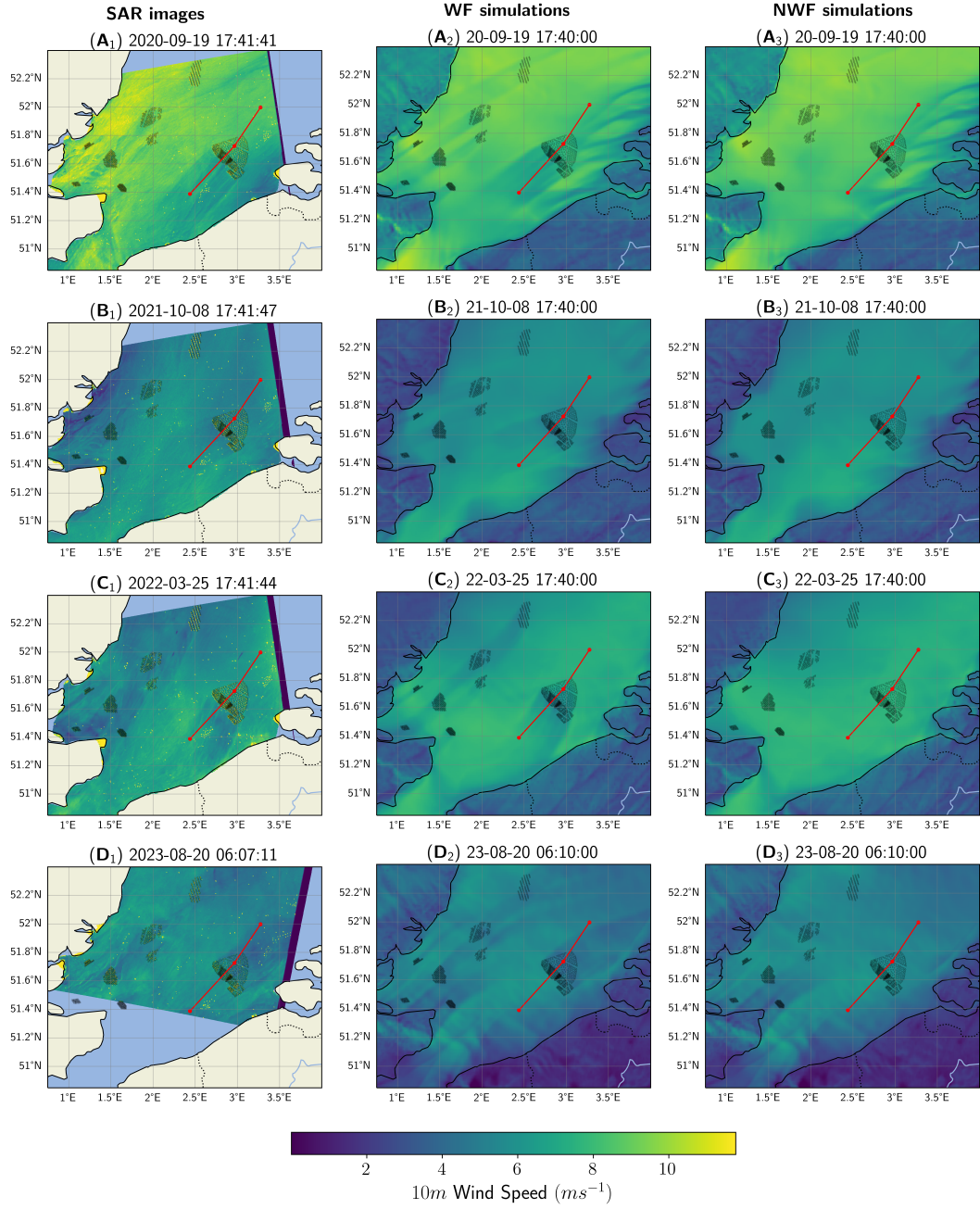
Figure 16. Two-dimensional wind speeds at 10-meter height: SAR images (left, subscript 1), WF simulations (middle, subscript 2), and NWF simulations (right, subscript 3). Four snapshots are compared where the wind farm-produced wake is present. The red line depicts the transect connecting the WHi, BSB, and EPL locations.
