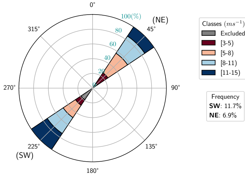
Figure 11. Frequency of the wind speed classes under SW (11.7%) and NE (6.9%) wind directions, respectively. The frequency is calculated on the common timestamps of the lidars and not over the full period of analysis.
