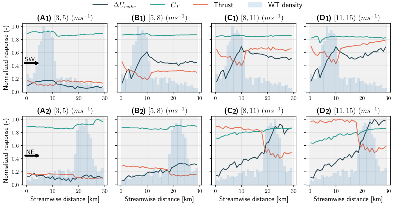
Figure 17. Streamwise-averaged and normalized \Delta U_{wake} , C_T , and thrust computed based on Equation (5). The shaded grayed area extending to about 28 kilometers represents the length of the Belgian-Dutch cluster, while the light blue bins depict the streamwise-averaged wind turbine density. The top row shows cases with SW wind direction, and the bottom row corresponds to NE wind direction, respectively.
