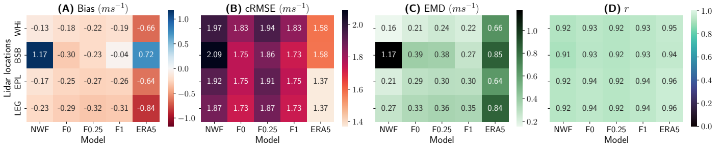
Figure A1. Evaluation of hub height wind speed from four different WRF runs and ERA5 data at four lidar Locations: Bias (A), cRMSE (B), EMD (C), and r (D) scores.
