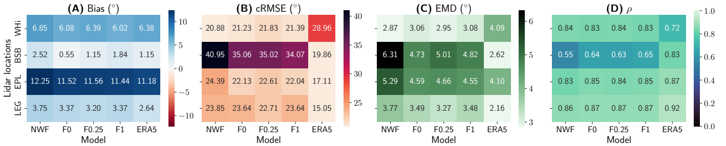
Figure A2. Evaluation of hub height wind directions from four different WRF runs and ERA5 data at four lidar Locations: Bias (A), cRMSE (B), EMD (C), and r (D) scores.
