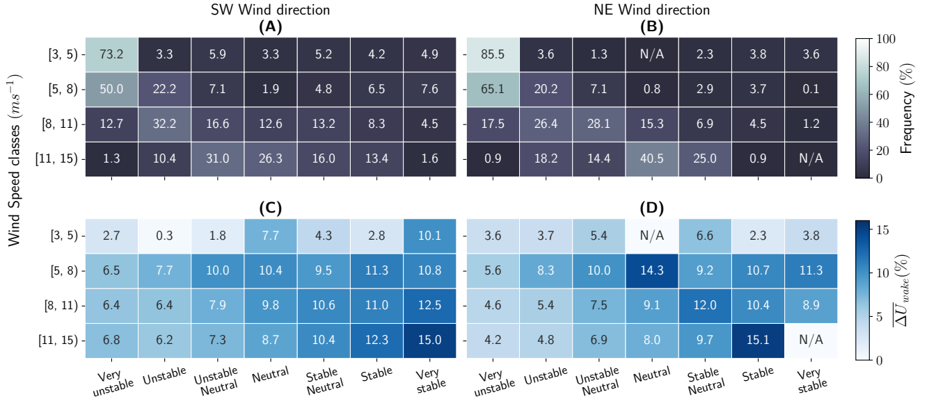
Figure 14. Frequency of the ABL stability conditions for each wind speed regime, under SW (A), and NE (B) wind directions. The stability regimes based on L are computed as the average of the WHi, BSB, and EPL from the NWF simulations. Plots (C) and (D) show the averaged wake magnitude across the three locations for different ABL conditions and wind speed classes under SW and NE wind directions, respectively.
