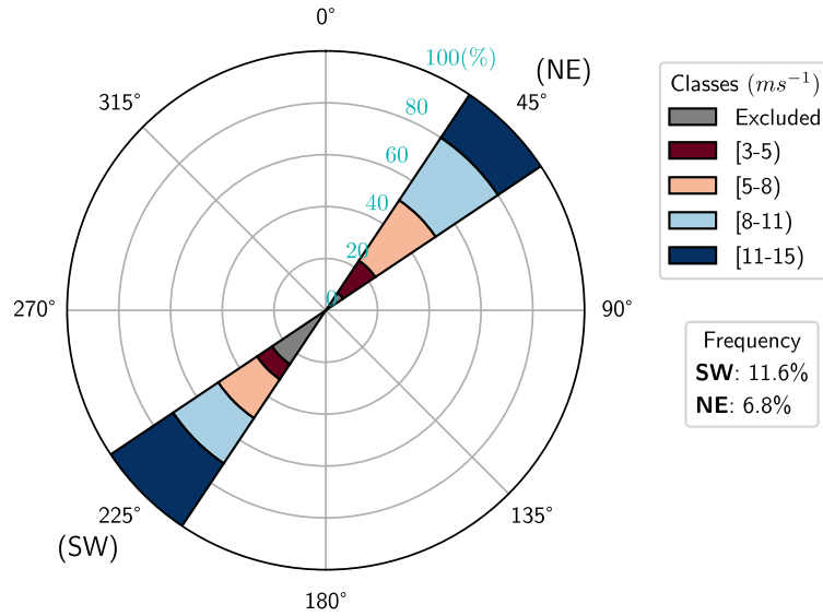
Figure 11. Frequency of the wind speed classes under SW (11.6%) and NE (6.8%) wind directions, respectively. The frequency is calculated on the common timestamps of the lidars and not over the full period of analysis.
