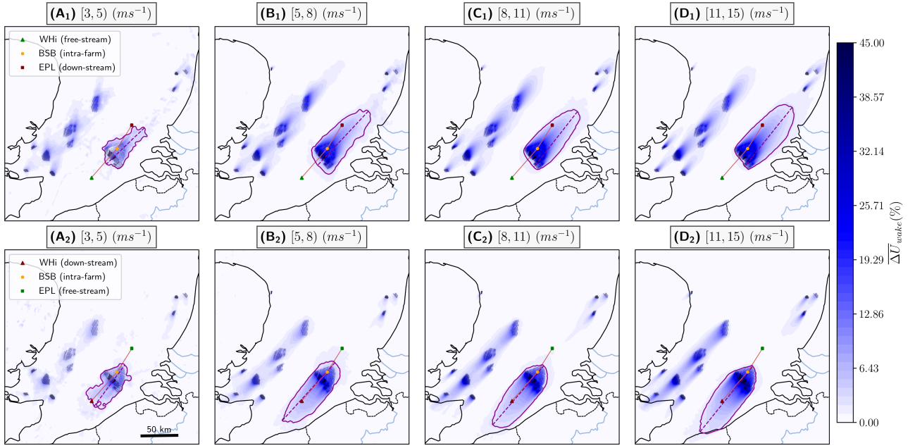
Figure 15. Wind speed deficits calculated at the hub height under the four wind speed regimes. The orange line illustrates the WHi, BSB, and EPL transect. Subscript 1 indicates that wind direction is SW (top), and subscript 2 denotes NE wind direction conditions (bottom). Wind speed deficits are averaged across each wind speed class. Solid purple lines depict the 5% wind speed deficit, and dashed purple lines the maximum wake length within this area.
