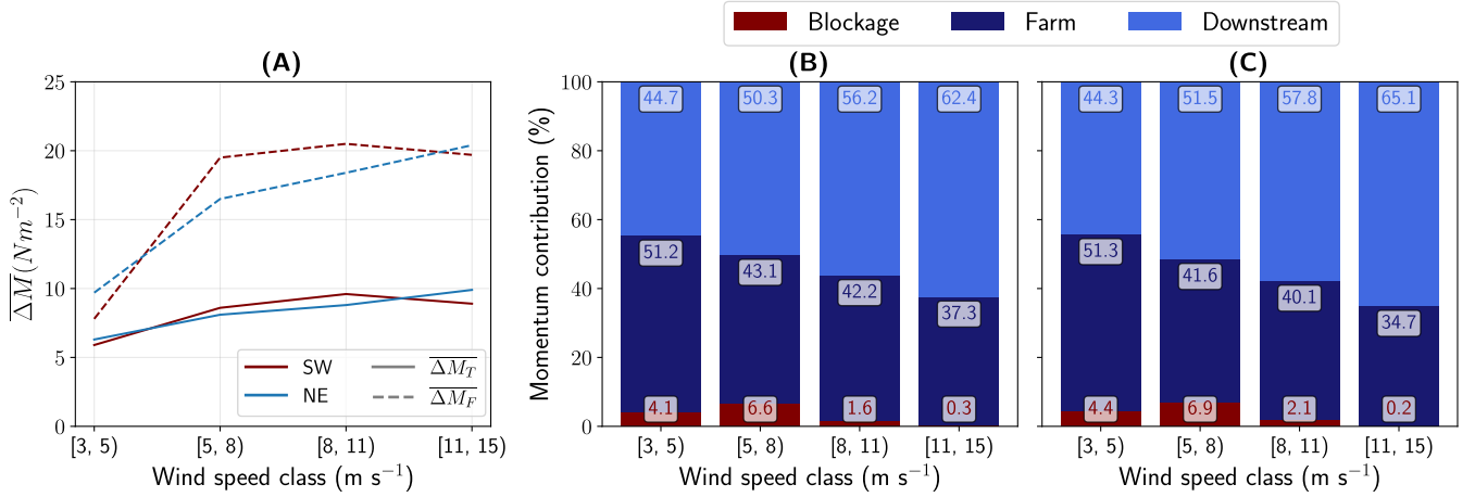
Figure 16. (A) Momentum flux deficits across the total 5% wind speed deficit region ( \overline{\Delta M_T} ) and the Belgian-Dutch cluster area ( \overline{\Delta M_F} ). Momentum flux deficit fractions within the 5% wind speed deficit area under SW (B) and NE (C) wind directions across different wind speed regimes. The farm area is the only source of momentum due to the Fitch WFP scheme. The contributions of blockage, farm (i.e., momentum extraction), and downstream momentum flux deficits are depicted in numbers at each bar.
