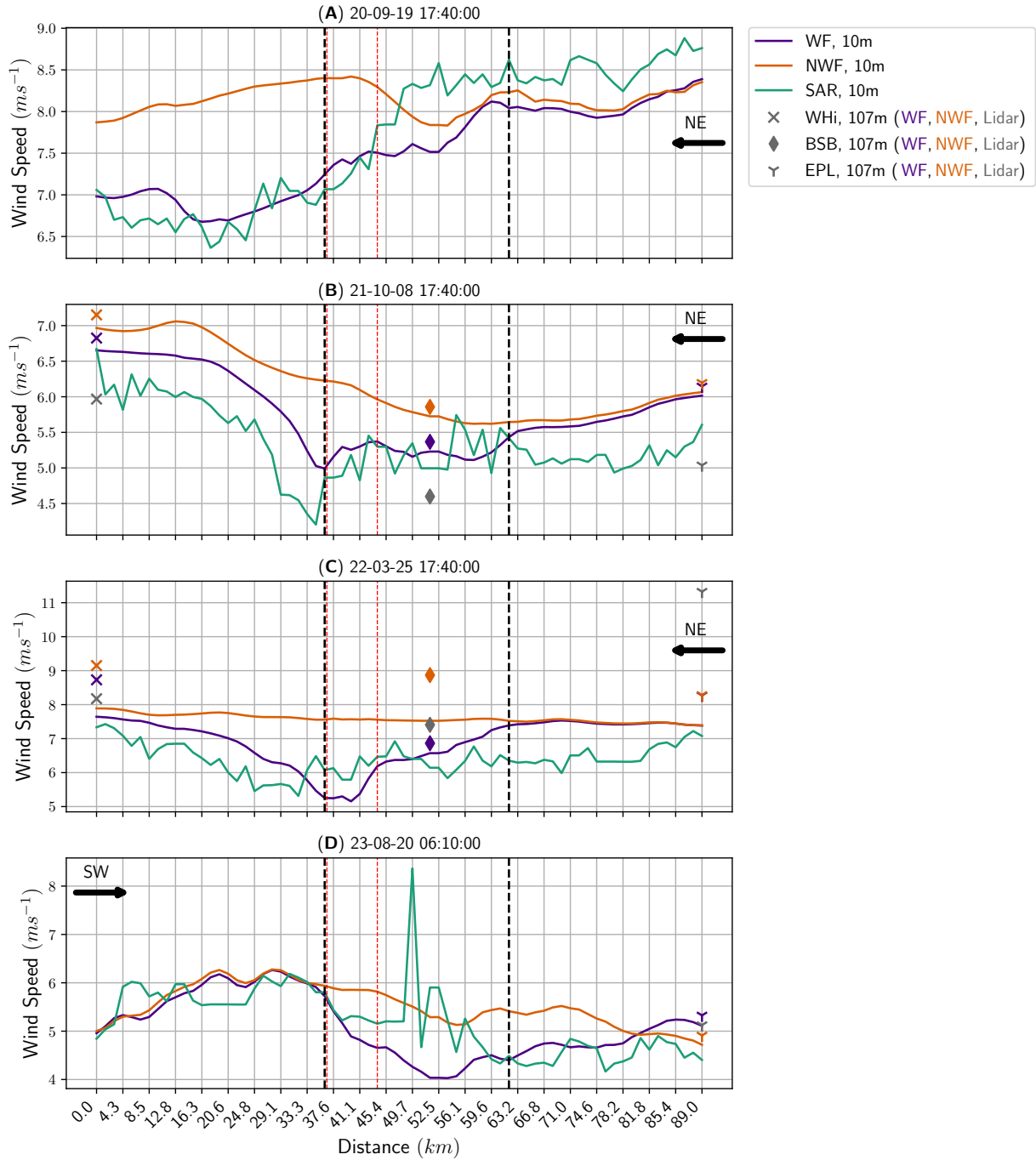
Figure 19. Wind speeds along the WHi, BSB, and EPL transects. Comparison between WF (purple), NWF (orange), and SAR (green) at 10-meter height, including lidar observations at 107-meter height (scatter points) along the transects where available. Similar to Figures 12 and 13, the vertical black and red dashed lines indicate the Belgian-Dutch cluster and the Belgian zone only, respectively.
