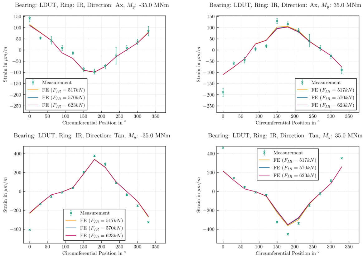
Figure 12: Axial and tangential strain of the lower bearing inner ring for bolt preload set 2 and M_y = \pm 35 MNm with constant coefficient of friction of 0.2
