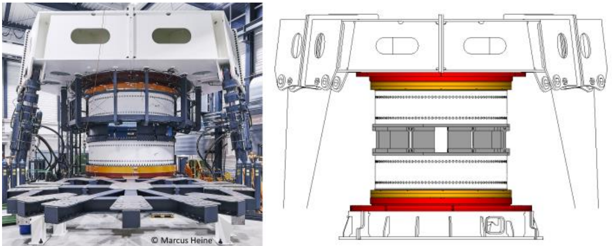
Figure 5: Fraunhofer IWES blade bearing test rig BEAT6.1 (left) and the FE test rig model (right)
