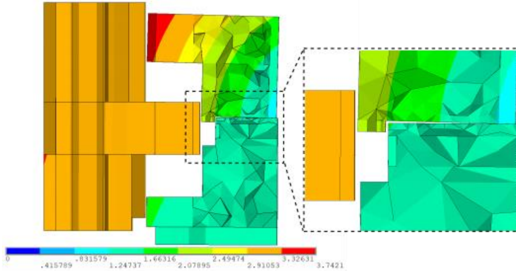
Figure 7: Gap opening of the outer ring split of the lower bearing
