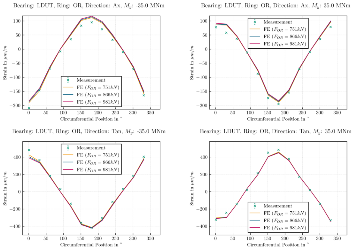
Figure 11: Axial and tangential strain of the lower bearing outer ring for bolt preload set 2 and M_y = \pm 35 MNm with constant coefficient of friction of 0.2
