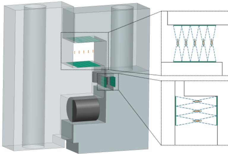
Figure 2: Modelling the rollers of a three-row roller bearing with nonlinear springs
