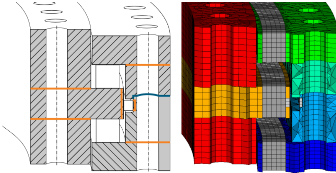
120 Figure 3: Defined contacts between the bearing ring sections (left) and resulting mesh of the bearing rings (right)
