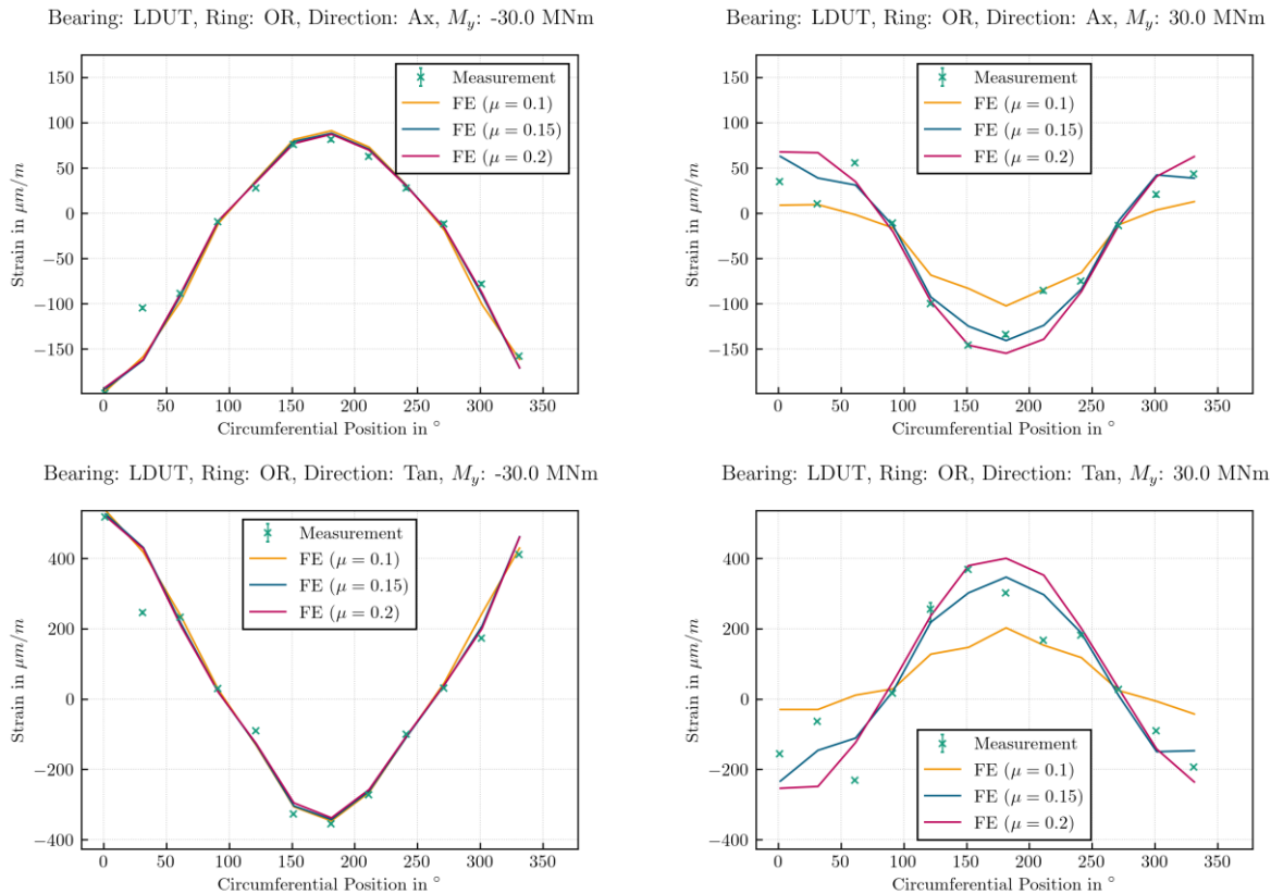
Figure 8: Axial and tangential strain of the lower bearing outer ring for bolt preload set 1 and M_y = \pm 30 MNm with constant bolt preloads of 330 kN
