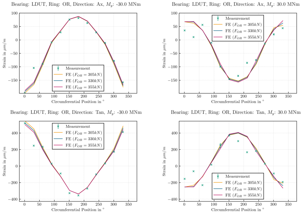
250 Figure 9: Axial and tangential strain of the lower bearing outer ring for bolt preload set 1 and M_y = \pm 30 MNm with constant coefficient of friction of 0.2
