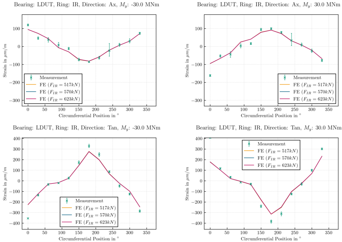
Figure 10: Axial and tangential strain of the lower bearing inner ring for bolt preload set 1 and M_y = \pm 30 MNm with constant coefficient of friction of 0.2
