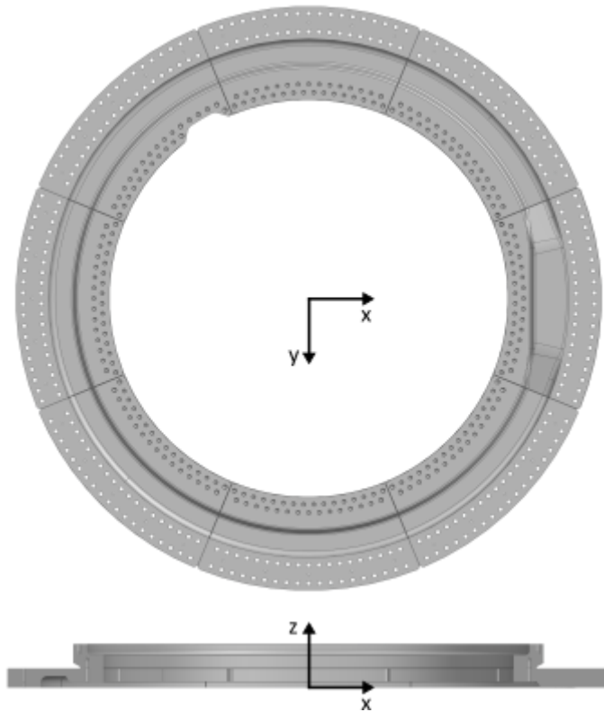
Figure 4: Bottom view and cross section of the lower hub adapter
