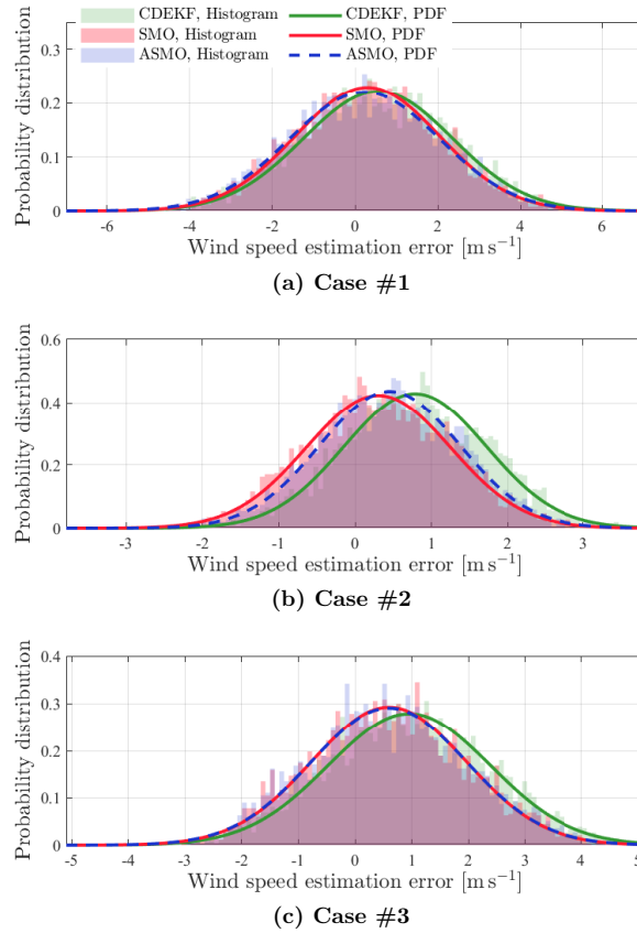
Figure 17. Comparison of the distribution and probability density function (PDF) of the REWS estimation error in three test cases.
