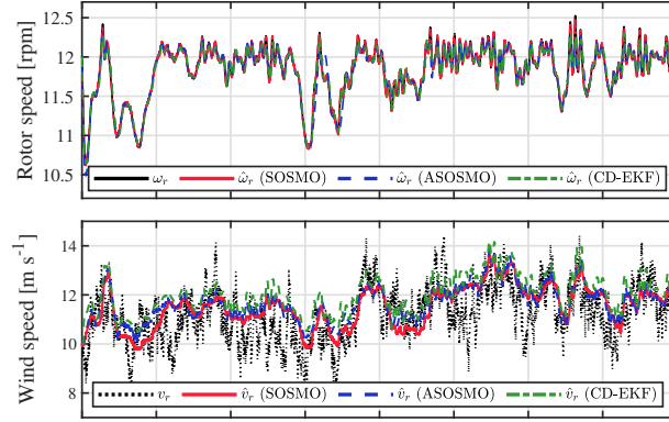
Figure 14. Experimental results for case 2: rotor speed \omega_r , REWS v_r , and their estimated values under turbulent wind and wave conditions.
